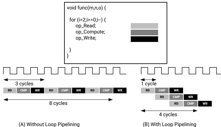
Figure 135: Loop Pipeline
