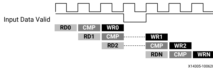
Figure 18: Loop Pipelining with Stall
