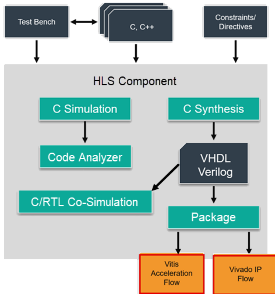
Figure 2: HLS Component Development Flow
