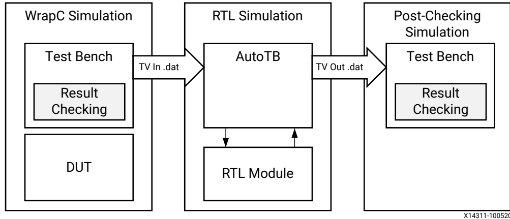
Figure 123: C/RTL Verification Flow
