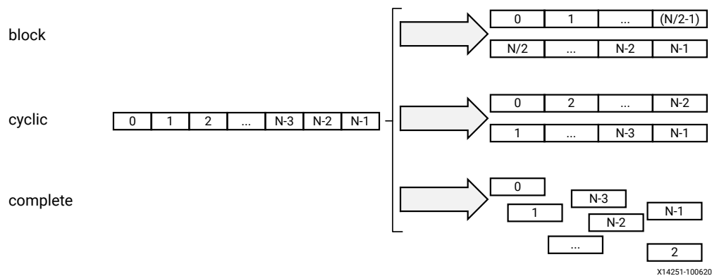
Figure 28: Array Partitioning
