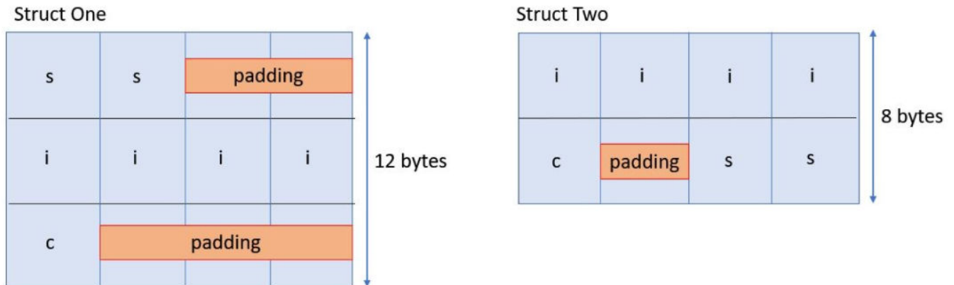
Figure 53: Padding of Structs
