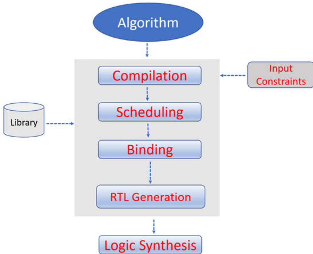
Figure 57: HLS Tasks
