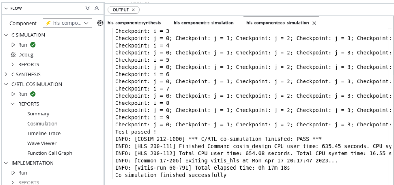
Figure 122: HLS Component Running C/RTL Co-Simulation
