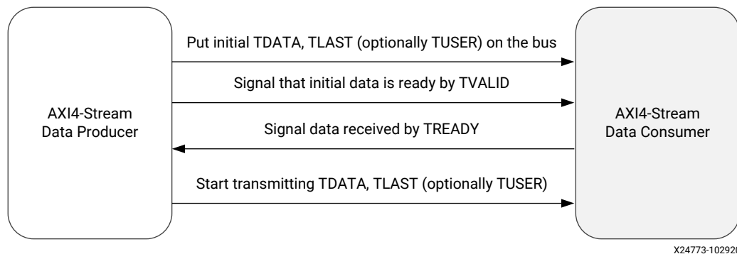
Figure 46: AXI4-Stream Handshake
