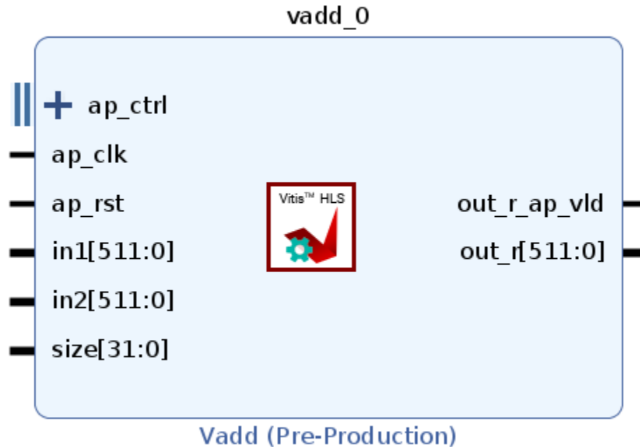
Figure 36: RTL Ports After Default Interface Synthesis
