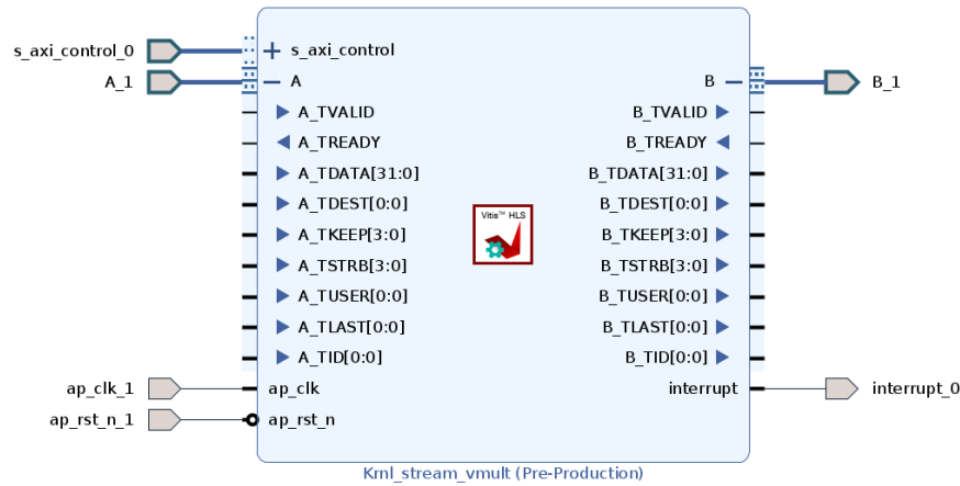
Figure 48: AXI4-Stream Interfaces with Side-Channels
