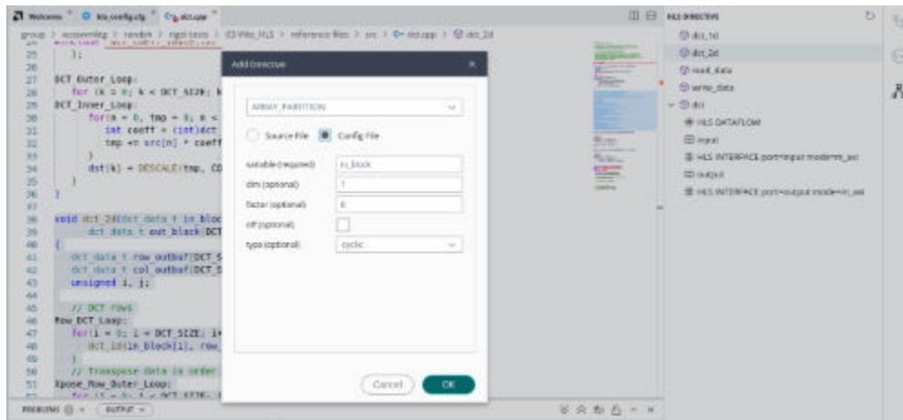
Figure 97: HLS Directive Editor
