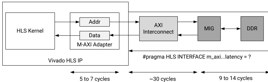
Figure 66: Burst Transaction Diagram
