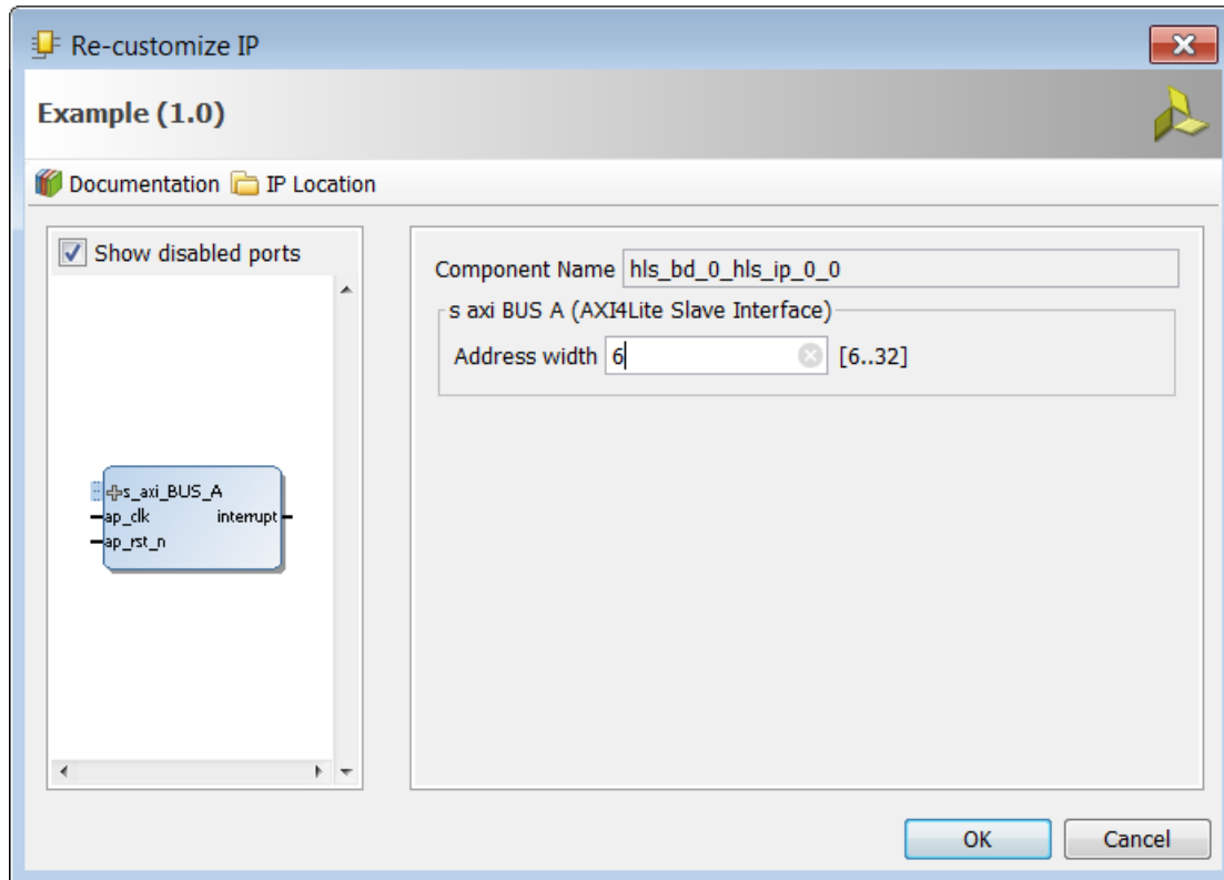
Figure 45: Customizing AXI4-Lite Slave Interfaces in IP Integrator
