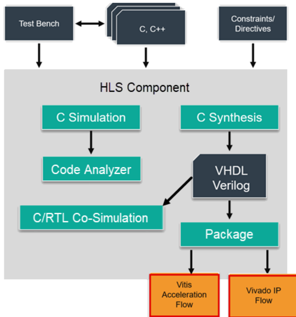
Figure 85: Vitis HLS Development Flow
