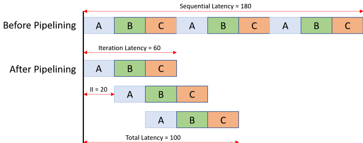
Figure 6: Pipelining
