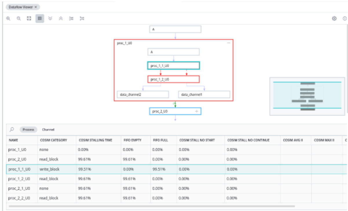
Figure 125: Deadlock Viewer
