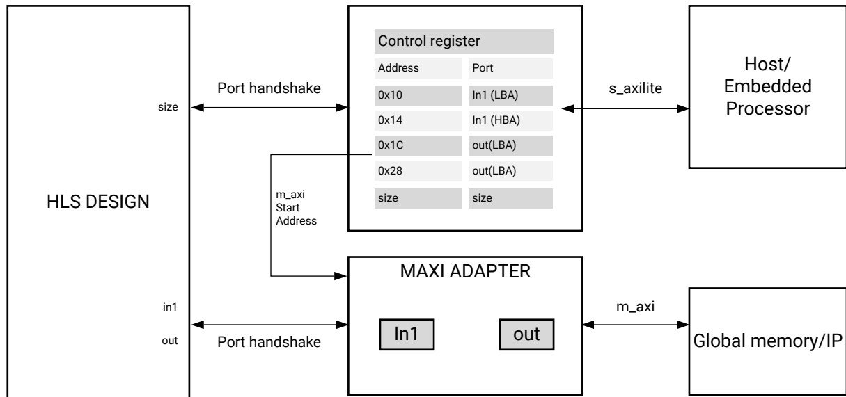
Figure 39: AXI Adapters in Slave Mode
