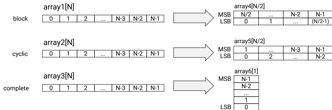
Figure 30: Array Reshaping
