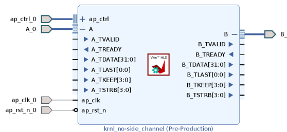
Figure 47: AXI4-Stream Interfaces without Side-Channels
