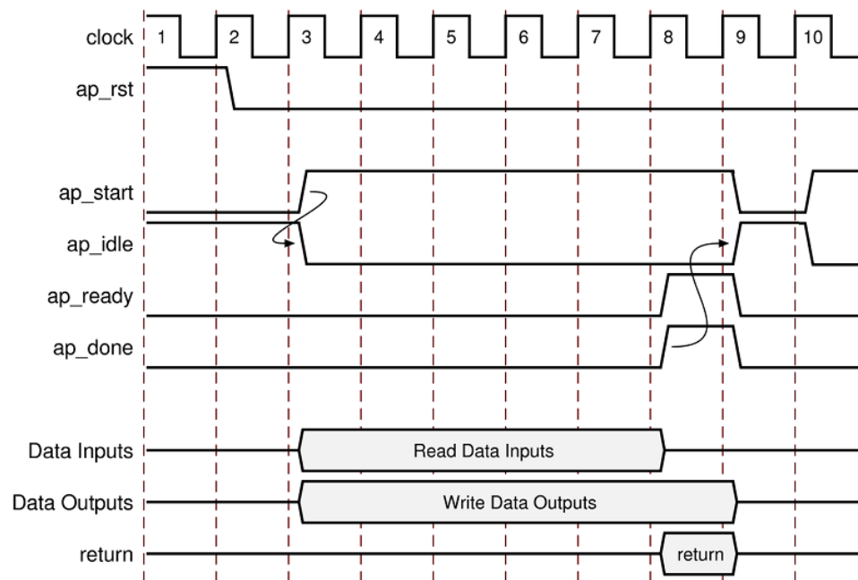
Figure 49: RTL Port Timing with Default Synthesis
