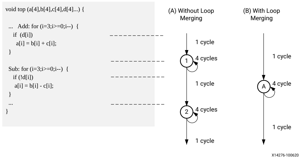
Figure 24: Loop Directives
