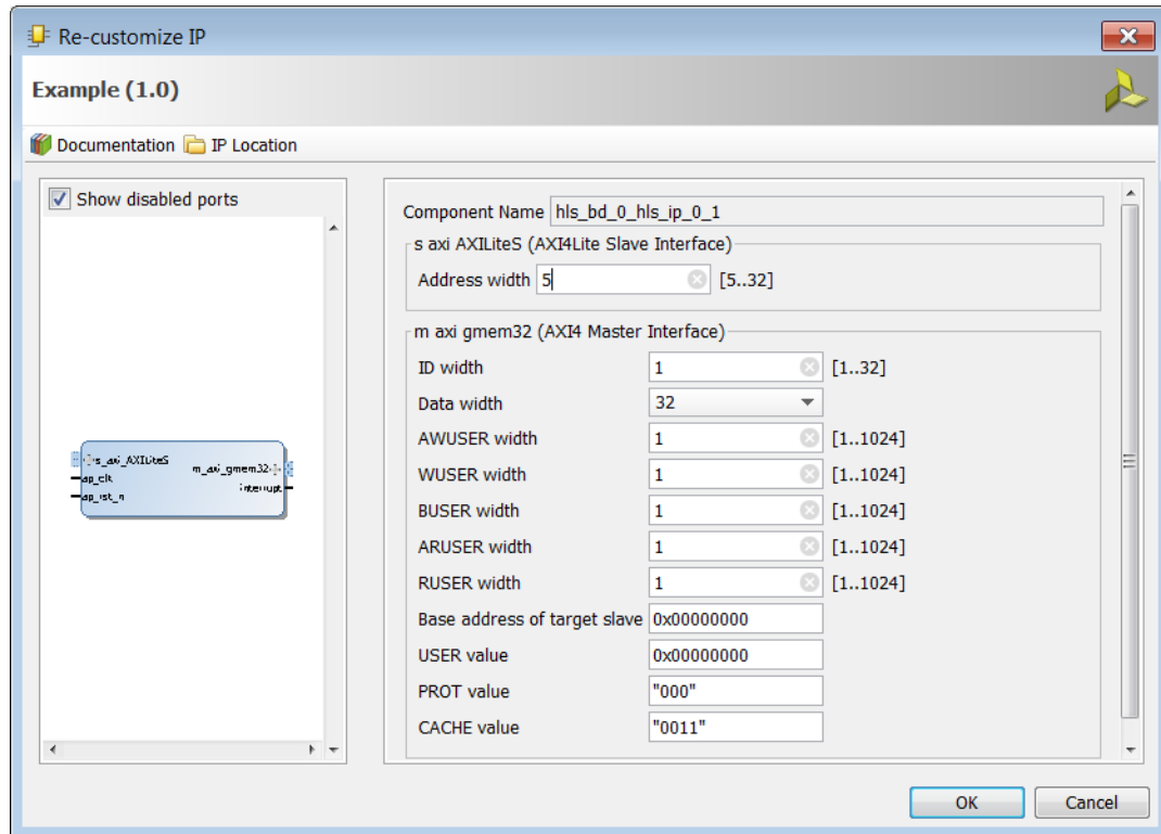
Figure 43: Customizing AXI4 Master Interfaces in IP Integrator
