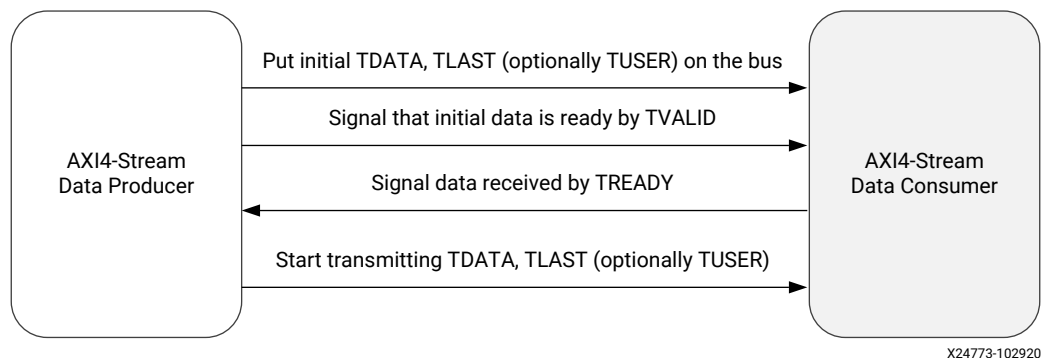
Figure 35: AXI4-Stream Handshake
