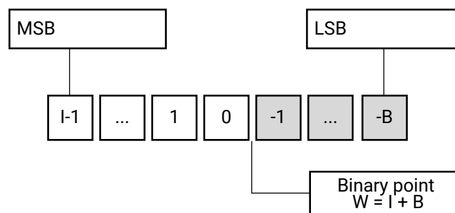
Figure 136: Fixed-Point Data Type
