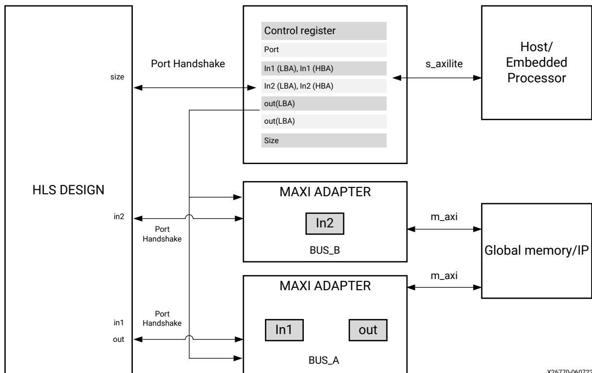
Figure 41: 2 MAXI Bundles
