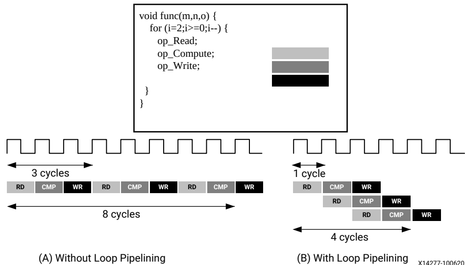
Figure 16: Loop Pipelining
