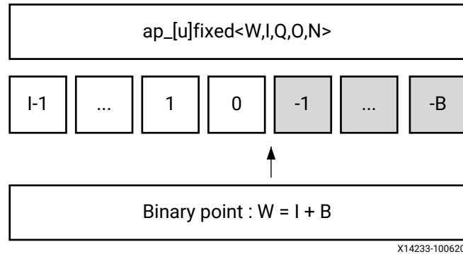
Figure 137: Arbitrary Precision Fixed-Point Types
