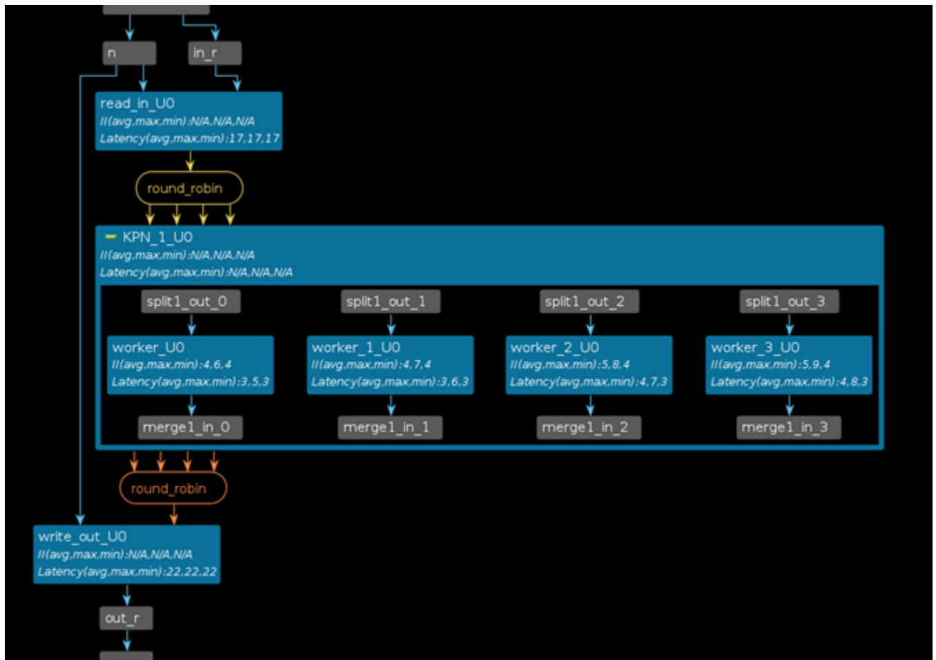
Figure 15: Mixed Task-Channel and Dataflow
