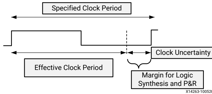
Figure 96: Clock Period and Margin
