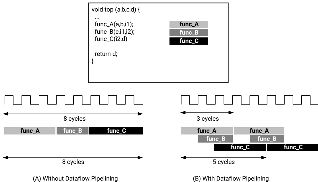
Figure 134: DATAFLOW Pragma
