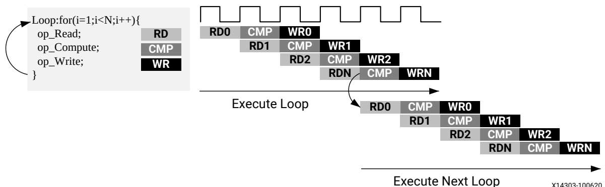
Figure 17: Loop Pipelining with Rewind Option
