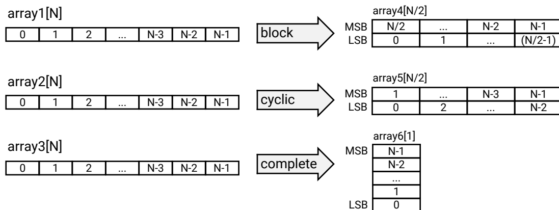
Figure 133: ARRAY_RESHAPE Pragma
