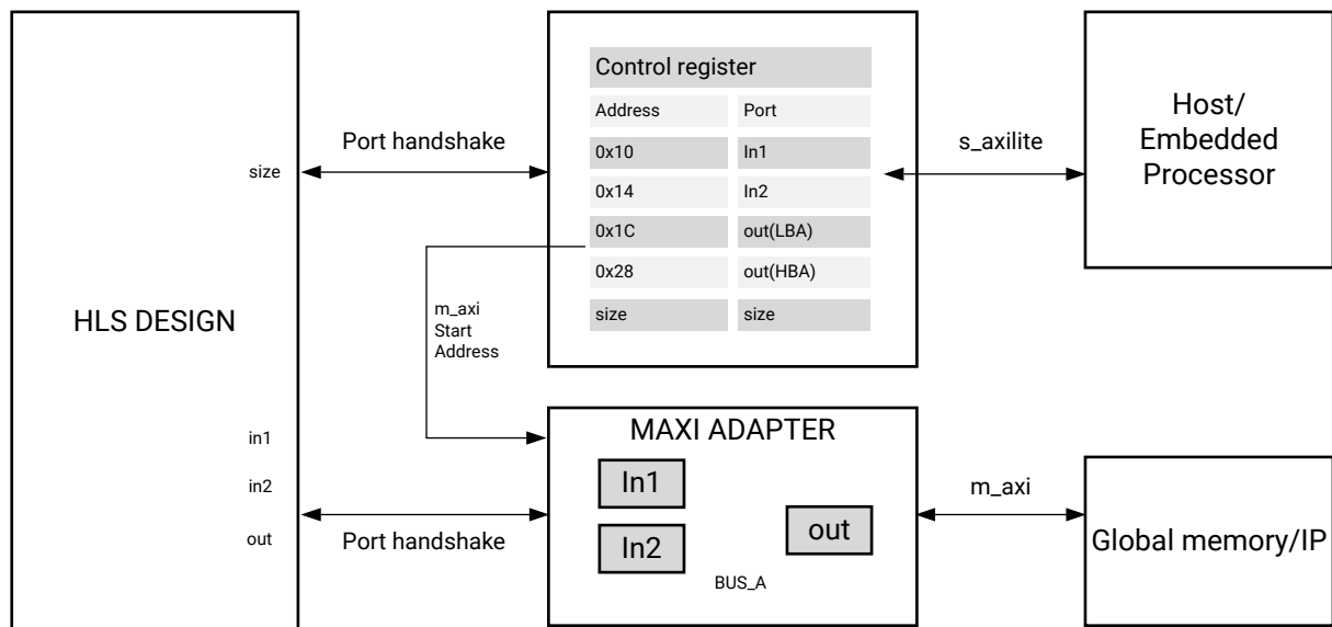
Figure 40: MAXI and S_AXILITE
