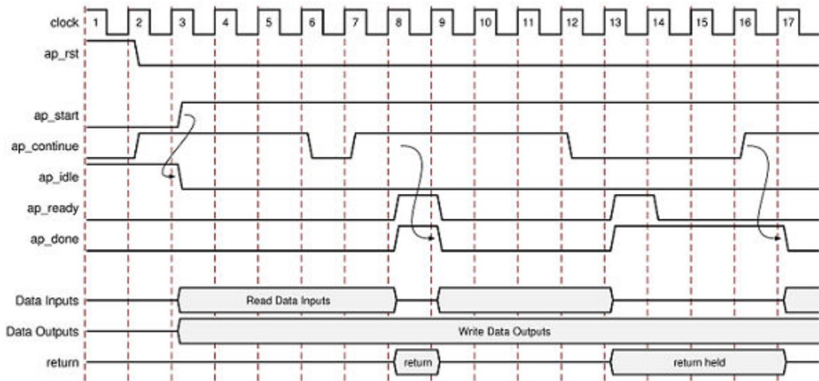
Figure 55: Behavior of ap_ctrl_chain Interface
