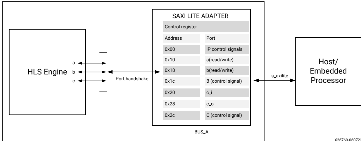
Figure 44: S_AXILITE Adapter
