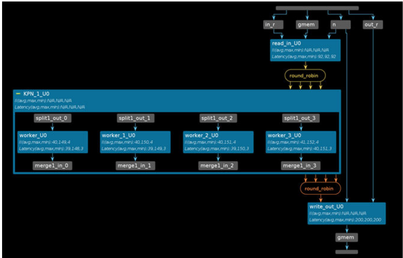
Figure 139: Split/Merge Dataflow
