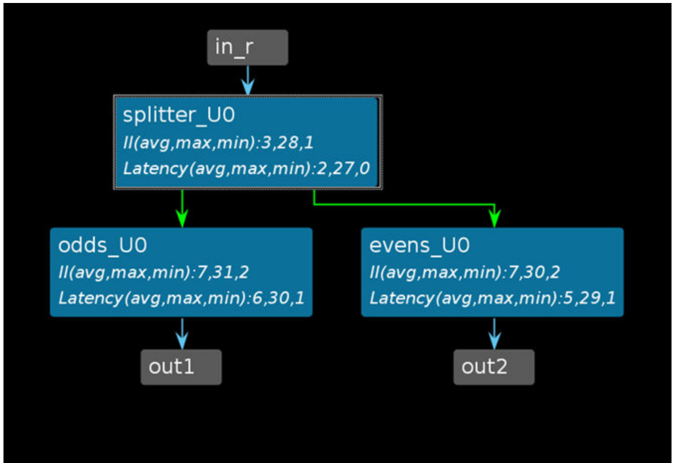
Figure 12: Dataflow Diagram of hls::task Example
