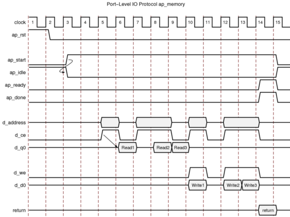
Figure 51: Behavior of ap_memory Interface
