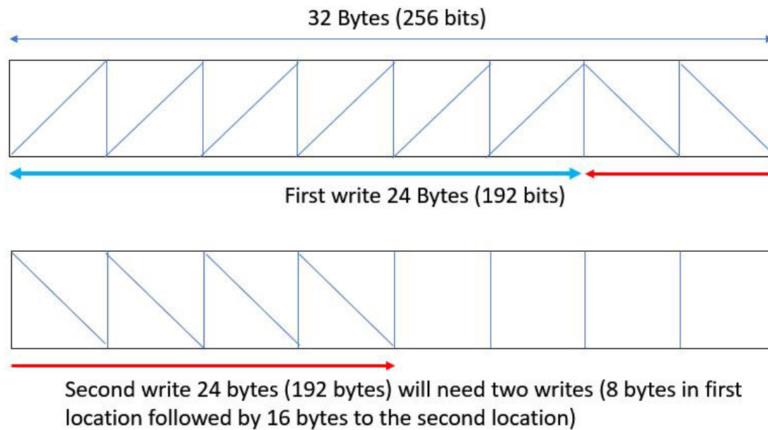
Figure 54: Misaligned Write Cycles
