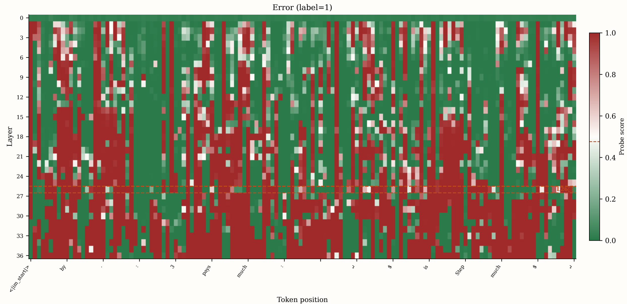
Layer \times token probe heatmap — 2hop_arithmetic_0000
