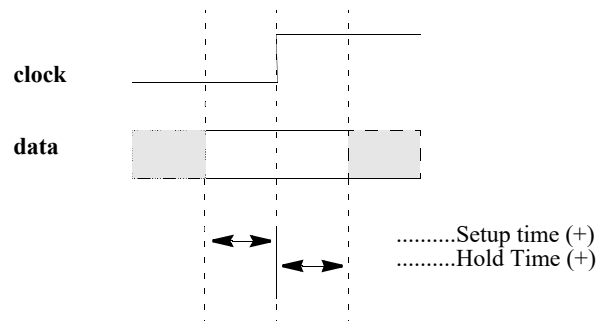
Figure 31-4—Data constraint interval, positive setup/hold
