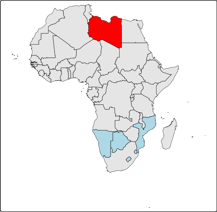
Local Moran's I (LISA) Cluster Map
