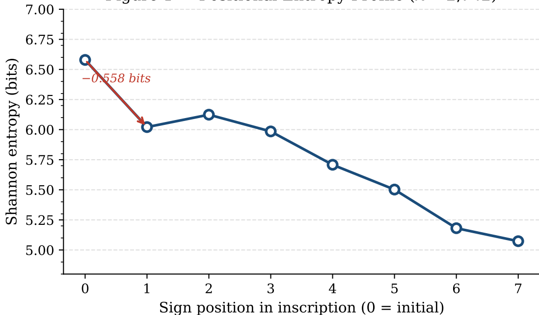
Figure 1 — Positional Entropy Profile ( N = 2,742 )
