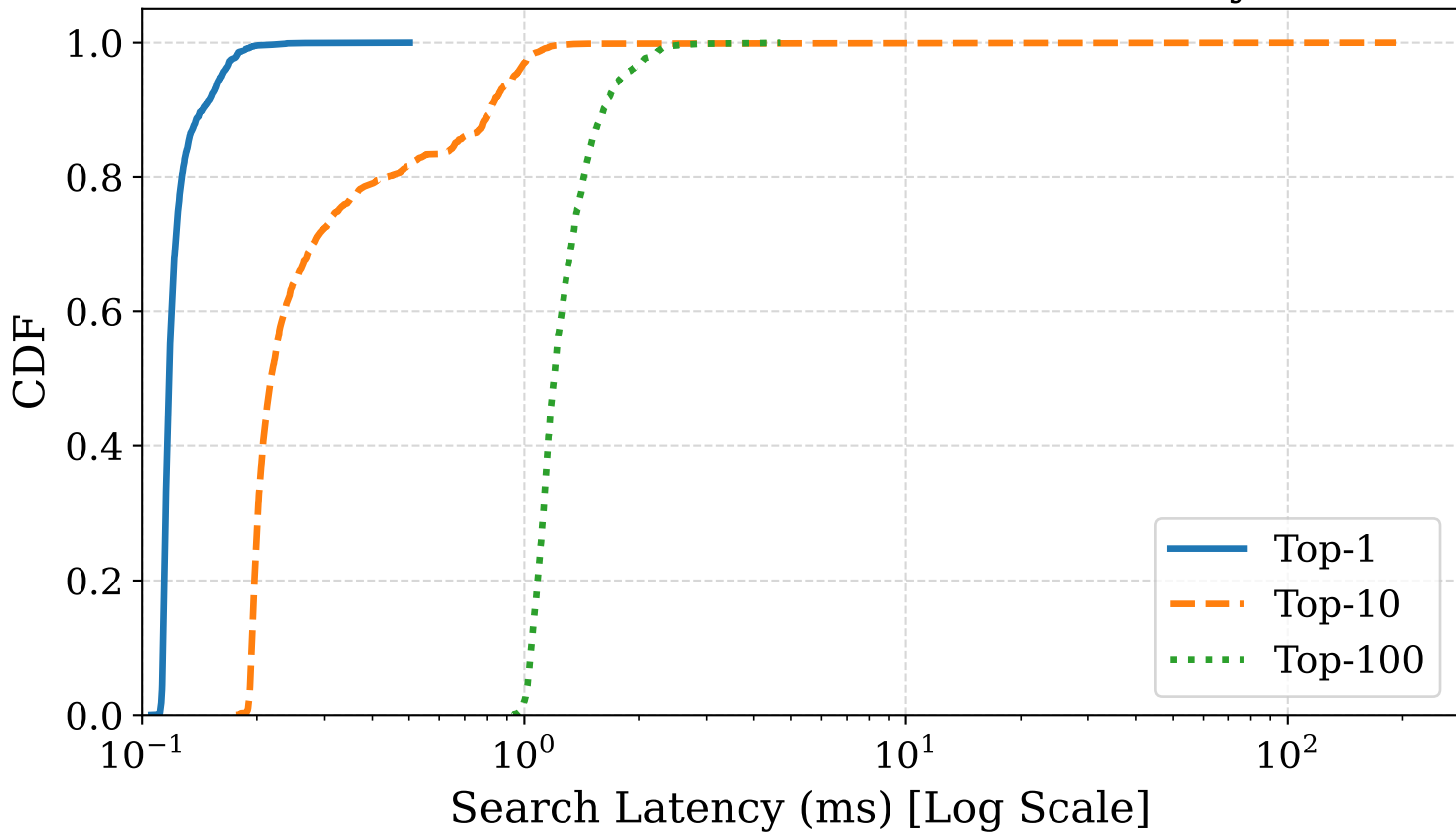
CDF of HNSW Vector Search Latency
