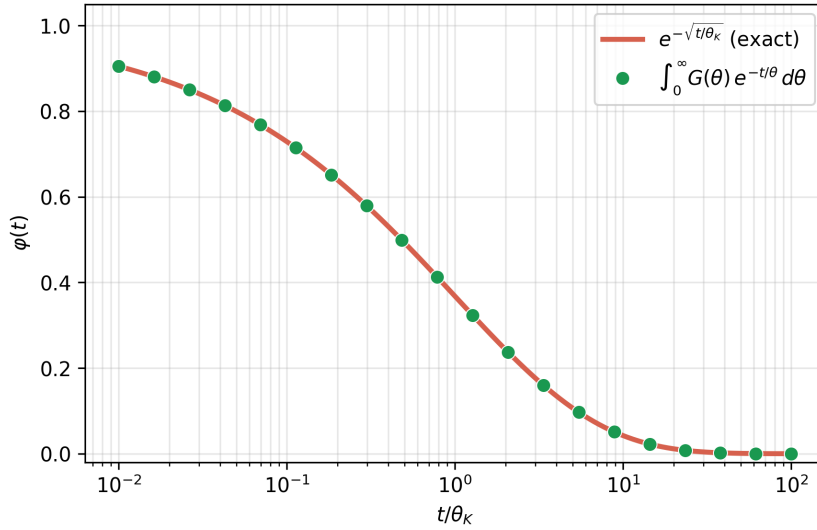
Figure 1: Verification of the Pollard identity for n = 1/2 : \varphi(t) = e^{-(t/\theta_K)^{1/2}} .
