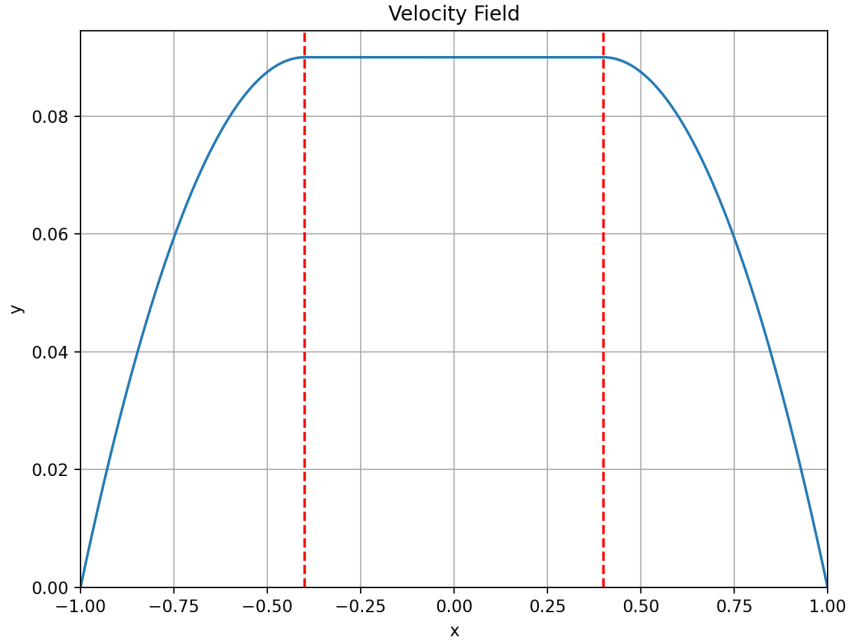
Figure 2: Velocity field for a Bingham fluid flowing through a tube.
