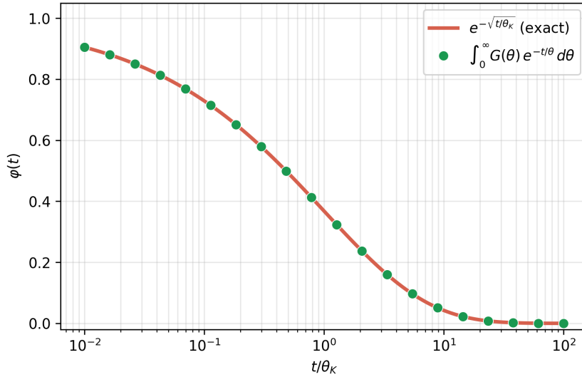
Figure 1: The relaxation function \varphi(t) = e^{-\sqrt{t/\theta_K}} (solid line) replicated by the numerical integration of equation 1.2.
