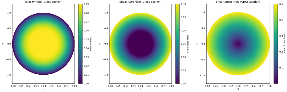
Figure 3: Cross-sectional profiles of velocity, shear rate, and shear stress for a Bingham fluid flowing through a tube. The region near the center of the tube (where r < r_0 ) has zero shear rate. The velocity profile is flat in this region and then decreases towards the walls of the tube. The shear stress increases linearly from r = 0 to r = R .
