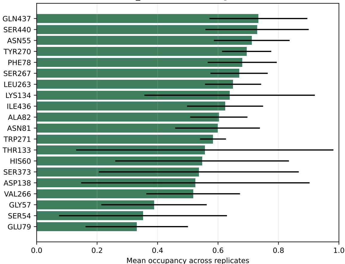
SGLT2 Mol_13144 consensus ligand contacts
