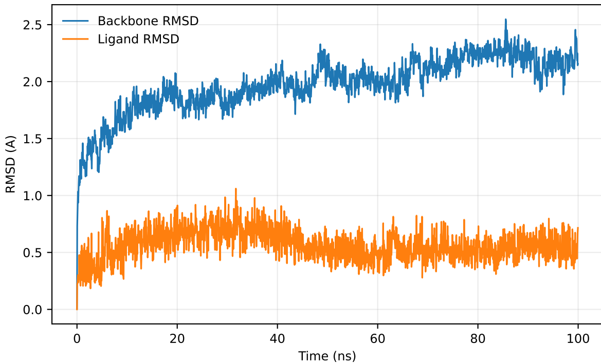
SGLT2 Mol_13144 rep3 RMSD
