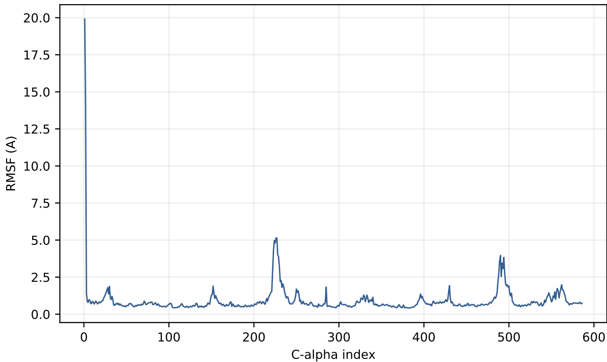
SGLT2 Mol_13144 rep3 C-alpha RMSF
