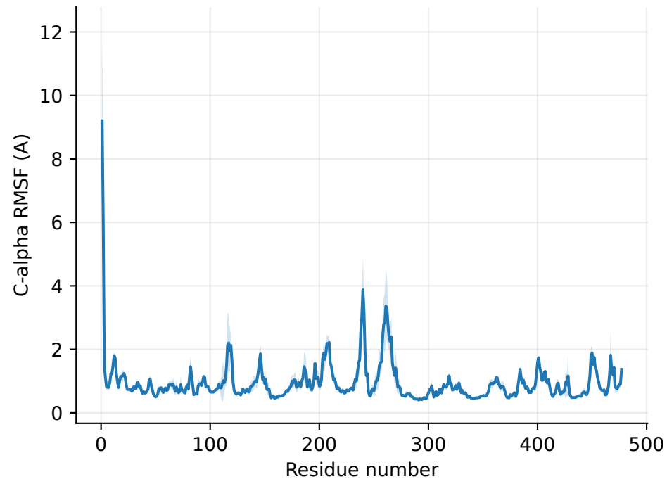
Per-residue C-alpha RMSF, mean \pm SD across replicates
