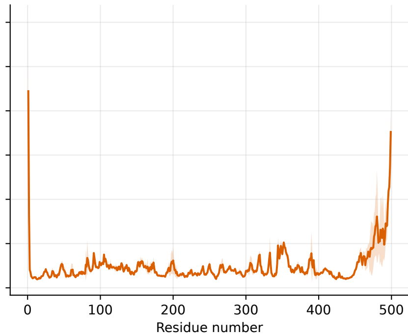
Per-residue C-alpha RMSF, mean \pm SD across replicates
