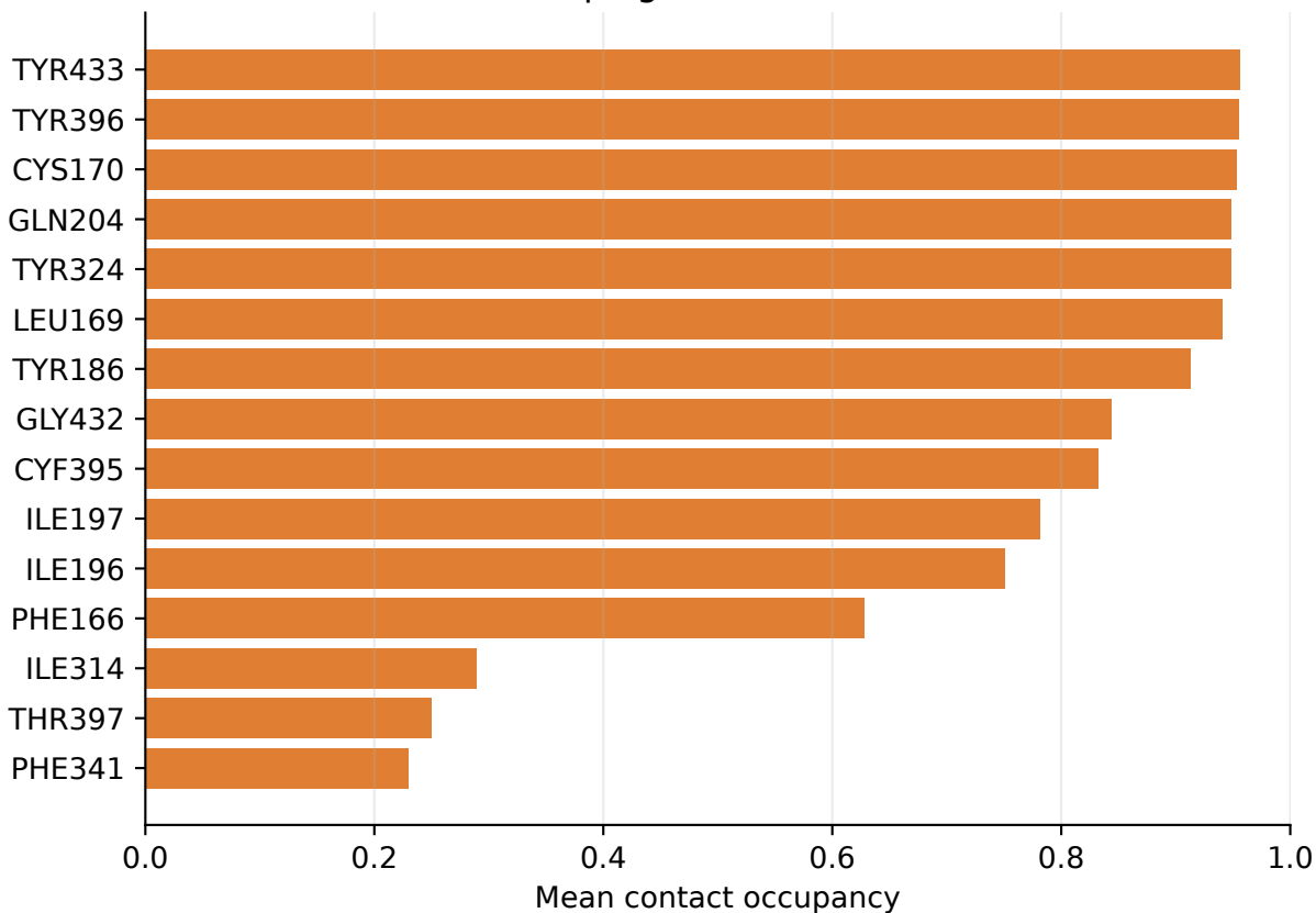
MAO-B: top ligand-contact residues
