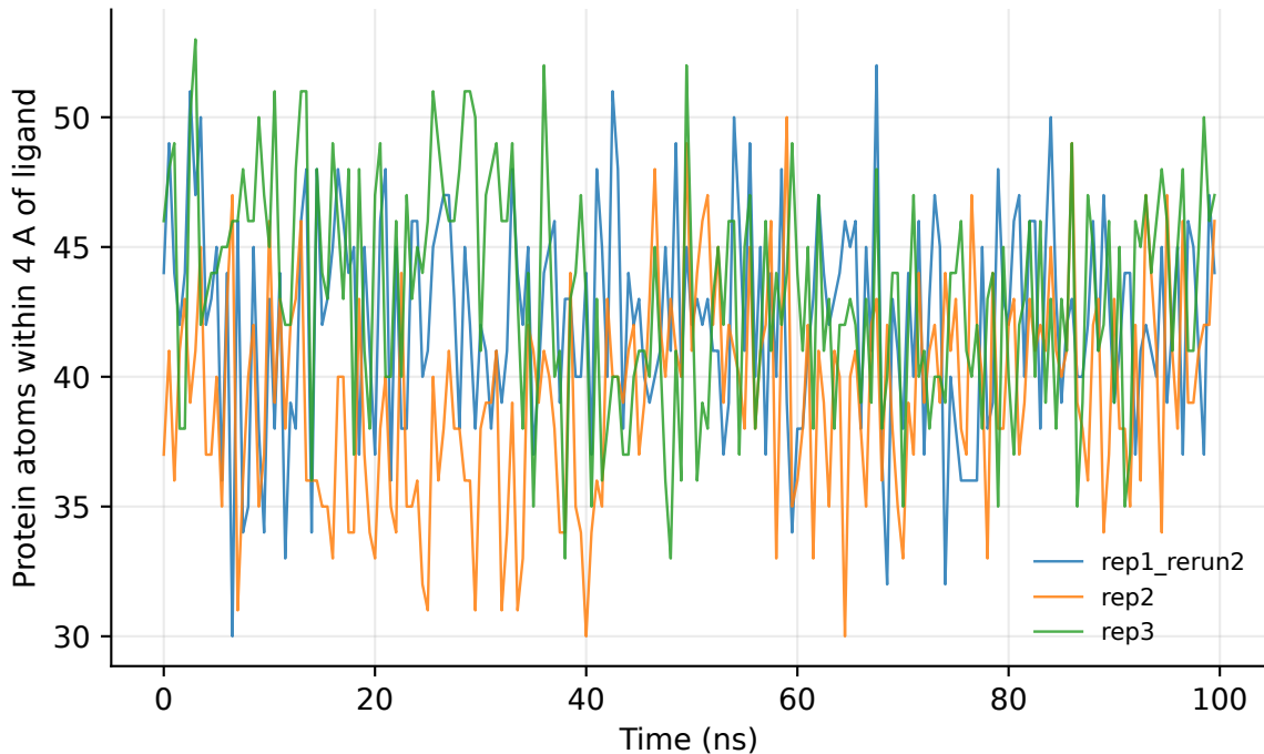
MAO-B PBC-corrected Protein atoms within 4 Å of ligand
