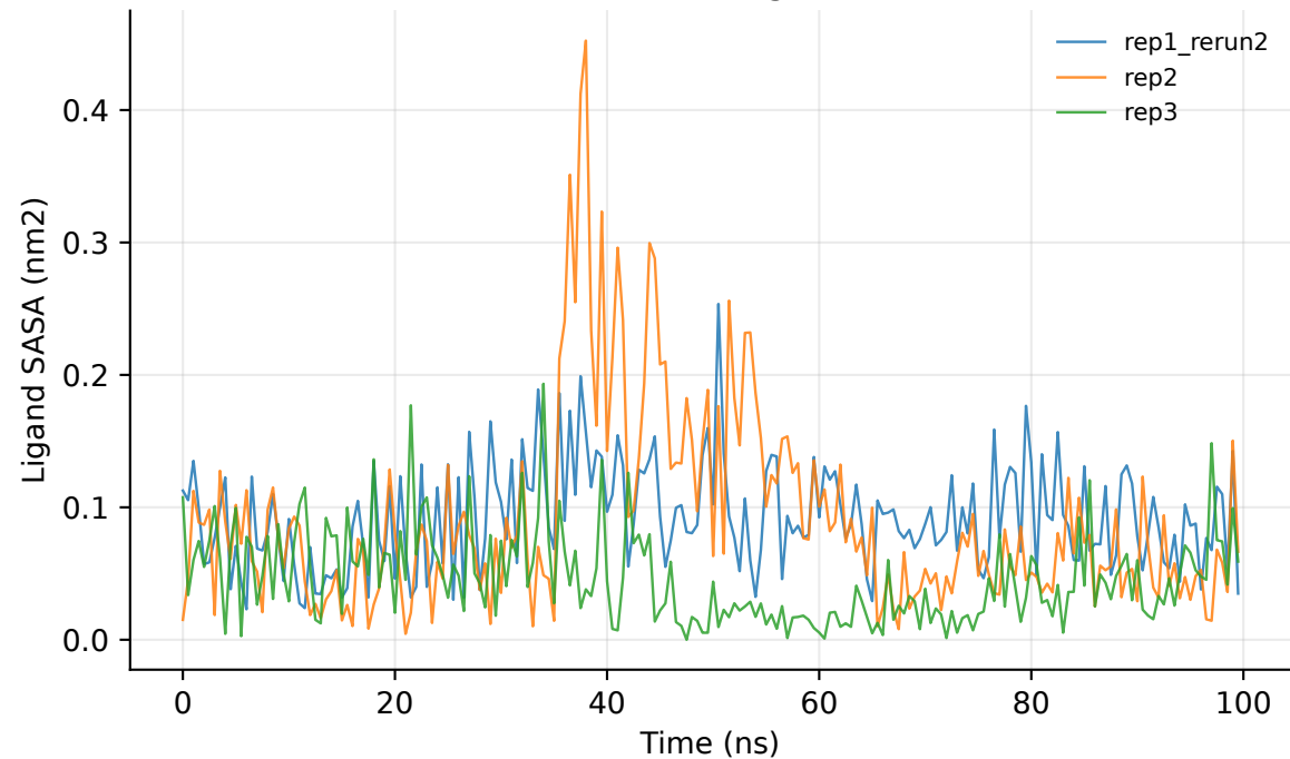
MAO-B PBC-corrected Ligand SASA (nm 2 )
