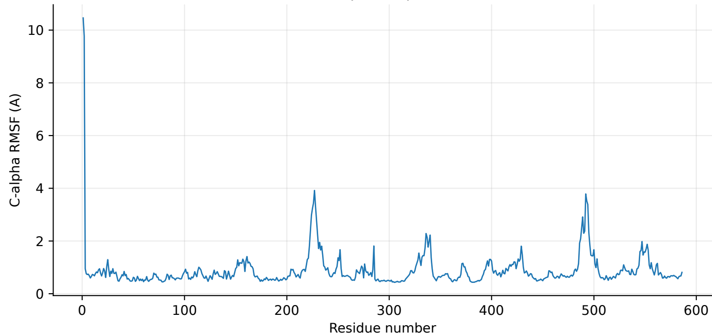
SGLT2 rep1 C-alpha RMSF
