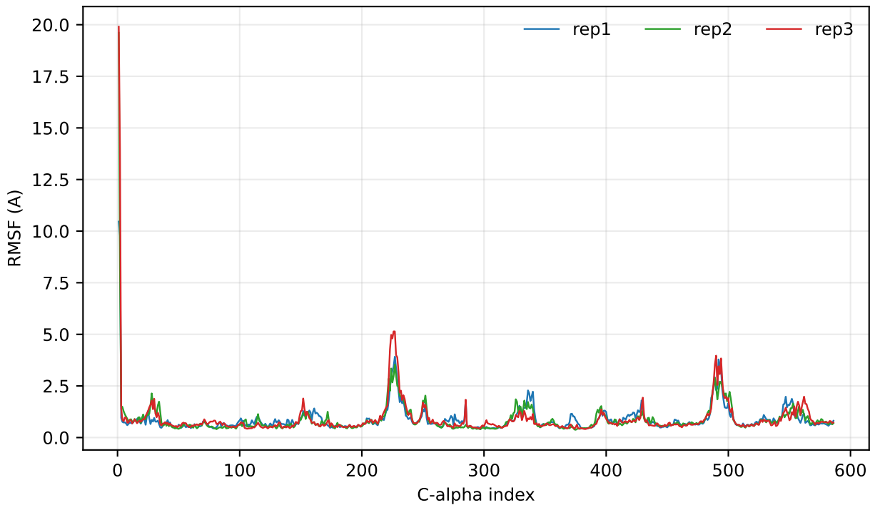
SGLT2 Mol_13144 C-alpha RMSF across replicates
