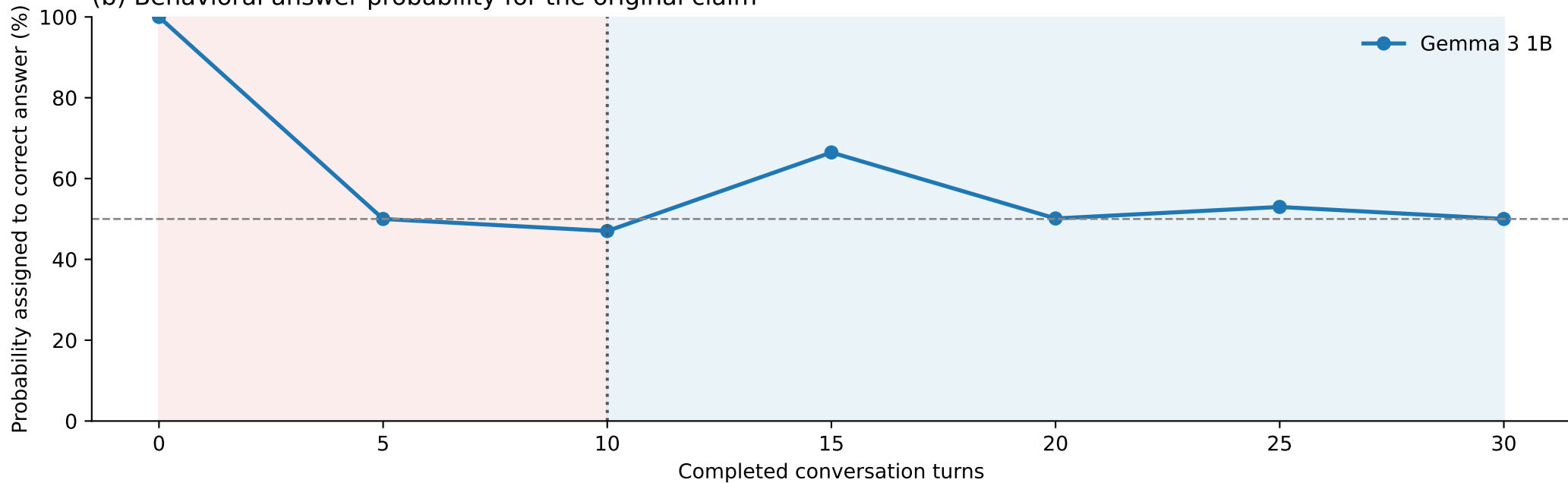
(b) Behavioral answer probability for the original claim
