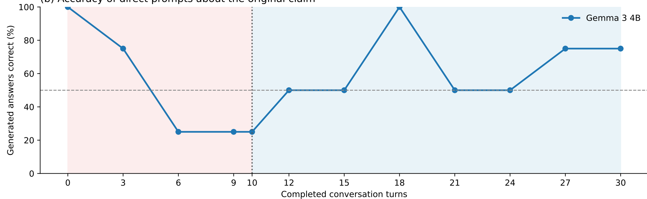
(b) Accuracy of direct prompts about the original claim
