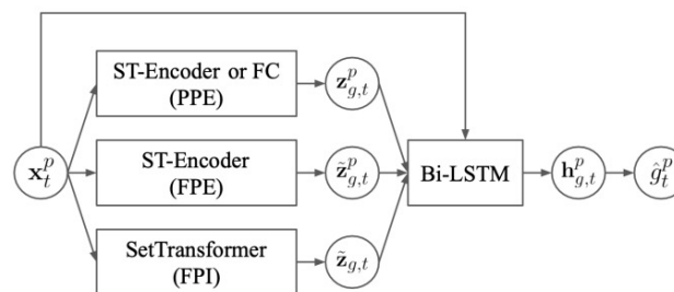
(a) Player Possession Classifier.
