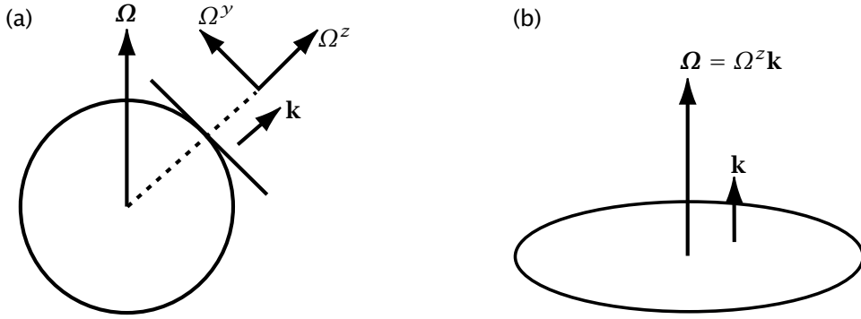
Fig. 2.4 (a) On the sphere the rotation vector \mathbf{\Omega} can be decomposed into two components, one in the local vertical and one in the local horizontal, pointing toward the pole. That is, \mathbf{\Omega} = \Omega_y \mathbf{j} + \Omega_z \mathbf{k} where \Omega_y = \Omega \cos \vartheta and \Omega_z = \Omega \sin \vartheta . In geophysical fluid dynamics, the rotation vector in the local vertical is often the more important component in the horizontal momentum equations. On a rotating disk, (b), the rotation vector \mathbf{\Omega} is parallel to the local vertical \mathbf{k} .
