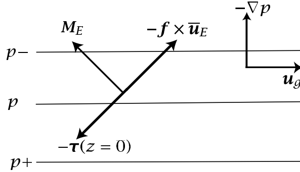
Fig. 2.11 A bottom Ekman layer, generated from an eastward geostrophic flow above it. An overbar denotes a vertical integral over the Ekman layer, so that -\bar{f} \times \bar{\mathbf{u}}_E is the Coriolis force on the vertically integrated Ekman velocity. \mathbf{M}_E is the frictionally induced boundary layer transport, and \boldsymbol{\tau} is the stress.
