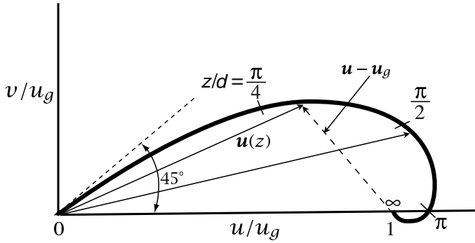
Fig. 2.9 The idealized Ekman layer solution in the lower atmosphere, plotted as a hodograph of the wind components: the arrows show the velocity vectors at particular heights, and the curve traces out the continuous variation of the velocity. The values on the curve are of the non-dimensional variable z/d , where d = (2A/f)^{1/2} , and v_g is chosen to be zero.
