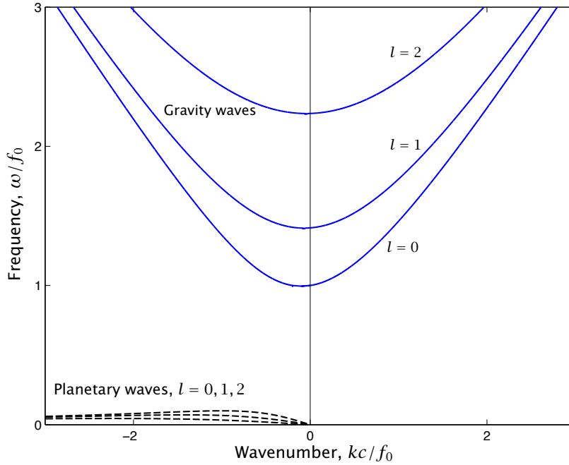
Fig. 6.12 Dispersion relation for Rossby-gravity waves, obtained from (3.129) with \hat{\beta} = 0.2 for three values of l . There is a frequency gap between the Rossby or planetary waves and the gravity waves. For the stratified mid-latitude atmosphere or ocean the frequency gap is in fact much larger.
