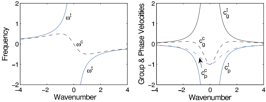
Fig. 6.7 Left: the dispersion relation for barotropic ( \omega^t , solid line) and baroclinic ( \omega^c , dashed line) Rossby waves in the two-layer model, calculated using (3.71) and (3.72) with k^y = 0 , plotted for both positive and negative zonal wavenumbers and frequencies. The wavenumber is non-dimensionalized by k_d , and the frequency is non-dimensionalized by \beta/k_d . Right: the corresponding zonal group and phase velocities, c_g = \partial\omega/\partial k^x and c_p = \omega/k^x , with superscript 't' or 'c' for the barotropic or baroclinic mode, respectively. The velocities are non-dimensionalized by \beta/k_d^2 .
