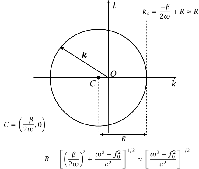
Fig. 6.11 Wave propagation diagrams for Rossby-gravity waves, obtained using (3.116). The top figure shows the diagram in the low frequency, Rossby wave limit, and the bottom figure shows the high frequency, gravity wave limit. In each case the locus of wavenumbers for a given frequency is a circle centered at C = (-\beta/2\omega, 0) with a radius R given by (3.117), but the approximate expressions differ significantly at high and low frequency.
