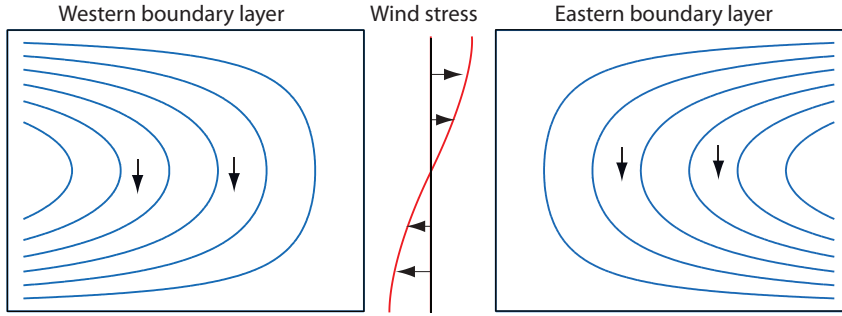
Figure 5.5 Two possible Sverdrup flows, \psi_T , for the wind stress shown in the centre. Each solution satisfies the no-flow condition at either the eastern or western boundary, and a boundary layer is therefore required at the other boundary. Both flows have the same, equatorward, meridional flow in the interior. Only the flow with the western boundary current is physically realizable, however, because only then can friction produce a curl that opposes that of the wind stress, so allowing the flow to equilibrate.
