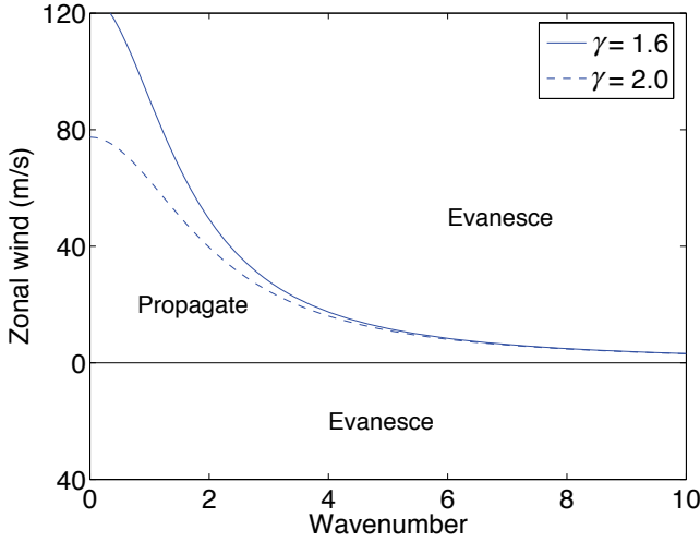
Figure 4.4 The boundary between propagating waves and evanescent waves as a function of zonal wind and wavenumber, using (4.58), for a couple of values of \gamma . With N = 2 \times 10^{-2} \text{ s}^{-1} , \gamma = 1.6 ( \gamma = 2 ) corresponds to a scale height of 7.0 km (5.5 km) and a deformation radius NH/f of 1400 km (1100 km).
