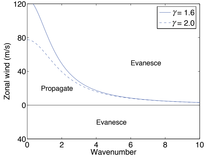
Figure 4.4 The boundary between propagating waves and evanescent waves as a function of zonal wind and wavenumber, using (4.58), for a couple of values of \gamma . With N = 2 \times 10^{-2} \text{ s}^{-1} , \gamma = 1.6 ( \gamma = 2 ) corresponds to a scale height of 7.0 km (5.5 km) and a deformation radius NH/f of 1400 km (1100 km).
