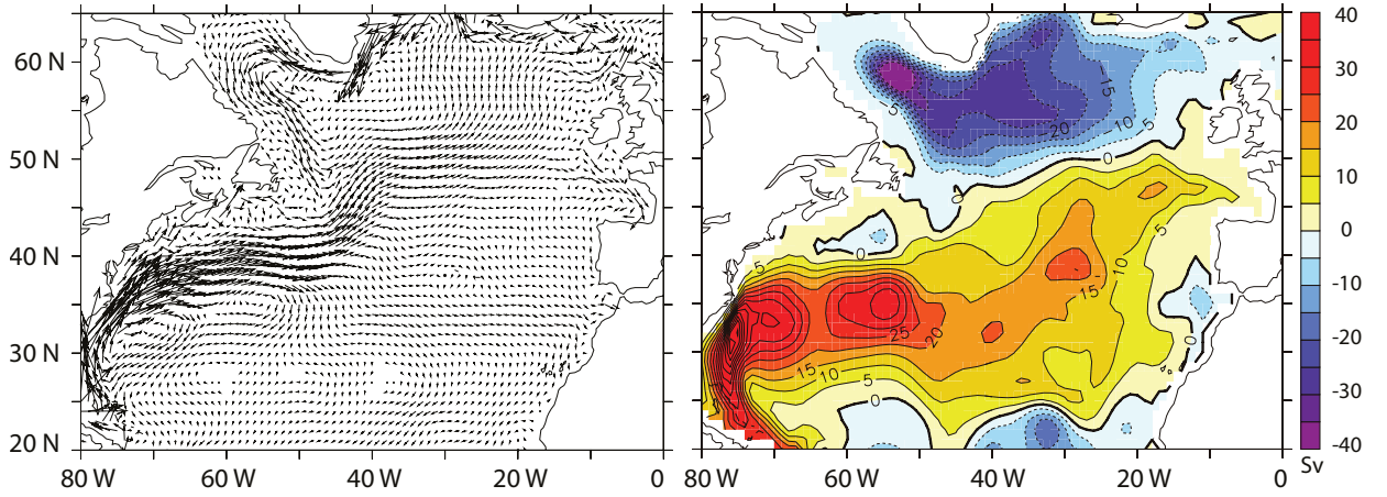
Figure 5.3 Left: the time averaged velocity field at a depth of 75 m in the North Atlantic. Right: the streamfunction of the vertically integrated flow, in Sverdrups ( 1 \text{ Sv} = 10^9 \text{ kg s}^{-1} ). Note the presence of an anticyclonic subtropical gyre (clockwise circulation, shaded red), a cyclonic subpolar gyre (anticlockwise, blue), and intense western boundary currents.
