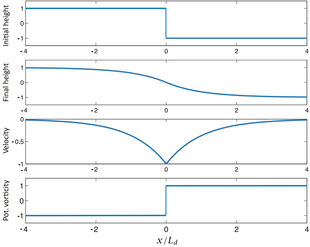
Figure 2.8 Solutions of a linear geostrophic adjustment problem. Top panel: the initial height field, given by (2.90) with \eta_0 = 1 . Second panel: equilibrium (final) height field, \eta given by (2.103) and \eta = f_0 \psi / g . Third panel: equilibrium geostrophic velocity (normal to the gradient of height field), given by (2.104). Bottom panel: potential vorticity, given by (2.99), and this does not evolve. The distance, x is non-dimensionalized by the deformation radius L_d = \sqrt{gH}/f_0 , and the velocity by \eta_0(g/f_0 L_d) . Changes to the initial state occur only within \mathcal{O}(L_d) of the initial discontinuity; and as x \rightarrow \pm\infty the initial state is unaltered.
