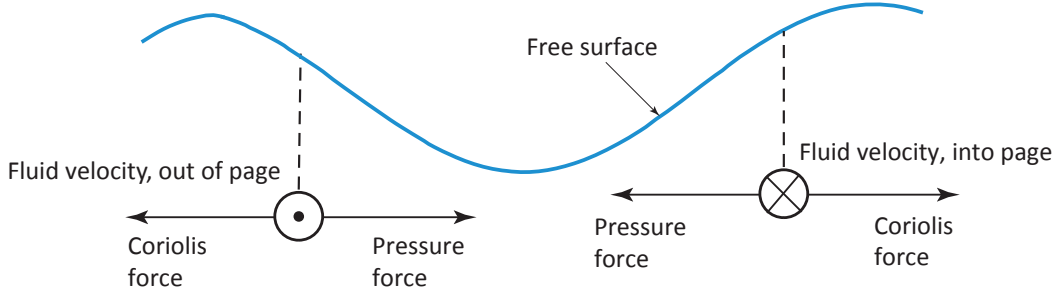
Figure 2.4 Geostrophic flow in a shallow water system, with a positive value of the Coriolis parameter f , as in the Northern Hemisphere. The pressure force is directed down the gradient of the height field, and this can be balanced by the Coriolis force if the fluid velocity is at right angles to it. If f were negative, the geostrophic flow would be reversed.
