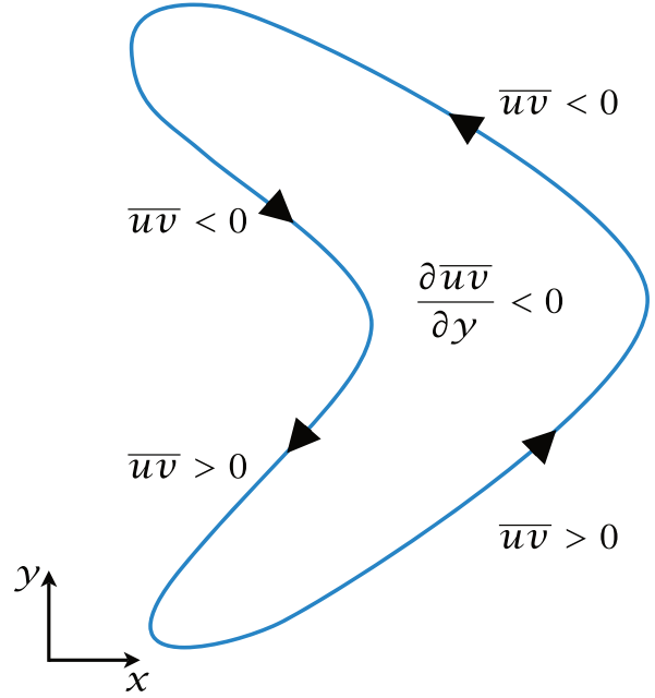
Figure 4.8 The momentum transport in physical space, caused by the propagation of Rossby waves away from a source in mid-latitudes. The ensuing bow-shaped eddies are responsible for a convergence of momentum, as indicated in the idealization pictured.
