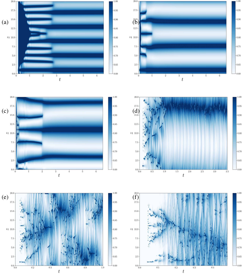
Figure 7: Hövmoller plots for relative humidity at z = 0.5 for M = 0.19 at (a) Ra = 2 \times 10^5 , (b) Ra = 1 \times 10^6 , (c) Ra = 2 \times 10^6 , (d) Ra = 2 \times 10^7 , (e) Ra = 5 \times 10^7 , (f) Ra = 2.5 \times 10^8 .
