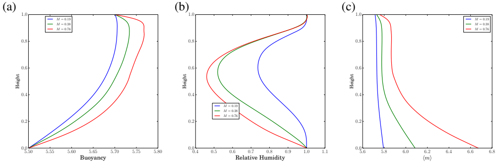
Figure 18: Horizontally averaged profiles for (a) buoyancy, (b) relative humidity and (c) m(z) for Ra = 2 \times 10^6 and a range of M . Note the different horizontal scale for \langle m \rangle from those of earlier figures showing \langle m \rangle .
