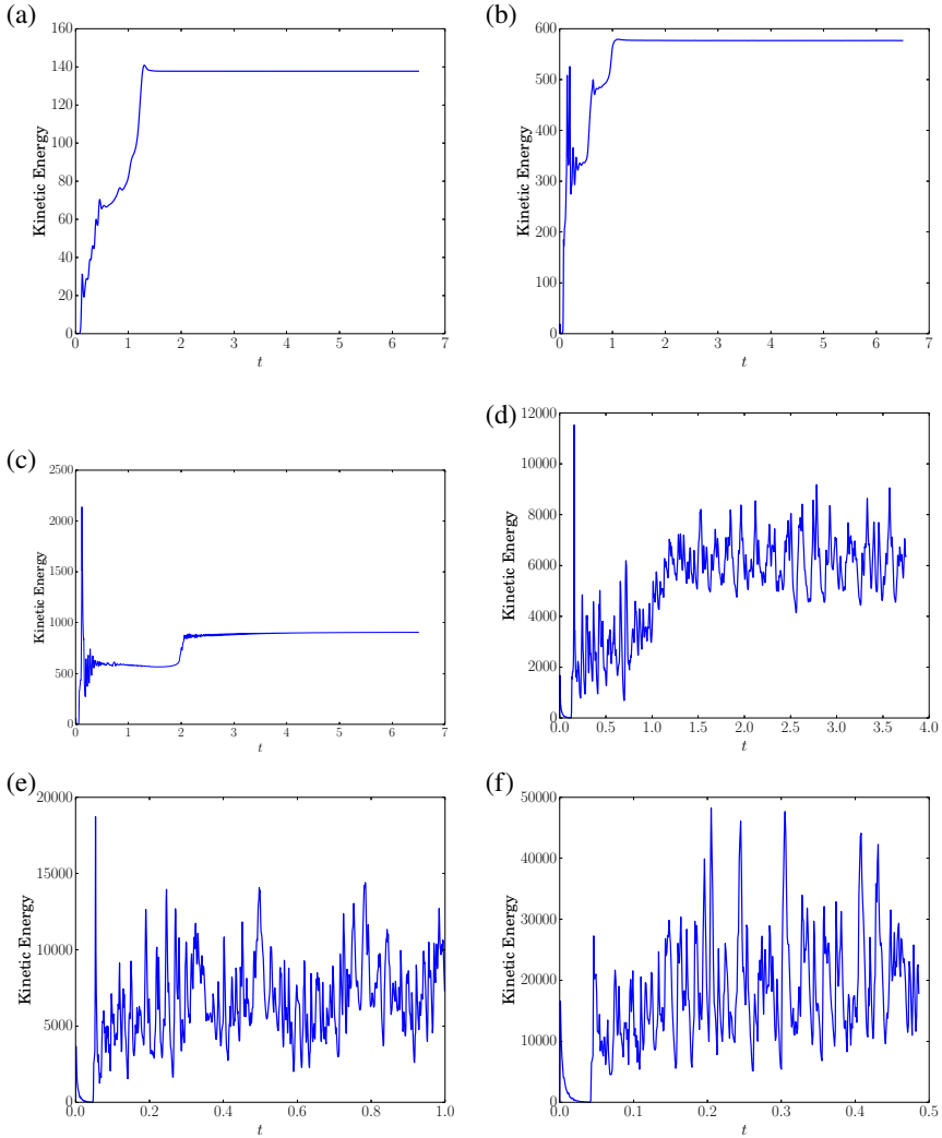
Figure 5: Timeseries for nondimensional kinetic energy for numerical simulations with M = 0.19 and (a) Ra = 2 \times 10^5 , (b) Ra = 1 \times 10^6 , (c) Ra = 2 \times 10^6 , (d) Ra = 2 \times 10^7 , (e) Ra = 5 \times 10^5 , (f) Ra = 2.5 \times 10^7 . The horizontal axis is time in diffusive units of H^2/\kappa , and note the differing scales of the axes in the panels.
