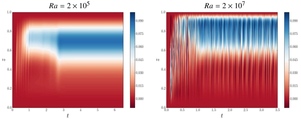
Figure 13: Time series (Hövmüller plots) of the x -averaged buoyancy fluxes, \langle w'b' \rangle , at two values of Rayleigh number. The time-averaged fields, over the later parts of the time period, are shown in Fig. 12.
