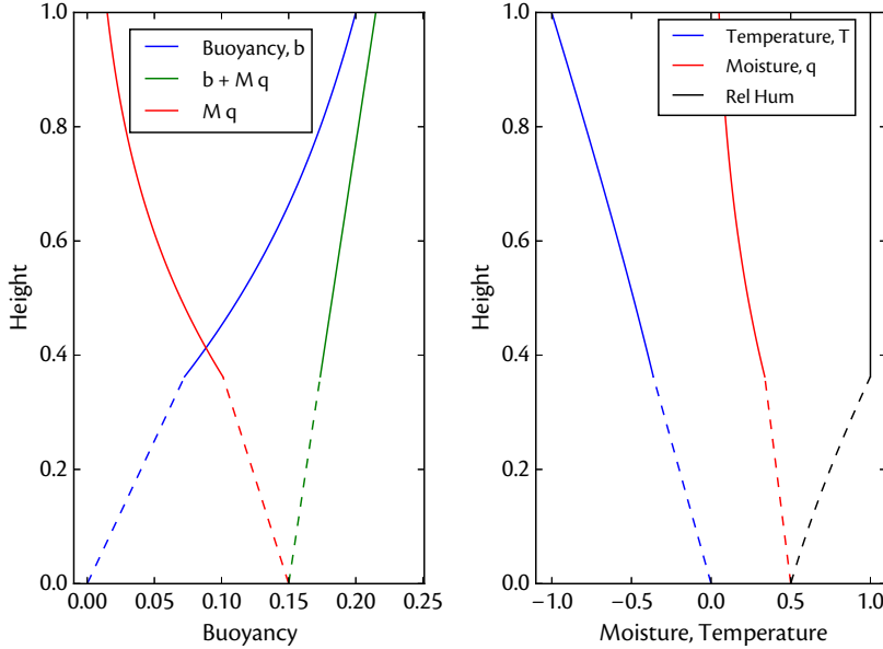
Figure 2: Drizzle solution with an unsaturated lower boundary, with relative humidity of 0.5. Other parameters are the same as in Fig. 1. The dashed lines show the linear profiles of moisture and buoyancy up to a height of about 0.38, above which the solution is saturated.
