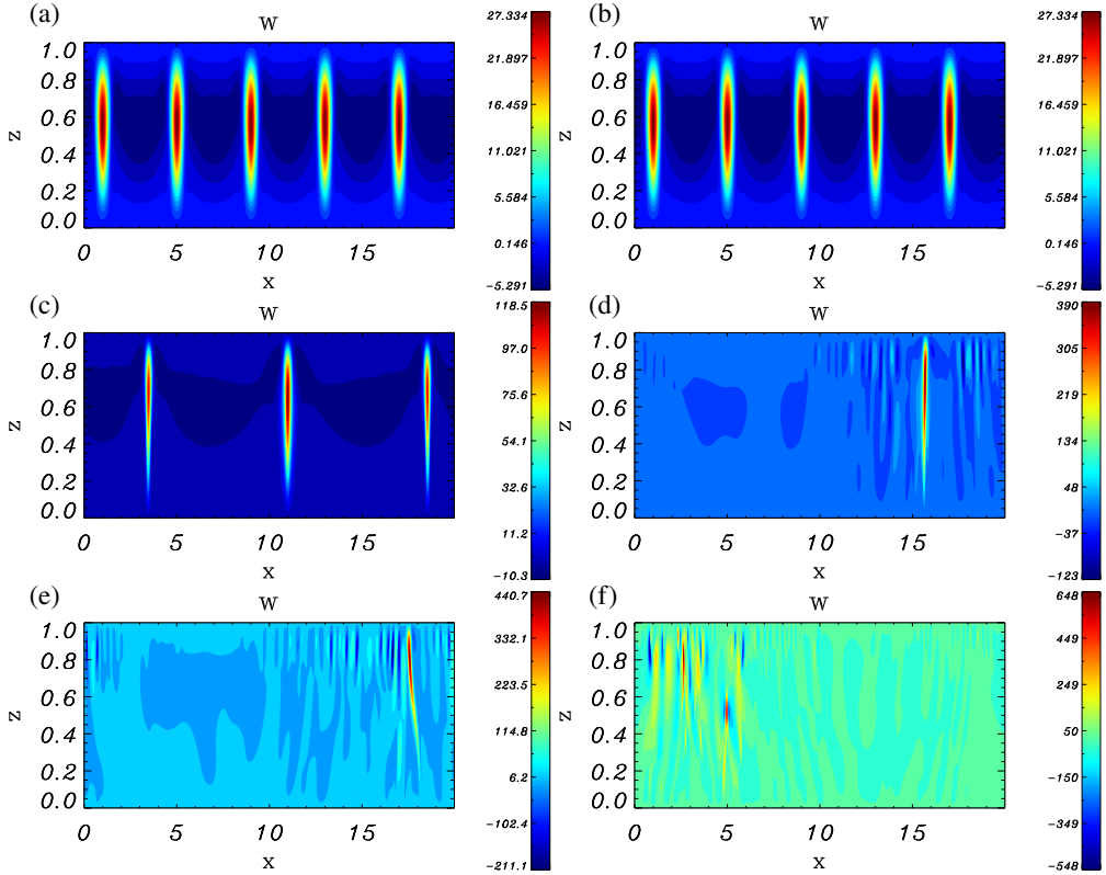
Figure 8: Snapshots of vertical velocity in a statistically equilibrated state for M = 0.19 at (a) Ra = 2 \times 10^5 , (b) Ra = 1 \times 10^6 , (c) Ra = 2 \times 10^6 , (d) Ra = 2 \times 10^7 , (e) Ra = 5 \times 10^7 , (f) Ra = 2.5 \times 10^8 .
