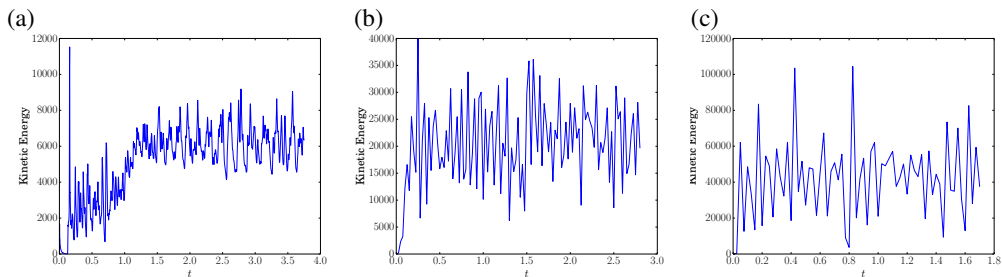
Figure 17: Timeseries for kinetic energy at Ra=2 \times 10^6 for: (a) M = 0.19 , (b) M = 0.38 and (c) M = 0.76 . Note the different scales on the vertical axes.
