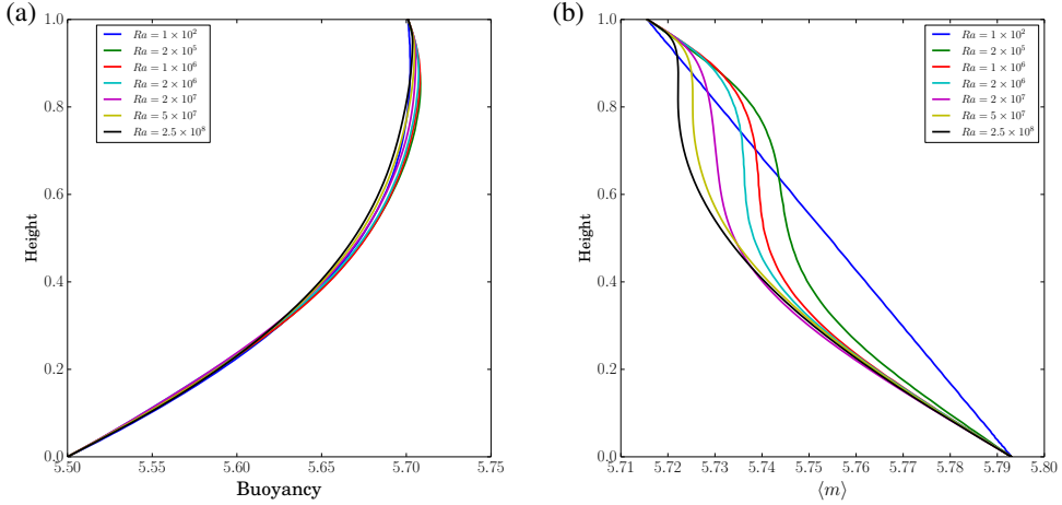
Figure 10: Horizontally averaged profiles for (a) buoyancy and (b) m(z) for M = 0.19 and a range of Ra .
