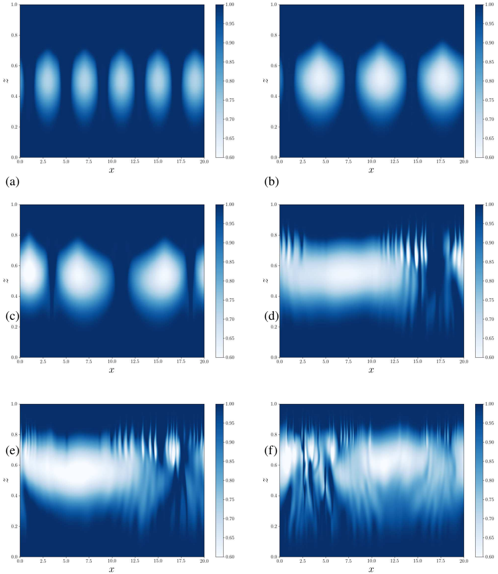
Figure 9: Snapshots of relative humidity in a statistically equilibrated state for M = 0.19 at (a) Ra = 2 \times 10^5 , (b) Ra = 1 \times 10^6 , (c) Ra = 2 \times 10^6 , (d) Ra = 2 \times 10^7 , (e) Ra = 5 \times 10^7 , (f) Ra = 2.5 \times 10^8 .
