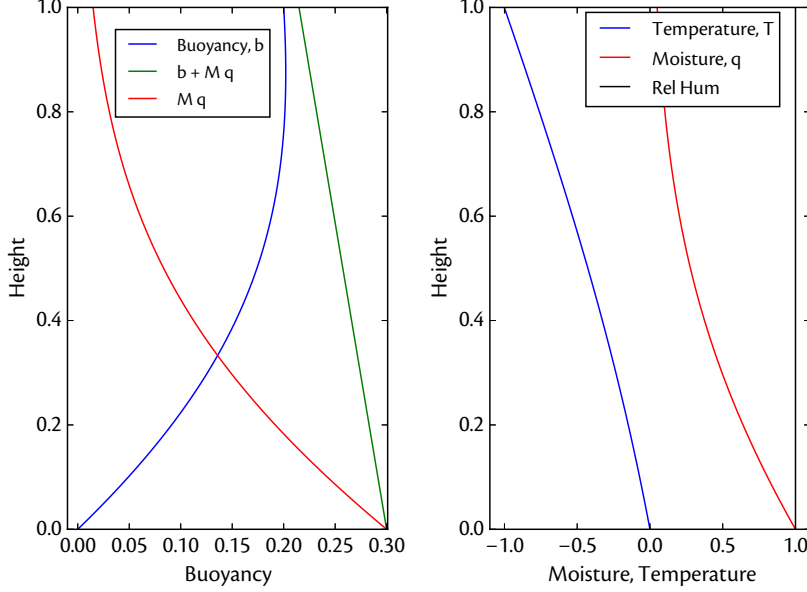
Figure 1: The drizzle solution with saturated upper and lower boundaries. The boundary conditions are that b = 0 at z = 0 and b = 0.2 at z = 1 and q = q_s at both boundaries, thus giving the values of m (= b + Mq) at the boundaries. These solutions were obtained with M = 0.3 , \alpha = 3 and \beta = 1.2 .
