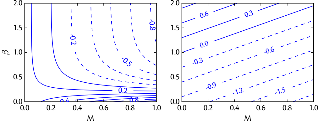
Figure 3: Contour plot of the value of the vertical gradient of m(z) = b + Mq_s (i.e., \partial m/\partial z ) in the drizzle solution as a function of \beta and M , with \alpha = 3 . The left plot imposes values of b(0) = 0 and b(1) = 0.2 with T = b - \beta z . The right plot has T(0) = 0 and T(1) = -1 , with b = T + \beta z . The boundary values of q_s are calculated given the appropriate value of T . Convective instability is possible in the region of dashed lines.
