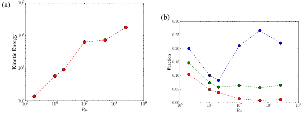
Figure 14: (a) Kinetic energy as a function of Ra . (b) Area fraction of near-saturated upflows as a function of Ra , with three different criteria. The blue line requires w > 0 and RH > 0.95 , the green line requires w > 0.02w_{\max} and RH > 0.95 and red line requires w > 0.1w_{\max} and RH > 0.95 .
