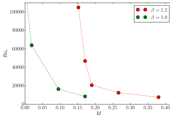
Figure 4: Stability of the linear drizzle solution. Graph of Ra_c versus M for the drizzle solution at \beta = 1 (green) and \beta = 1.2 (red). The dots mark the numerically determined stability boundary, with instability occurring above and to the right of the dots.
