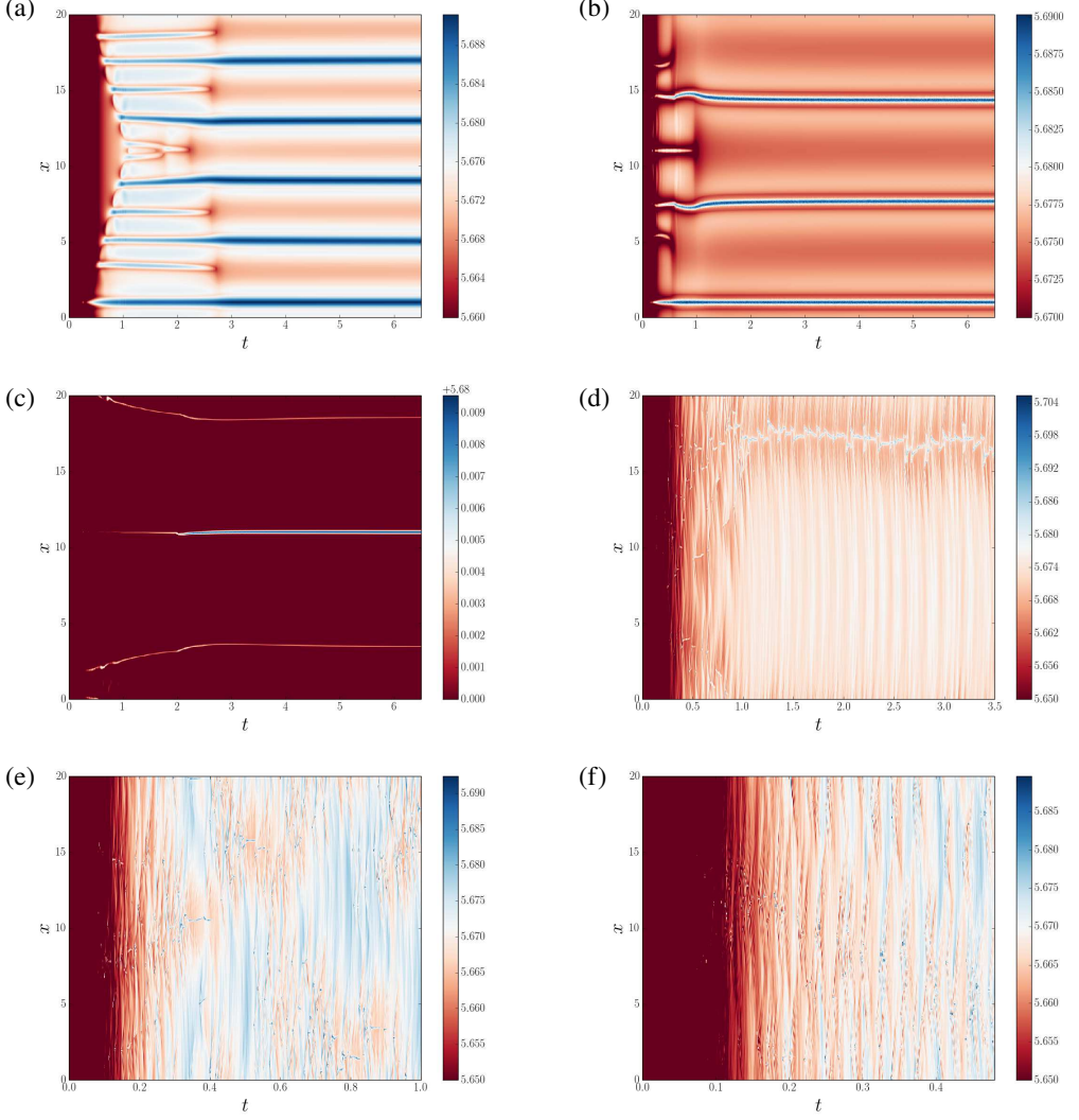
Figure 6: As for Fig. 5 but now Hövmoller plots at z = 0.5 for buoyancy for M = 0.19 at (a) Ra = 2 \times 10^5 , (b) Ra = 1 \times 10^6 , (c) Ra = 2 \times 10^6 , (d) Ra = 2 \times 10^7 , (e) Ra = 5 \times 10^7 , (f) Ra = 2.5 \times 10^8 .
