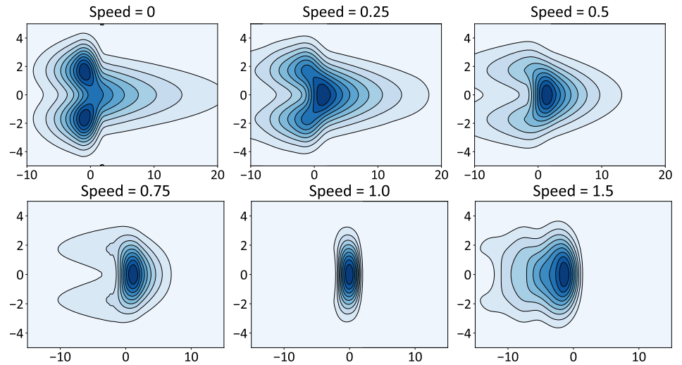
FIGURE 6 Pressure field in solutions of the shallow-water equations with a moving heat source. The x and y co-ordinates are scaled by the deformation radius and the speed is scaled by the gravity wave speed. The heat source is localized at the Equator, with a horizontal scale of about two deformation radii, and moves eastward at a constant speed. For plotting purposes the x -axis is shifted so that the centre of the heating at the time of the plots is always at x = 0 [Colour figure can be viewed at wileyonlinelibrary.com ]
