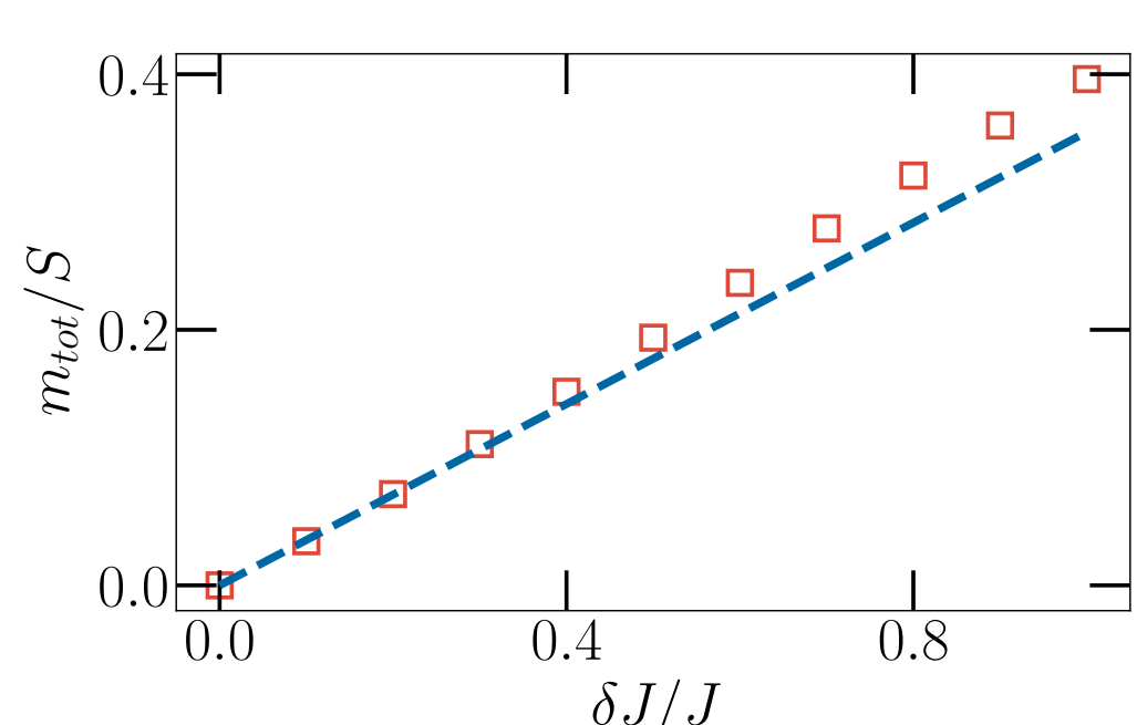
Uniform moment - disorder dependence in TLAF
