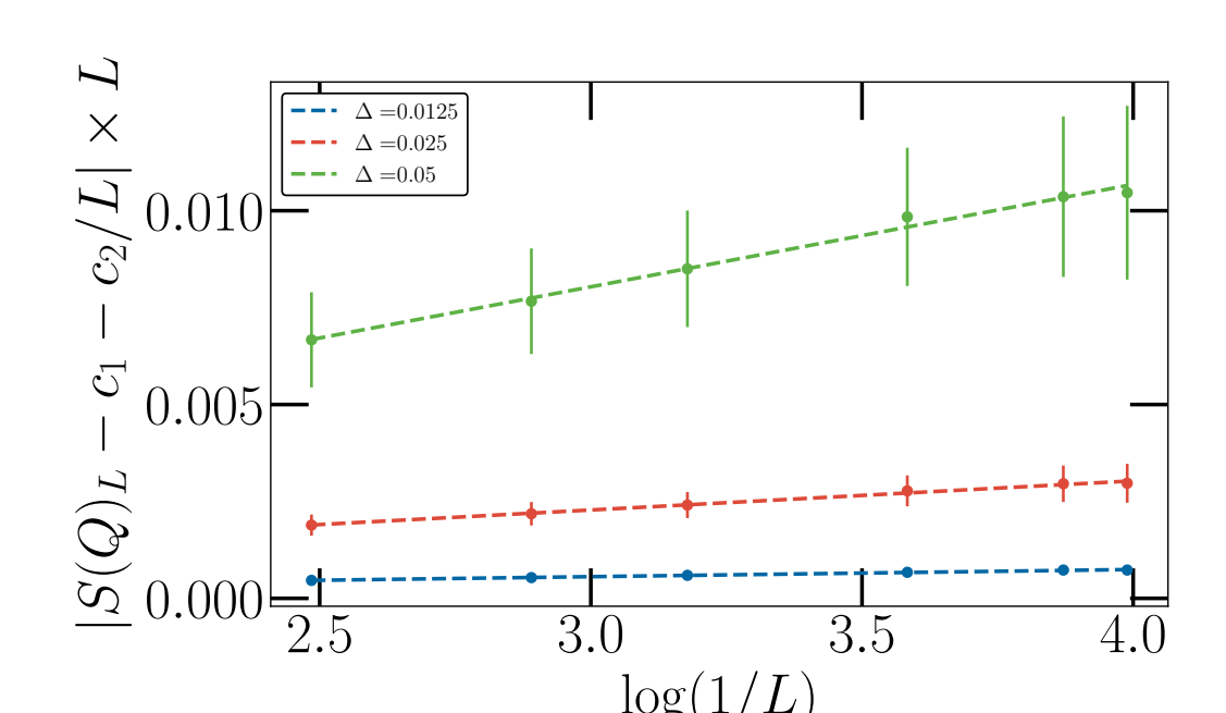
Sub-leading scaling for marginal behavior
