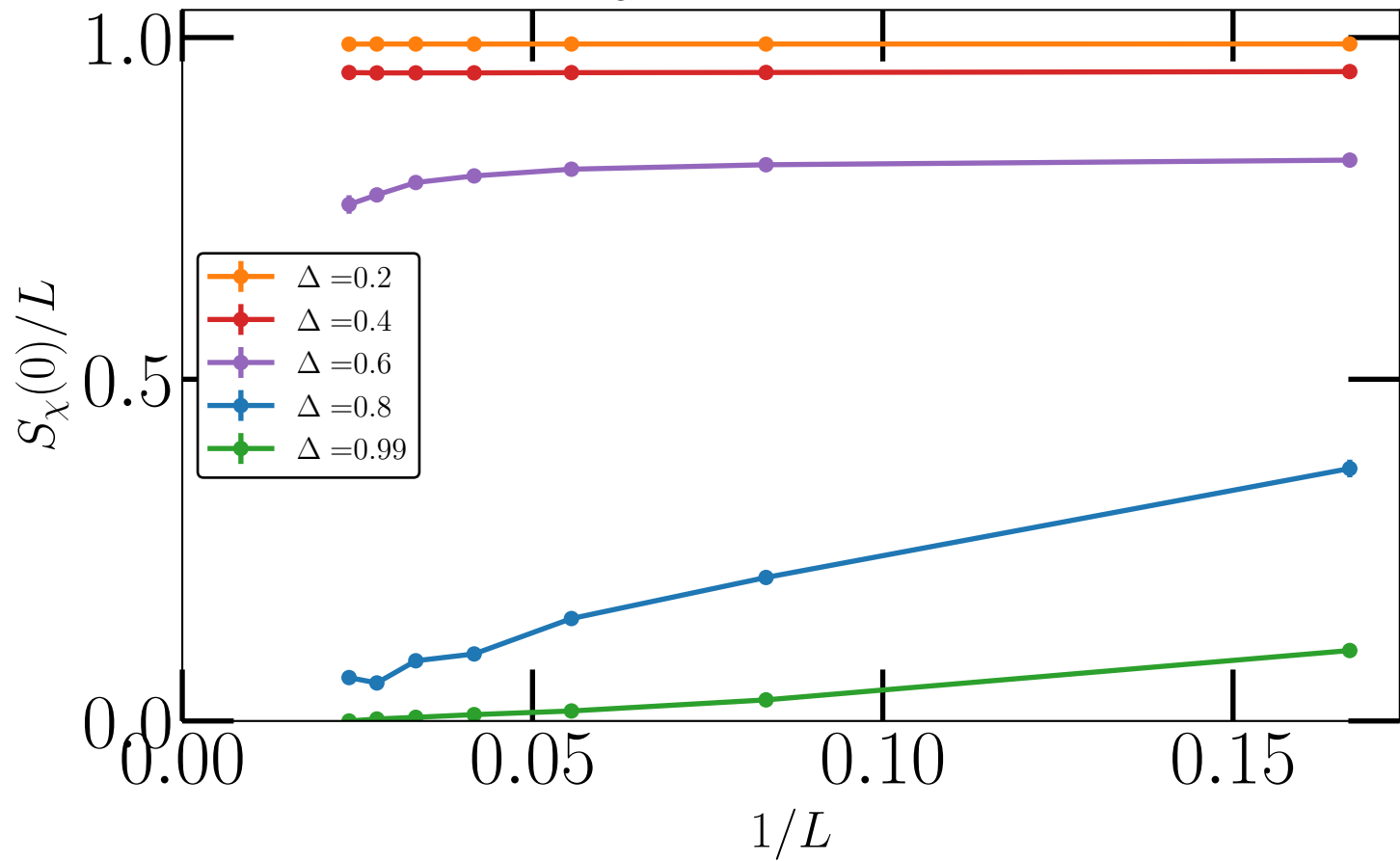
Heisenberg, Bimodal with \alpha=0.0 and P=0.25
