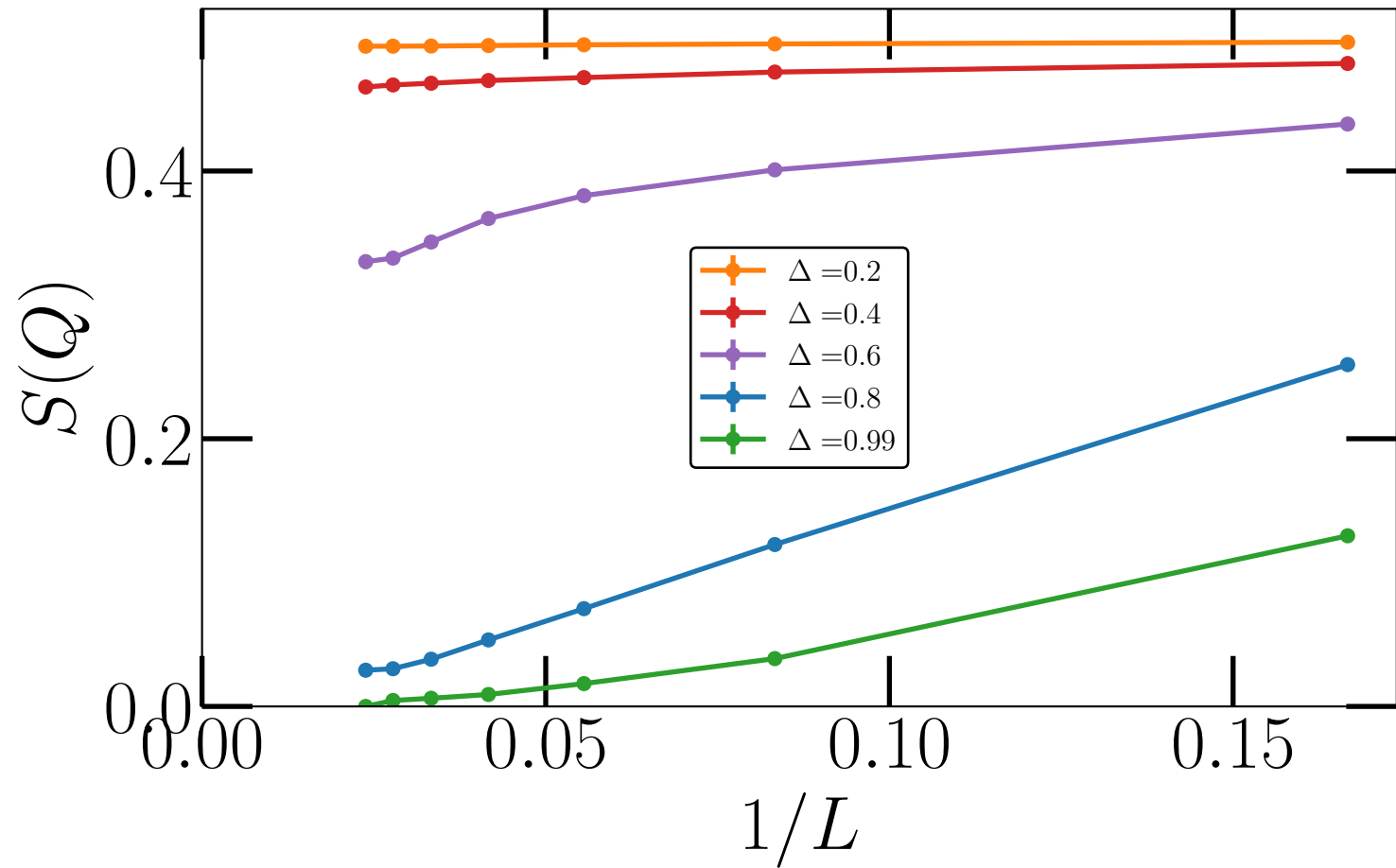
Heisenberg, Bimodal with \alpha=0.0 and P=0.5
