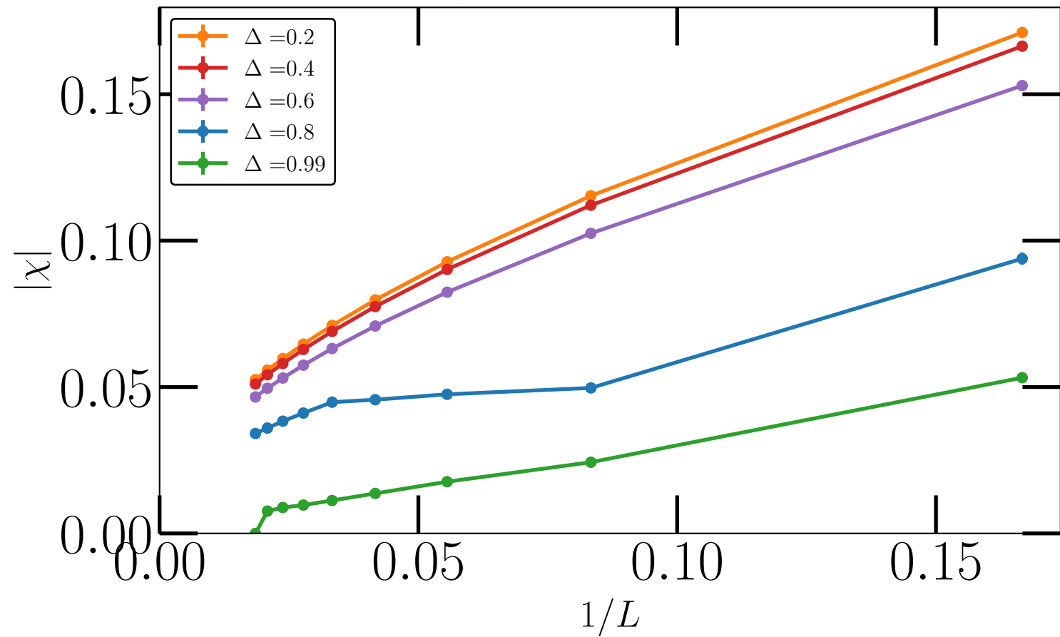
XY, Bimodal with \alpha=0.0 and P=0.5
