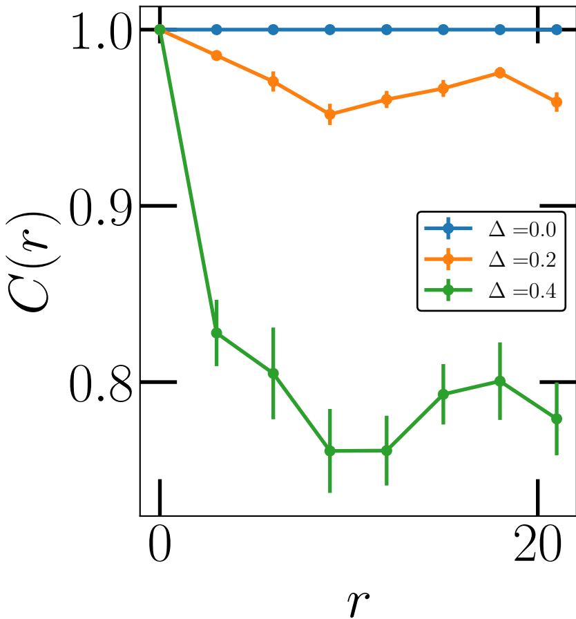
Triangular Lattice Heisenberg Model
