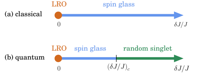
FIG. 1. Schematic ground-state phase diagram of chiral non-collinear magnets with quenched bond disorder in space dimension 1 < d \leq 2 , with \delta J/J parameterizing the disorder strength. (a) Classical limit ( S \rightarrow \infty ): The LRO of the clean system is destroyed for infinitesimal disorder in favor of a spin glass. (b) Quantum case: The spin glass turns into a random singlet (or valence bond) state at a critical level of disorder (whose numerical value depends on microscopic details).
