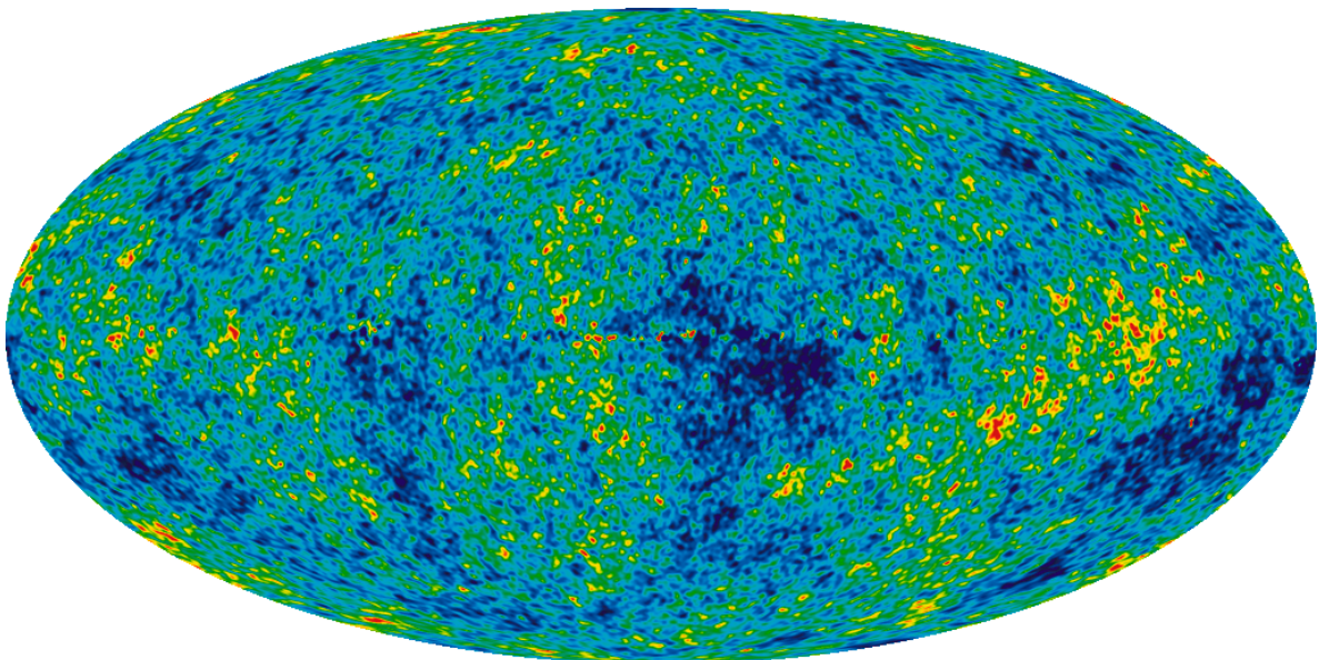
Figura 1: The detailed, all-sky picture of the infant universe created from seven years of WMAP data. The image reveals 13.7 billion year old temperature fluctuations (shown as color differences) that correspond to the seeds that grew to become the galaxies. The signal from the our Galaxy was subtracted using the multi-frequency data. This image shows a temperature range of \pm 200 microKelvin. Credit: NASA / WMAP Science Team
