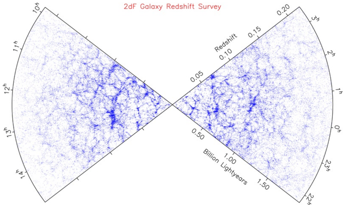
Figura 6: Galaxy distribution from the complete 2dFGRS
