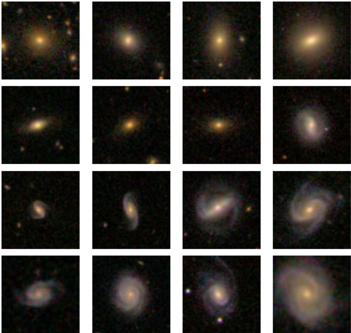
Figura 5: SDSS cutout images galaxies of different morphological type. From top to bottom: Elliptical, Lenticular, Barred and Spiral galaxies. Each image is 48 \times 48 \text{ arcsec}^2
