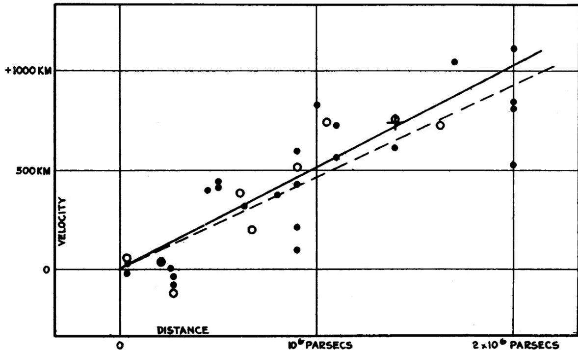
Figura 2: Hubble Law - Velocity-Distance Relation among Extra-Galactic Nebulae. Radial velocities, corrected for solar motion, are plotted against distances estimated from involved stars and mean luminosities of nebulae in a cluster. The black discs and full line represent the solution for solar motion using the nebulae individually; the circles and broken line represent the solution combining the nebulae into groups; the cross represents the mean velocity corresponding to the mean distance of 22 nebulae whose distances could not be estimated individually.
