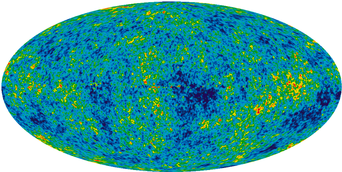
Figure 5: The detailed, all-sky picture of the infant universe created from seven years of WMAP data. The image reveals 13.7 billion year old temperature fluctuations (shown as color differences) that correspond to the seeds that grew to become the galaxies. The signal from the our Galaxy was subtracted using the multi-frequency data. This image shows a temperature range of \pm 200 microKelvin. Credit: NASA / WMAP Science Team
