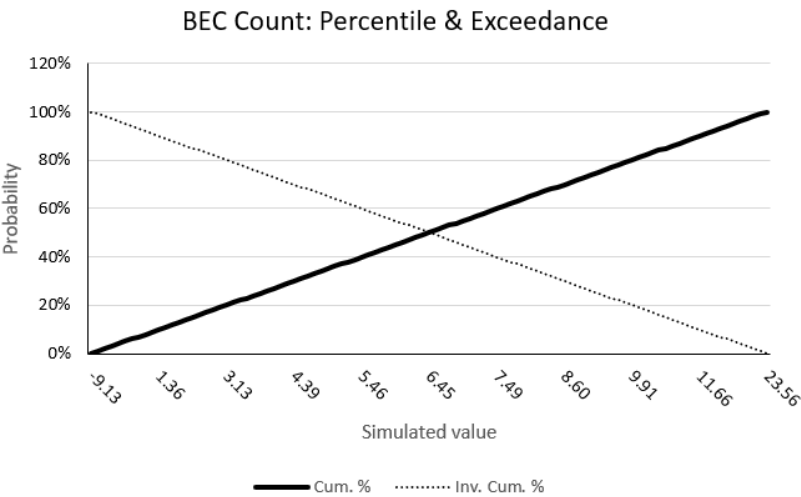
Fig. 3.50: A Monte Carlo simulation suggests that there is a 90% chance that 1 business email compromise event will occur within the sample. there is a 50% chance that 6 business email compromise events will occur. There is a 10% chance that 11 business email compromise event will occur within the sample.[144] [145]
