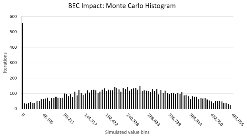
Fig. 3.51: We ran a Monte Carlo simulation of 10,000 iterations to spread random instances between confidence intervals taken from means of a seven year sample. We set a lower bound that the event would cost at $0. We set an upper bound that the event would cost $481,055.[146] [147]
