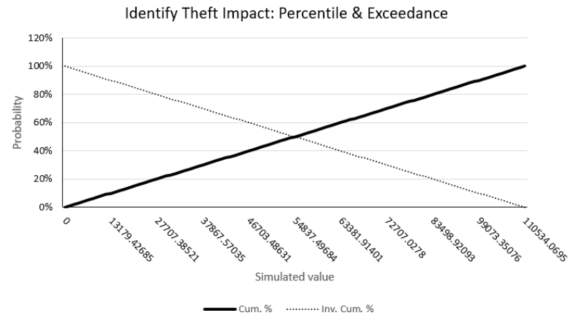
Fig. 3.48: A Monte Carlo simulation suggests that there is a 90% probability that identity theft events will cost $13,179.42 or more in a year. There is a 50% likelihood that they will cost at least $54,837.49 in a year. There is a 10% chance that they will cost $99,073.35 or more in a year. [140] [141]
