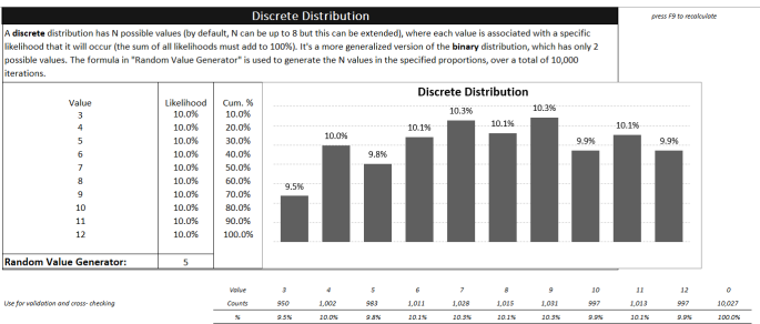
Fig. 3.42: We ran a Monte Carlo simulation of 10,000 iterations with a discrete distribution to spread random instances between upper and lower bounds taken from the means of seven year samples. We bounded between and possible CYBERCRIME events over a year.[128] [129]
