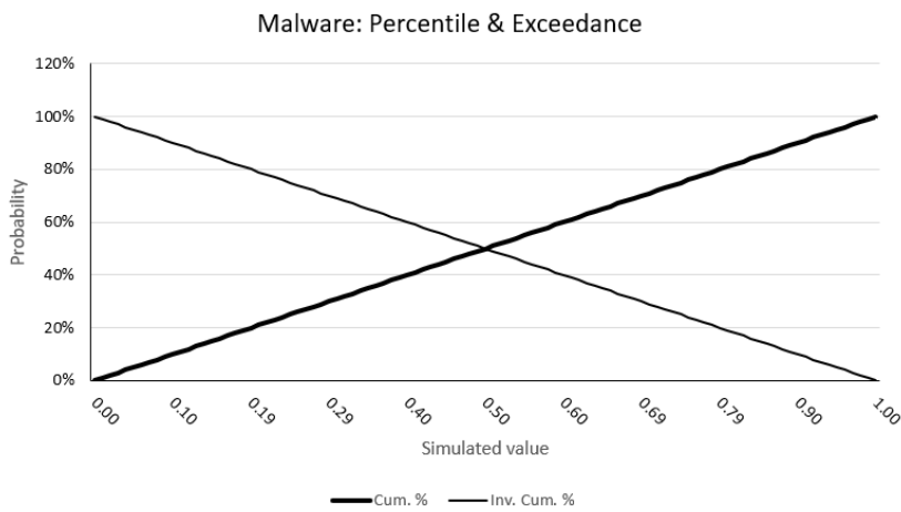
Fig. 3.14: The Monte Carlo simulation determined that there would be a 50% chance of malware. [222] [223]
