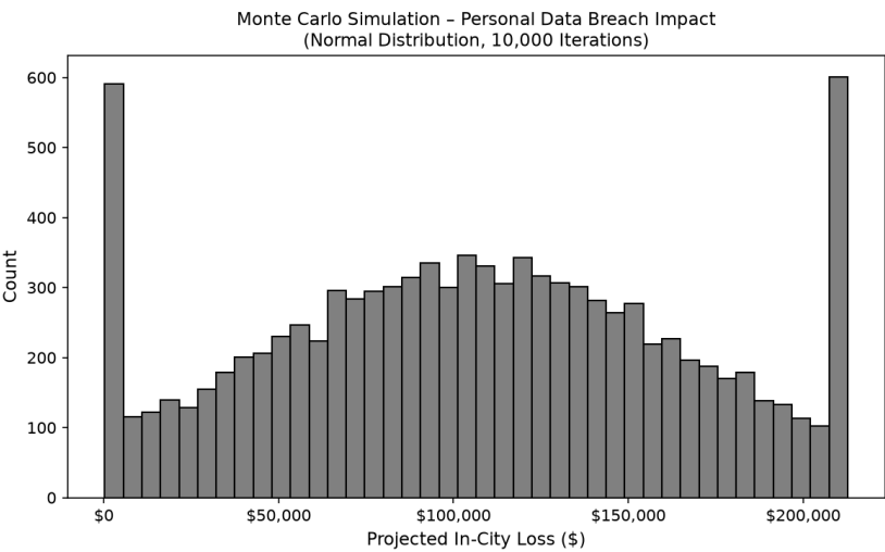
Fig. 5.14: We ran a Monte Carlo simulation of 10,000 iterations with a normal distribution to spread random instances between bounds taken from means of seven year samples. We set a lower bound that the events would cost at $270.50. We set an upper bound that the events would cost $212,708.42.[51] [52]
