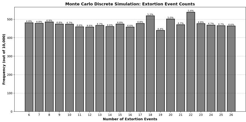
Fig. 5.29: We ran a Monte Carlo simulation of 10,000 iterations with a discrete distribution to spread random instances between upper and lower bounds taken from the means of seven year samples. We bounded between 6 and 26 possible extortion events over a year.[95] [96]
