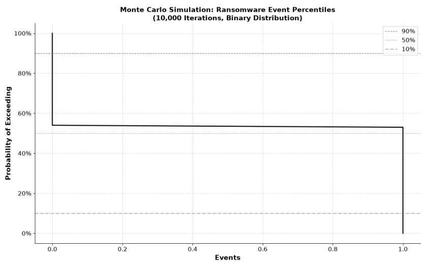
Fig. 5.23: A Monte Carlo simulation suggests that there is a 50% probability that 0.5 or more ransomware events will occur within the sample. This unusual result is because the confidence bounds are between 0 and 1. We interpret this as a 50% probability that one malware event will occur. [76] [77]
