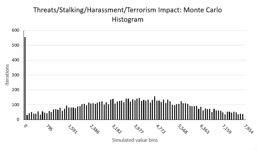
Fig. 5.33: We ran a Monte Carlo simulation of 10,000 iterations to spread random instances between confidence intervals taken from means of a seven year sample. We set a lower bound that the event would cost at $0. We set an upper bound that the event would cost $7,954.[103] [104]
