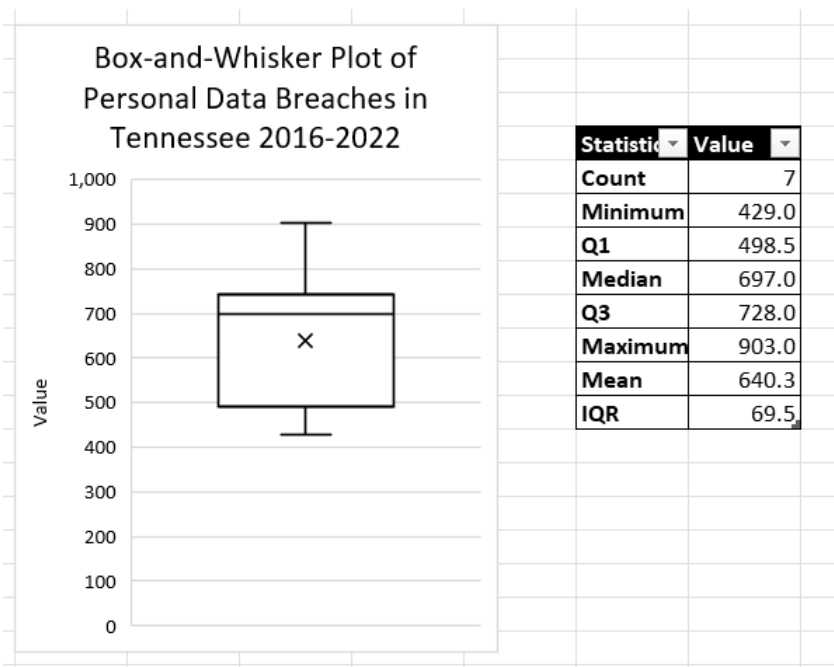
Fig. 5.3: Seven year summary of Personal Data Breaches in Tennessee reported to IC3.
