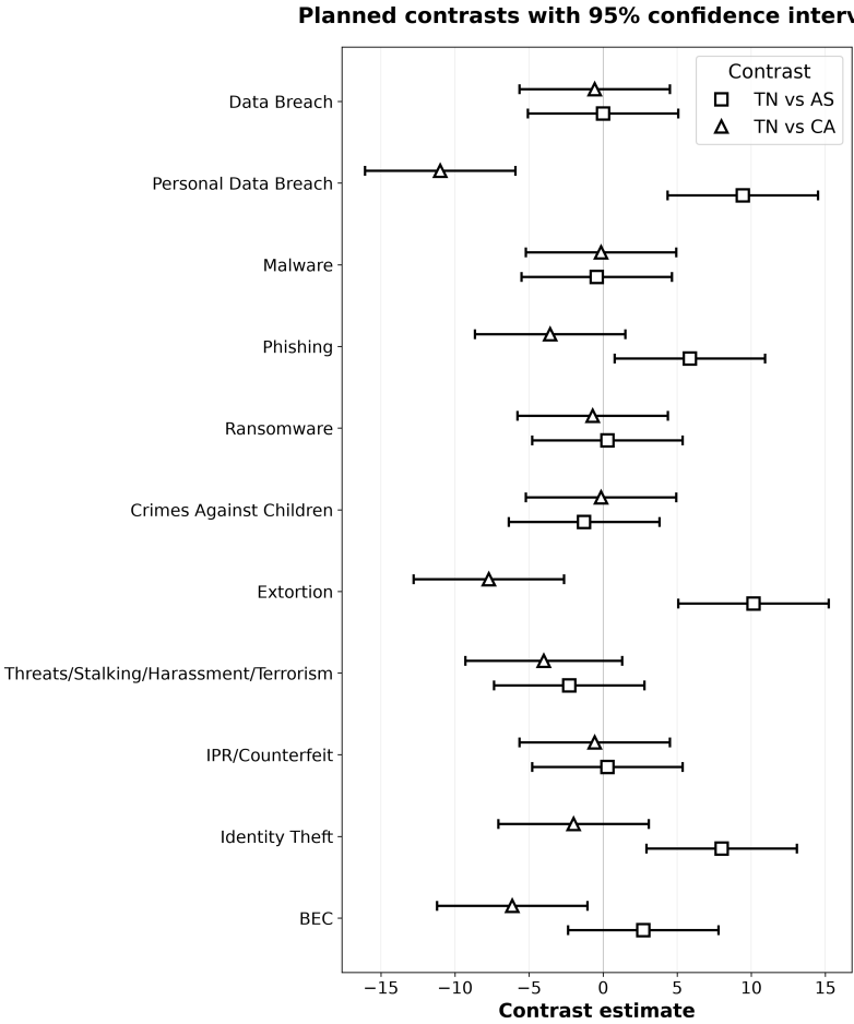
Fig. 5.45: Planned contrast estimates and 95% confidence intervals.
