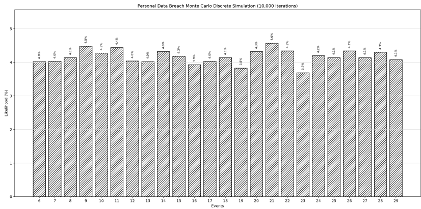
Fig. 5.13: We ran a Monte Carlo simulation of 10,000 iterations with a discrete distribution to spread random instances between upper and lower bounds taken from the means of seven year samples. We bounded between 6 and 29 possible personal data breach events over a year.[49] [50]
