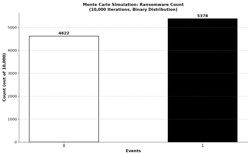
Fig. 5.22: We ran a Monte Carlo simulation of 10,000 iterations to spread random instances between confidence intervals taken from means of a seven year sample. We bounded between 0 and 1 possible ransomware events over a year.[74] [75]
