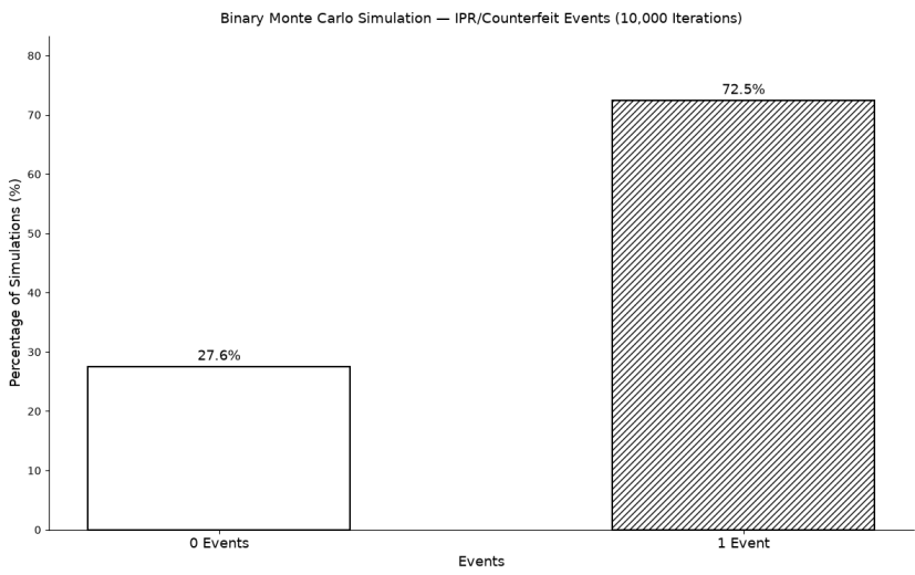
Fig. 5.35: We ran a Monte Carlo simulation of 10,000 iterations with a binary distribution to spread random instances between upper and lower bounds taken from the means of seven year samples. We bounded between 0 and 1 possible intellectual property rights (IPR) events over a year.[114] [115]
