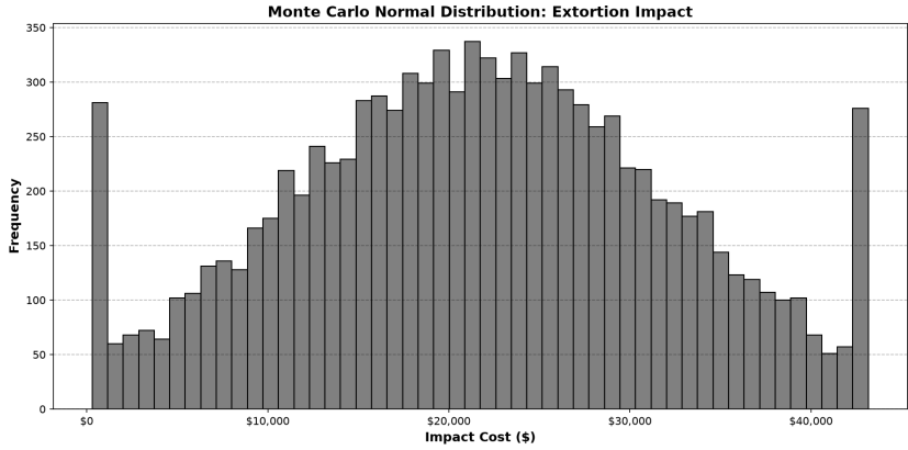
Fig. 5.30: We ran a Monte Carlo simulation of 10,000 iterations with a normal distribution to spread random instances between bounds taken from means of seven year samples. We set a lower bound that the events would cost at $300. We set an upper bound that the events would cost $43,167.06. [97] [98]
