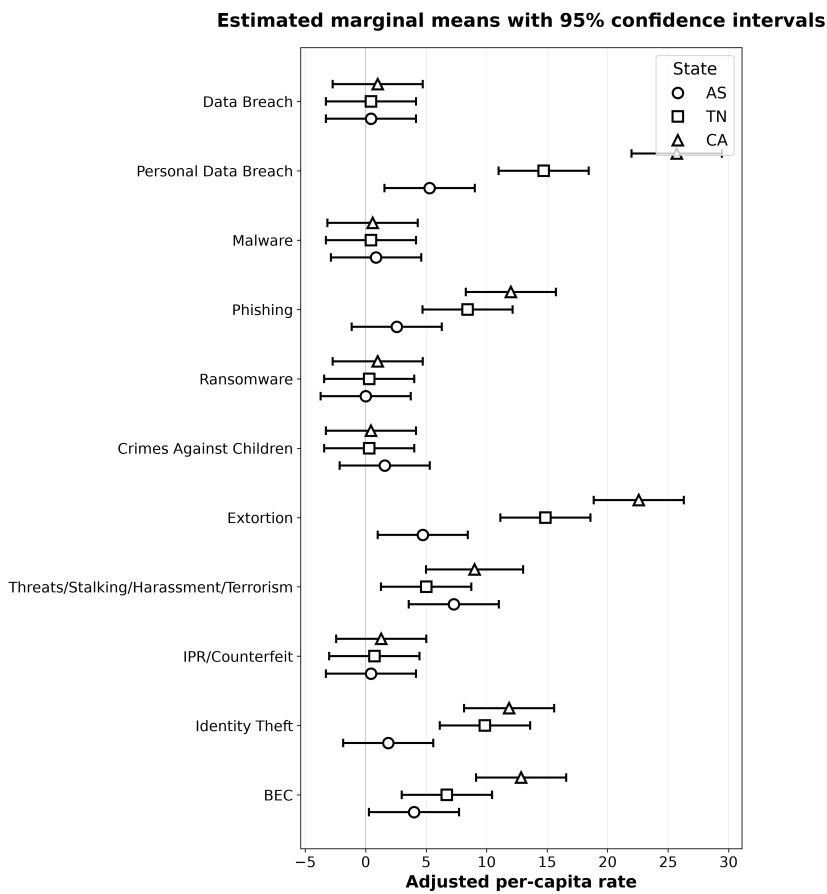
Fig. 5.44: Estimated marginal means and 95% confidence intervals.
