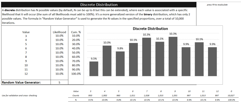
Fig. 5.47: We ran a Monte Carlo simulation of 10,000 iterations with a discrete distribution to spread random instances between confidence intervals taken from the means of seven year samples. We bounded between 3 and 12 possible phishing events over a year.[134] [135]
