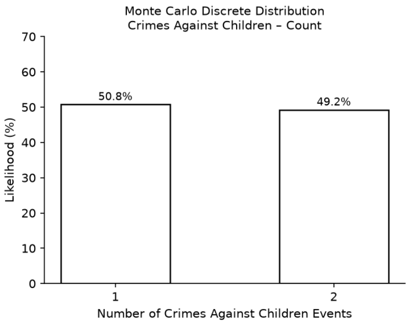
Fig. 5.26: We ran a Monte Carlo simulation of 10,000 iterations with a discrete distribution to spread random instances between upper and lower bounds taken from the means of seven year samples. We bounded between 1 and 2 possible crimes against children events over a year.[89] [90]
