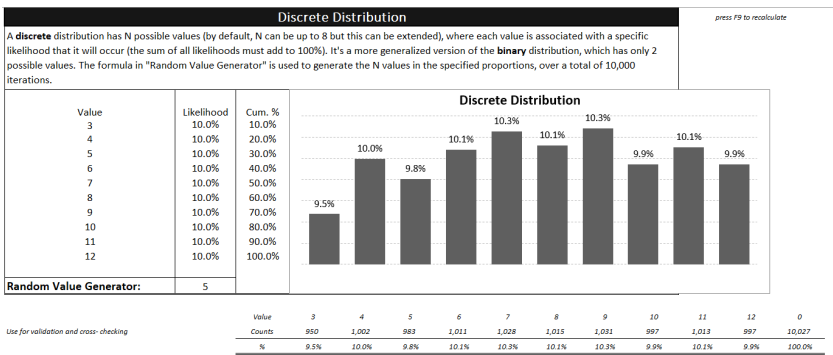
Fig. 5.19: We ran a Monte Carlo simulation of 10,000 iterations with a discrete distribution to spread random instances between confidence intervals taken from the means of seven year samples. We bounded between 3 and 12 possible phishing events over a year.[68] [69]
