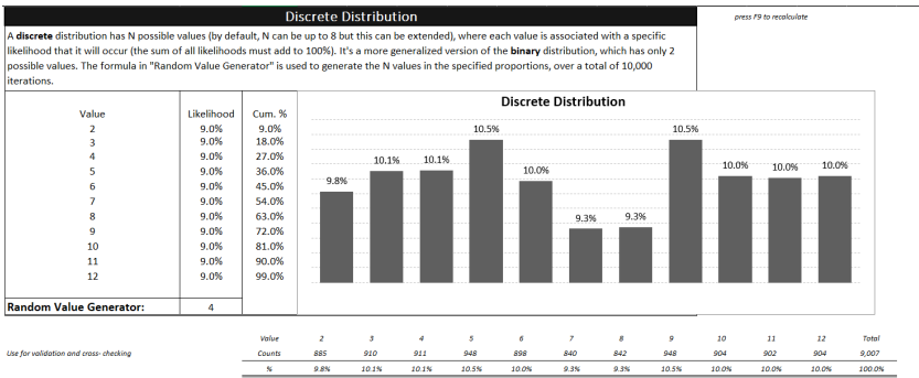
Fig. 5.38: We ran a Monte Carlo simulation of 10,000 iterations with a discrete distribution to spread random instances between confidence intervals taken from the means of seven year samples. We bounded between 2 and 12 possible identity theft events over a year.[120] [121]
