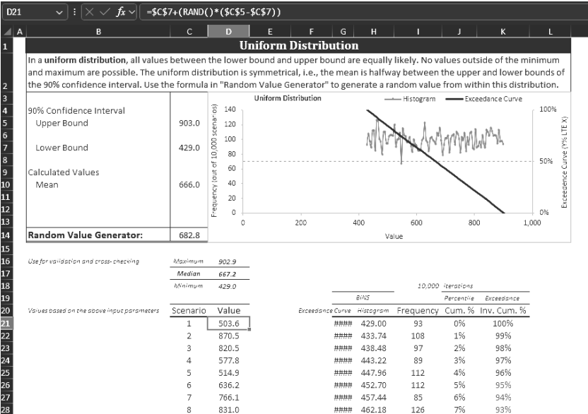
Fig. 5.1: Example run of a Monte Carlo simulation using state-level data to set bounds. Here we chose Personal data breach victim counts from 2016 and 2022 as upper and lower bounds. 10,000 rows projected randomized values between these bounds and determined mean and counts by confidence interval. [1]
