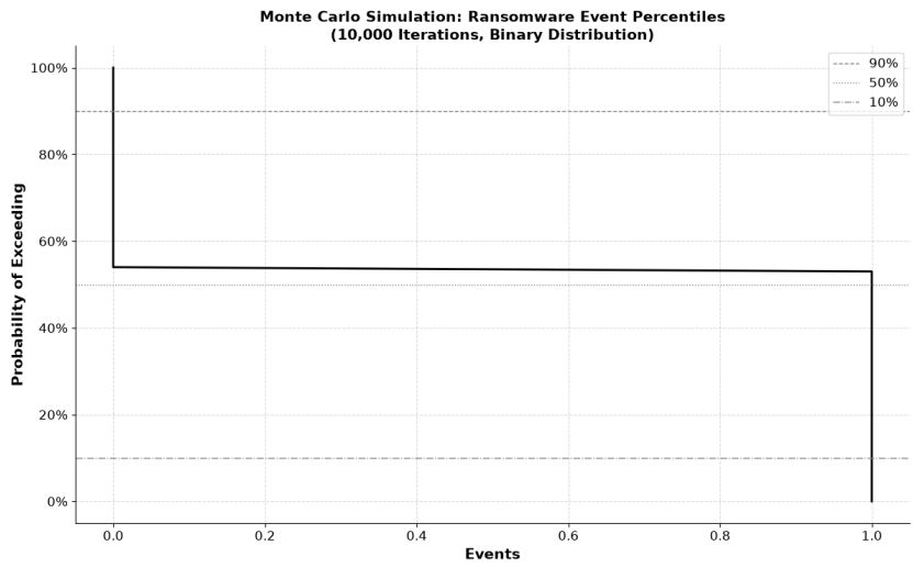
Fig. 5.49: A Monte Carlo simulation suggests that there is a 50% probability that 0.5 or more ransomware events will occur within the sample. This unusual result is because the confidence bounds are between 0 and 1. We interpret this as a 50% probability that one malware event will occur. [138] [139]
