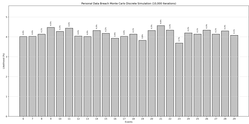
Fig. 5.46: We ran a Monte Carlo simulation of 10,000 iterations with a discrete distribution to spread random instances between upper and lower bounds taken from the means of seven year samples. We bounded between 6 and 29 possible personal data breach events over a year.[132] [133]
