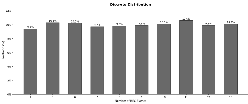
Fig. 5.41: We ran a Monte Carlo simulation of 10,000 iterations with a discrete distribution to spread random instances between confidence intervals taken from the means of seven year samples. We bounded between 4 and 13 possible business email compromise events over a year.[126] [127]
