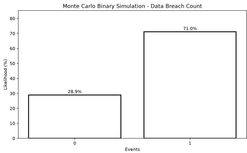
Fig. 5.10: We ran a Monte Carlo simulation of 10,000 iterations with a binary distribution to spread random instances between upper and lower bounds taken from the means of seven year samples. We bounded between 0 and 1 possible data breach events over a year.[43] [44]
