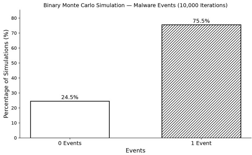
Fig. 5.16: We ran a Monte Carlo simulation of 10,000 iterations with a binary distribution to spread random instances between upper and lower bounds taken from the means of seven year samples. We bounded between 0 and 1 possible malware events over a year.[62] [63]
