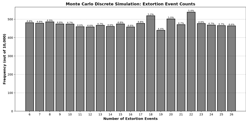
Fig. 5.50: We ran a Monte Carlo simulation of 10,000 iterations with a discrete distribution to spread random instances between upper and lower bounds taken from the means of seven year samples. We bounded between 6 and 26 possible extortion events over a year.[140] [141]
