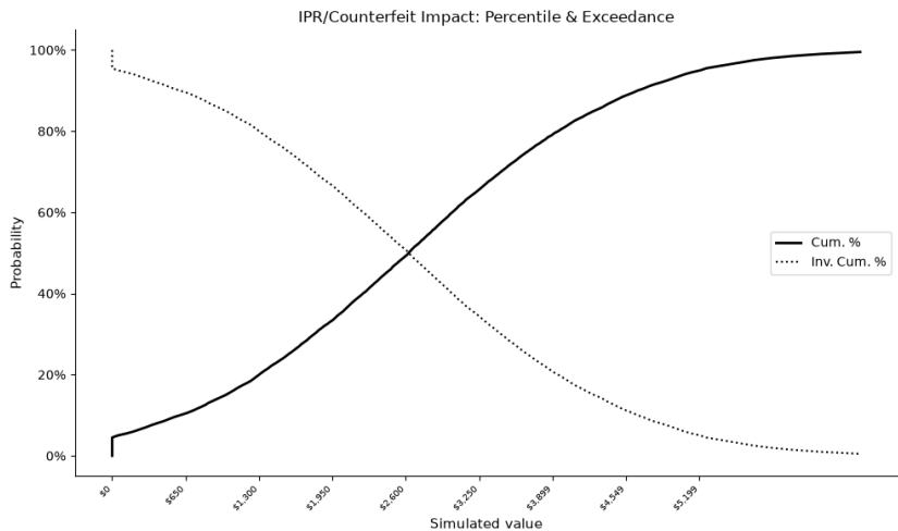
Fig. 5.36: We ran a Monte Carlo simulation of 10,000 iterations with a normal distribution to spread random instances between bounds taken from means of seven year samples. We set a lower bound that the events would cost at $0. We set an upper bound that the events would cost $5,199. [116] [117]
