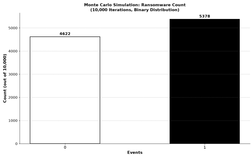
Fig. 5.48: We ran a Monte Carlo simulation of 10,000 iterations to spread random instances between confidence intervals taken from means of a seven year sample. We bounded between 0 and 1 possible ransomware events over a year.[136] [137]
