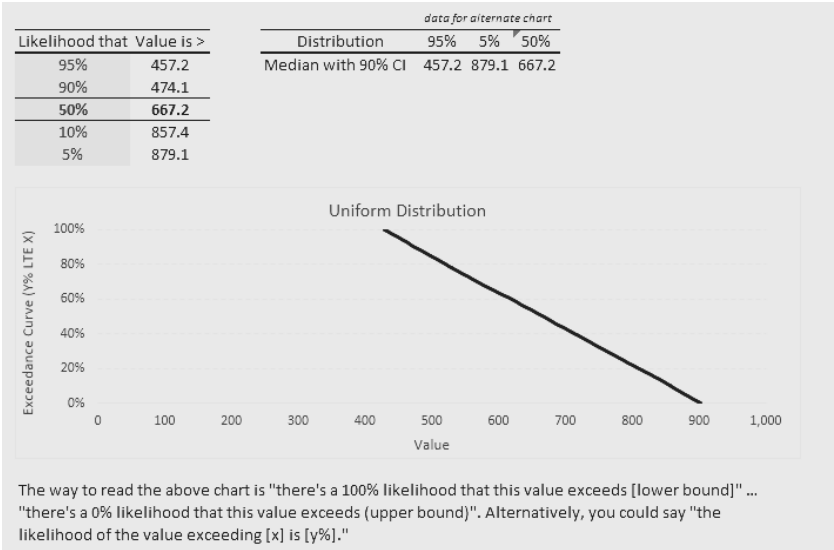
Fig. 5.2: Example results of applying Monte Carlo simulation to forecasting. Here we see the assertion that there is a 90% likelihood that the number of victims will be between 457 and 879; the mean of the simulation was 667.[5]
