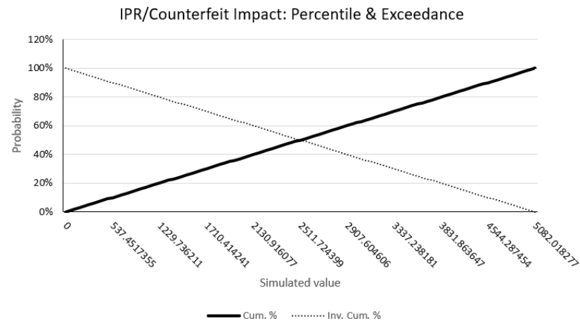
Fig. 3.42: A Monte Carlo simulation suggests that there is a 90% probability that intellectual property rights events will cost $537.45 or more in a year. There is a 50% likelihood that they will cost $2,511.72 or more in a year. There is a 10% chance that they will cost $4,544.28 or more in a year. [128] [129]
