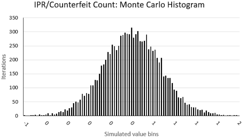
Fig. 3.43: We ran a Monte Carlo simulation of 10,000 iterations to spread random instances between confidence intervals taken from means of a seven year sample. We bounded between 0 and 11 possible identity theft events over a year.[130] [131]
