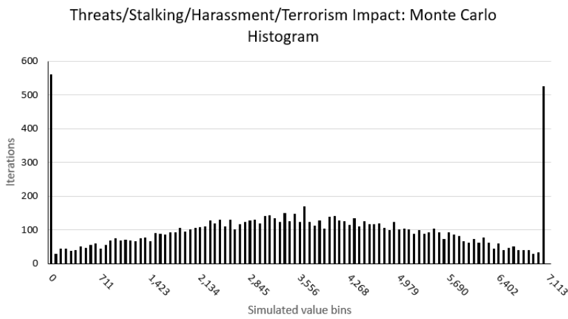
Fig. 3.37: We ran a Monte Carlo simulation of 10,000 iterations to spread random instances between confidence intervals taken from means of a seven year sample. We set a lower bound that the event would cost at $0. We set an upper bound that the event would cost $7,112.[111] [112]
