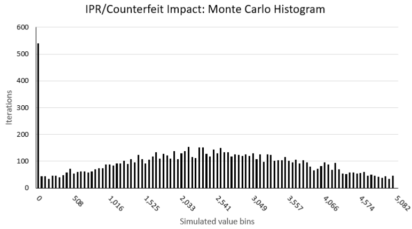
Fig. 3.41: We ran a Monte Carlo simulation of 10,000 iterations to spread random instances between confidence intervals taken from means of a seven year sample. We set a lower bound that the event would cost at $0. We set an upper bound that the event would cost $5,082.[126] [127]
