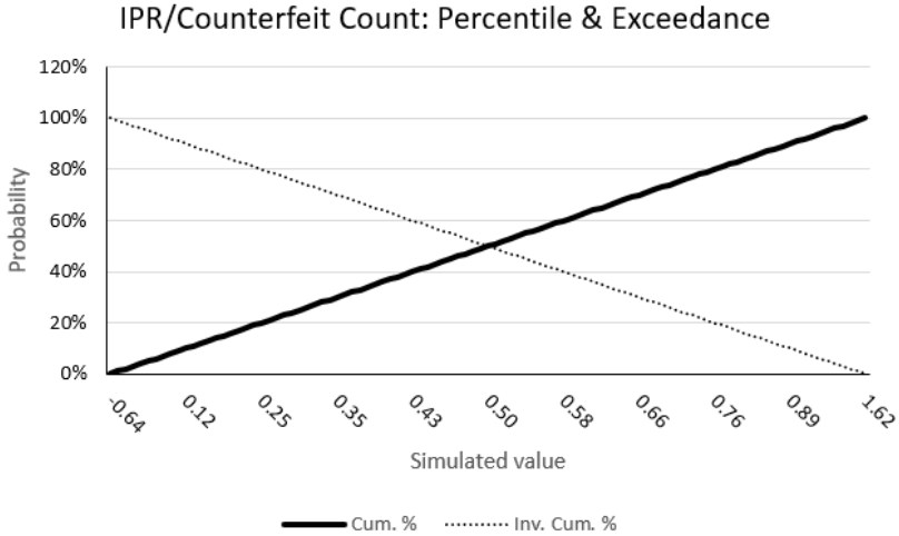
Fig. 3.40: A Monte Carlo simulation suggests that there is a 50% chance that an intellectual property rights event will occur within the sample. [124] [125]
