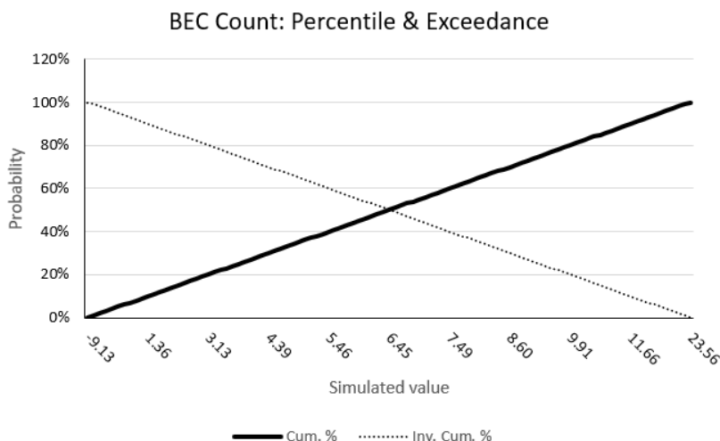
Fig. 3.52: A Monte Carlo simulation suggests that there is a 90% chance that 1 business email compromise event will occur within the sample. there is a 50% chance that 6 business email compromise events will occur. There is a 10% chance that 11 business email compromise event will occur within the sample.[148] [149]
