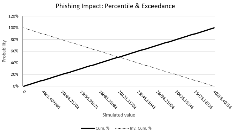
Fig. 3.24: A Monte Carlo simulation suggests that there is a 90% probability that phishing events will cost $4,661.40 or more in a year. There is a 50% likelihood that they will cost $20,179.13 or more in a year. There is a 10% chance that they will cost $35,678.52 or more in a year. [78] [79]
