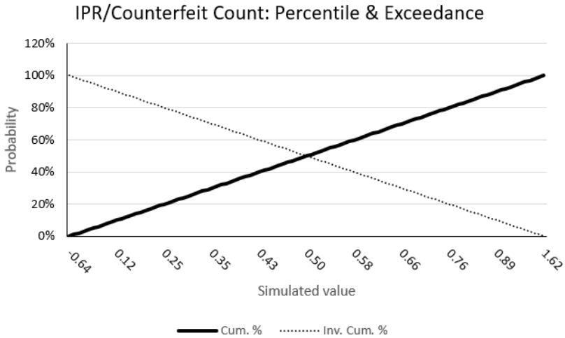
Fig. 3.44: A Monte Carlo simulation suggests that there is a 50% chance that an intellectual property rights event will occur within the sample. [132] [133]
