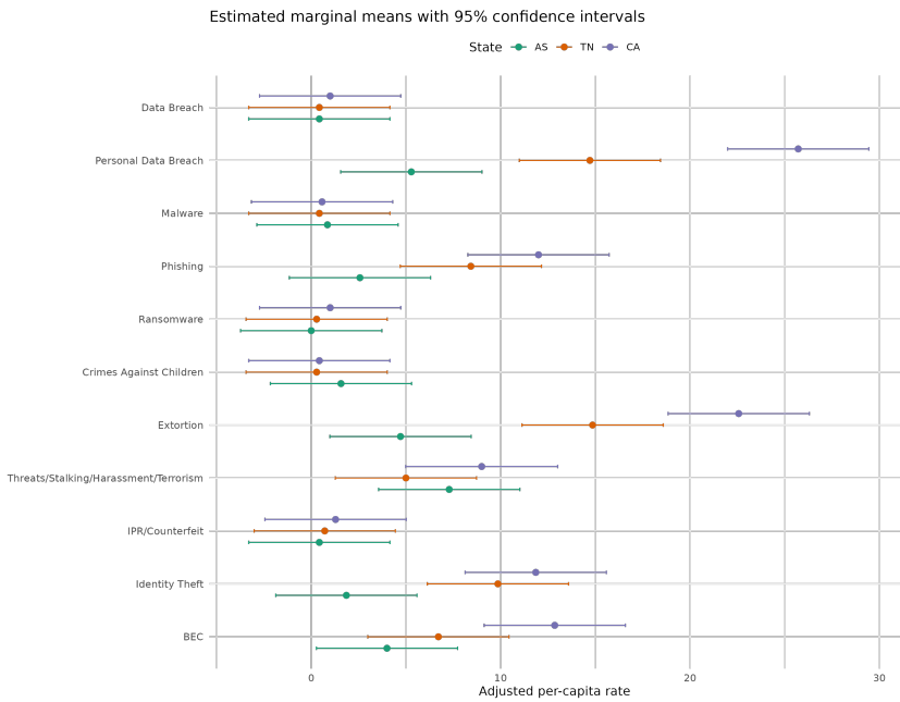
Fig. 3.51: Estimated marginal means and 95% confidence intervals.
