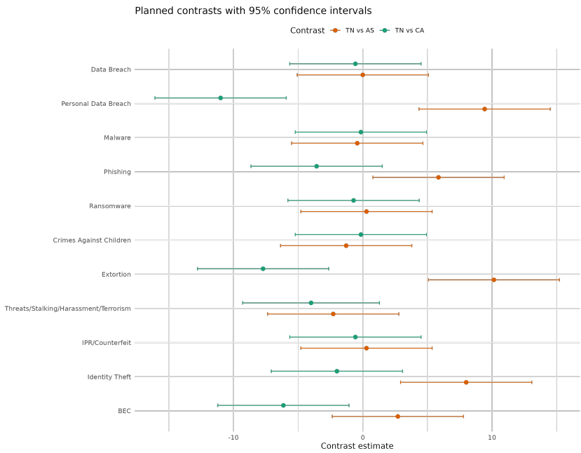
Fig. 3.52: Planned contrast estimates and 95% confidence intervals.
