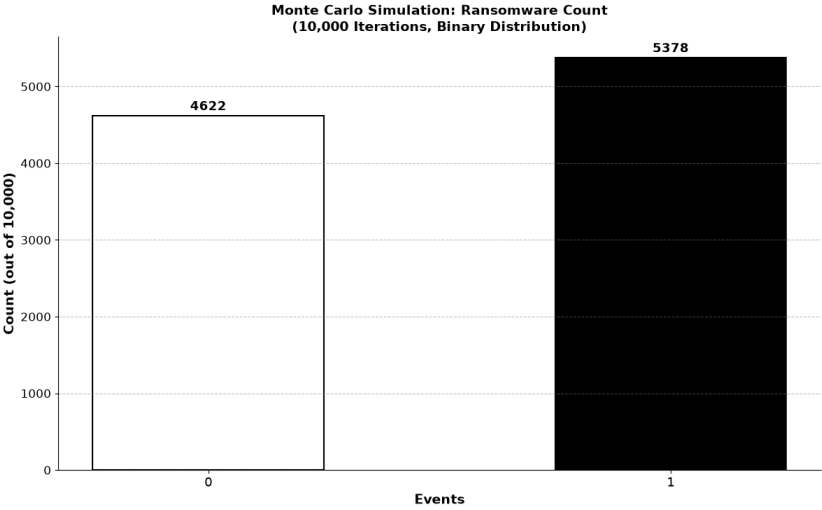
Fig. 3.22: We ran a Monte Carlo simulation of 10,000 iterations to spread random instances between confidence intervals taken from means of a seven year sample. We bounded between 0 and 1 possible ransomware events over a year.[74] [75]
