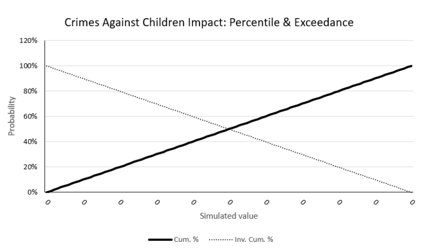
Fig. 3.30: Since the Monte Carlo simulation determined that there would be no reasonable chance of crimes against children in this sample, we can see that there would be no financial impact. [97] [98]
