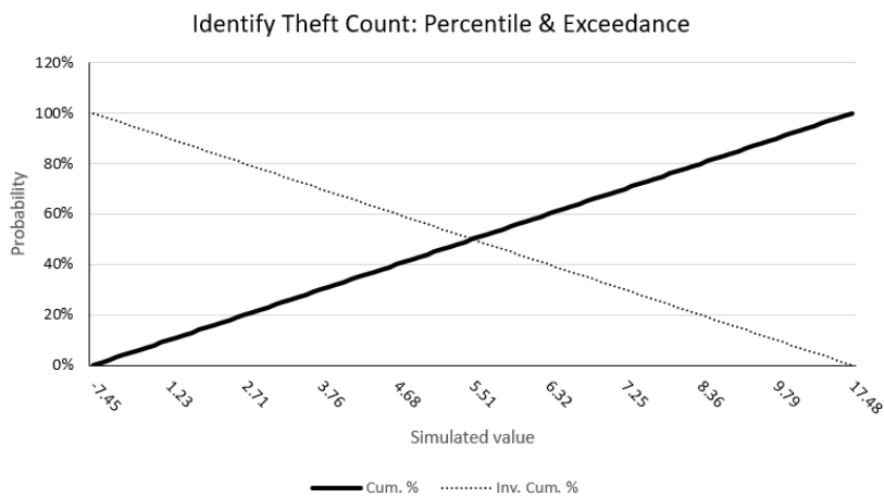
Fig. 3.43: A Monte Carlo simulation suggests that there is a 90% chance that 1 identity theft event will occur within the sample. There is a 50% chance that 5 identity theft events will occur. There is a 10% chance that 9 identity theft events will occur within the sample.[130] [131]
