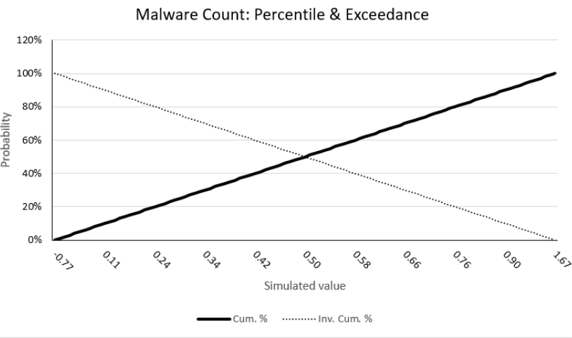
Fig. 3.19: A Monte Carlo simulation suggests that there is a 50% probability that 0.5 or more malware events will occur within the sample. This unusual result is because the confidence bounds are between 0 and 1. We interpret this as a 50% probability that one malware event will occur. [68] [69]
