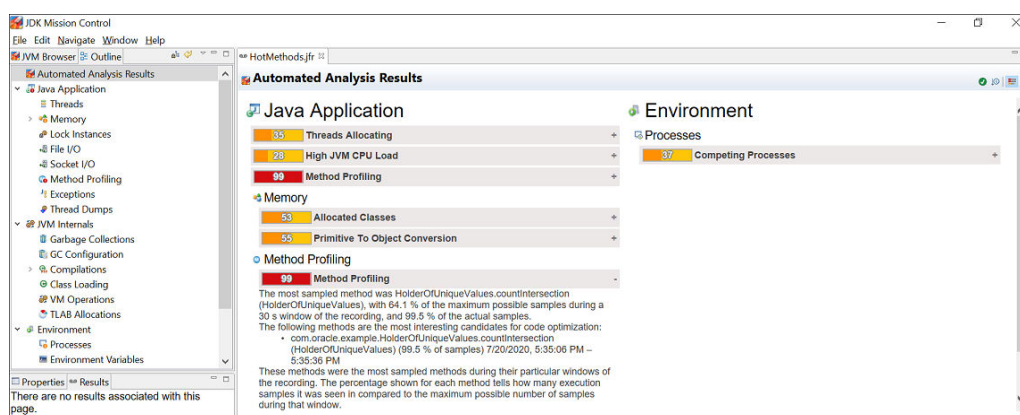
Figure 4-7 Code Execution Performance - Automated Analysis Results Page
