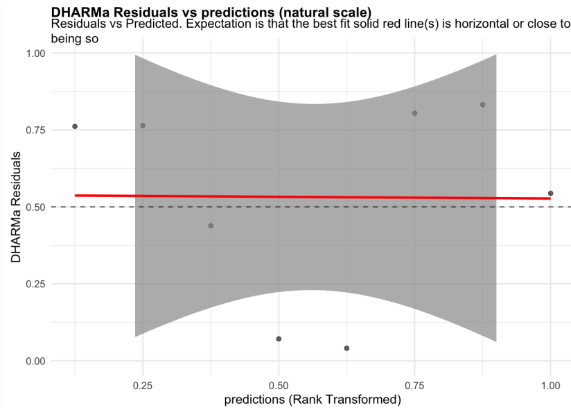
Figure 28: residuals_vs_predicted. Residuals vs Predicted Check the Residuals vs Fitted plots for good and bad examples here: https://library.virginia.edu/data/articles/diagnostic-plots
