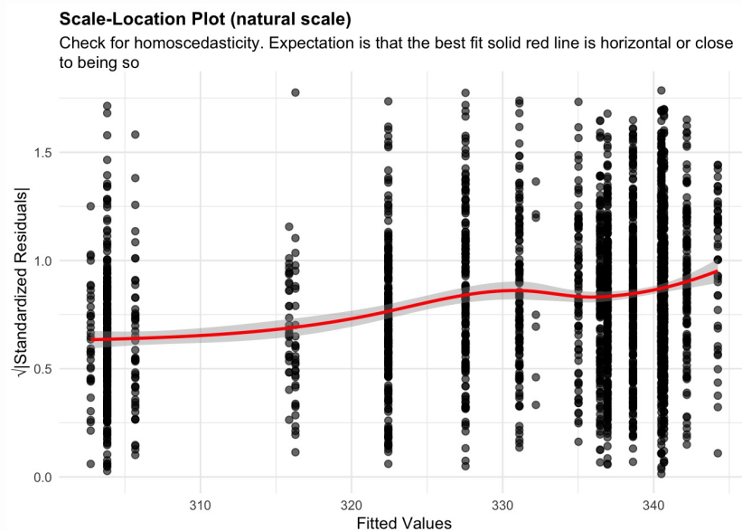
Figure 3: residuals homoscedasticity. Check for homoscedasticity (natural scale). Expectation is that the best fit solid red line is horizontal or close to being so. Check the Scale-Location plots for good and bad examples here: https://library.virginia.edu/data/articles/diagnostic-plots
