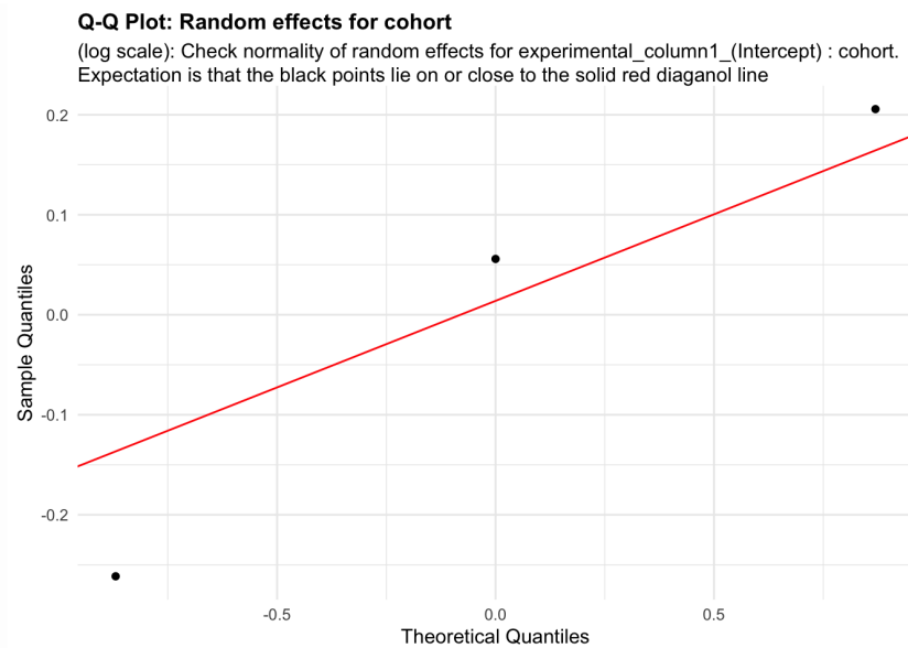
Figure 56: random_effects_QQ_2. Check normality of random effects for experimental_column1_(Intercept) (log scale): cohort. Expectation is that the black points lie on or close to the solid red diagonal line. Check the Normal Q-Q plots for good and bad examples here: https://library.virginia.edu/data/articles/diagnostic-plots
