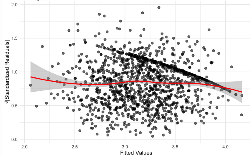
Figure 62: residuals_homoscedasticity. Check for homoscedasticity (log scale wo outlier). Expectation is that the best fit solid red line is horizontal or close to being so. Check the Scale-Location plots for good and bad examples here: https://library.virginia.edu/data/articles/diagnostic-plots
