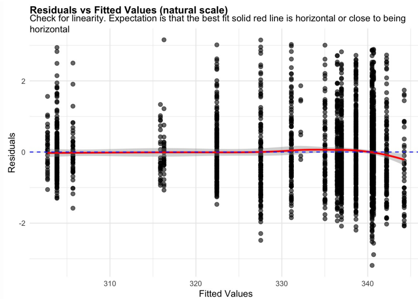
Figure 2: residuals vs fitted. Check for linearity (natural scale). Expectation is that the best fit solid red line is horizontal or close to being horizontal. Check the Residuals vs Fitted plots for good and bad examples here: https://library.virginia.edu/data/articles/diagnostic-plots
