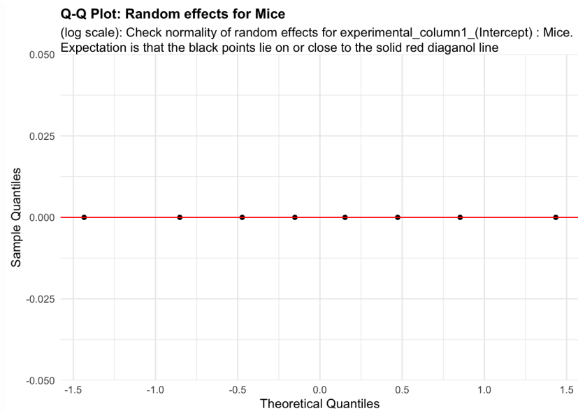
Figure 102: random_effects_QQ_2. Check normality of random effects for experimental_column1_(Intercept) (log scale): Mice. Expectation is that the black points lie on or close to the solid red diagonal line. Check the Normal Q-Q plots for good and bad examples here: https://library.virginia.edu/data/articles/diagnostic-plots
