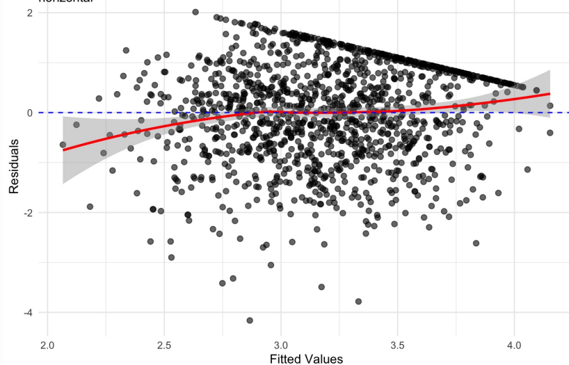
Figure 53: residuals_vs_fitted. Check for linearity (log scale). Expectation is that the best fit solid red line is horizontal or close to being horizontal. Check the Residuals vs Fitted plots for good and bad examples here: https://library.virginia.edu/data/articles/diagnostic-plots
