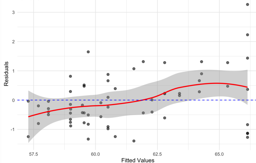
Figure 70: residuals_vs_fitted. Check for linearity (natural scale). Expectation is that the best fit solid red line is horizontal or close to being horizontal. Check the Residuals vs Fitted plots for good and bad examples here: https://library.virginia.edu/data/articles/diagnostic-plots
