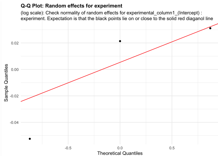
Figure 12: random_effects_QQ_2. Check normality of random effects for experimental_column1_(Intercept) (log scale): experiment. Expectation is that the black points lie on or close to the solid red diagonal line. Check the Normal Q-Q plots for good and bad examples here: https://library.virginia.edu/data/articles/diagnostic-plots
