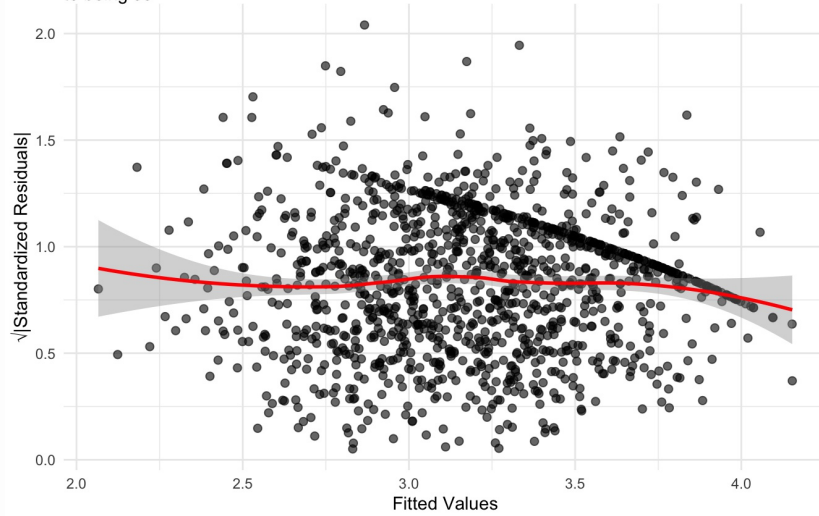
Figure 54: residuals_homoscedasticity. Check for homoscedasticity (log scale). Expectation is that the best fit solid red line is horizontal or close to being so. Check the Scale-Location plots for good and bad examples here: https://library.virginia.edu/data/articles/diagnostic-plots
