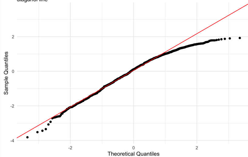
Figure 60: residuals_QQ. Check normality of residuals (log scale wo outlier). Expectation is that the black points lie on or close to the solid red diagonal line. Check the Normal Q-Q plots for good and bad examples here: https://library.virginia.edu/data/articles/diagnostic-plots
