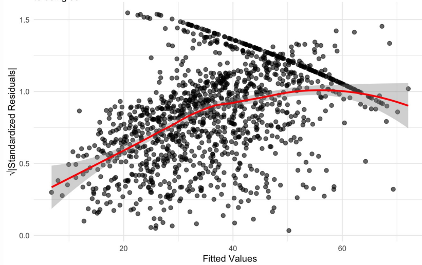
Figure 47: residuals_homoscedasticity. Check for homoscedasticity (natural scale). Expectation is that the best fit solid red line is horizontal or close to being so. Check the Scale-Location plots for good and bad examples here: https://library.virginia.edu/data/articles/diagnostic-plots
