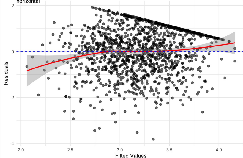
Figure 61: residuals_vs_fitted. Check for linearity (log scale wo outlier). Expectation is that the best fit solid red line is horizontal or close to being horizontal. Check the Residuals vs Fitted plots for good and bad examples here: https://library.virginia.edu/data/articles/diagnostic-plots
