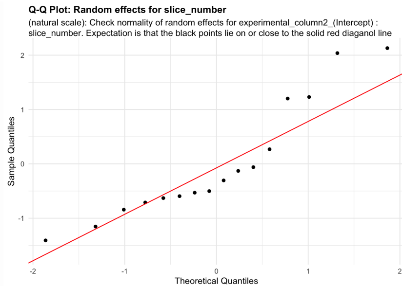
Figure 94: random_effects_QQ_1. Check normality of random effects for experimental_column2_(Intercept) (natural scale): slice_number. Expectation is that the black points lie on or close to the solid red diagonal line. Check the Normal Q-Q plots for good and bad examples here: https://library.virginia.edu/data/articles/diagnostic-plots
