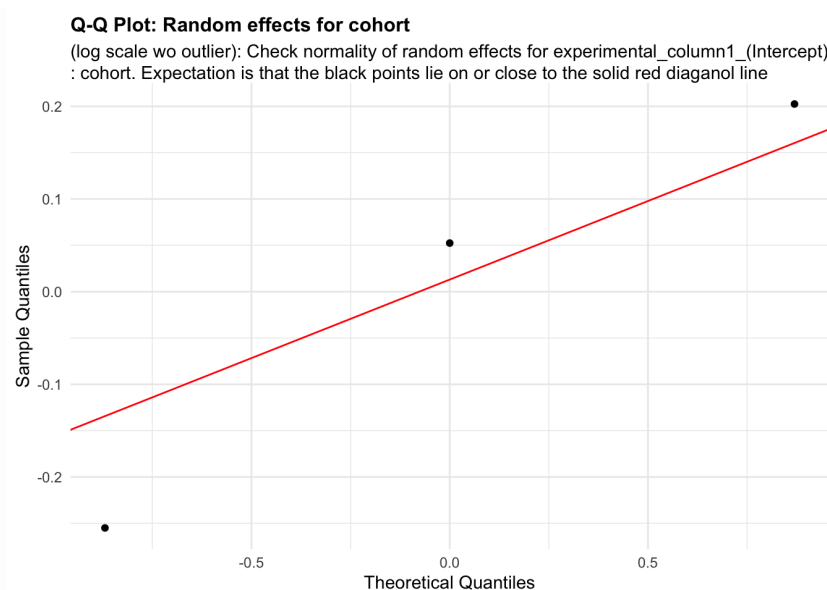
Figure 64: random_effects_QQ_2. Check normality of random effects for experimental_column1_(Intercept) (log scale wo outlier): cohort. Expectation is that the black points lie on or close to the solid red diagonal line. Check the Normal Q-Q plots for good and bad examples here: https://library.virginia.edu/data/articles/diagnostic-plots
