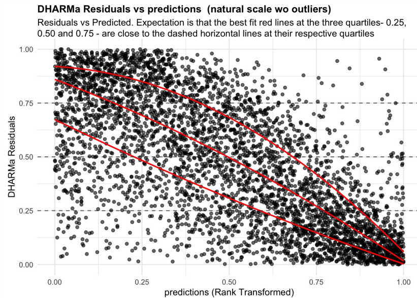
Figure 39: residuals_vs_predicted. Residuals vs Predicted Check the Residuals vs Fitted plots for good and bad examples here: https://library.virginia.edu/data/articles/diagnostic-plots
