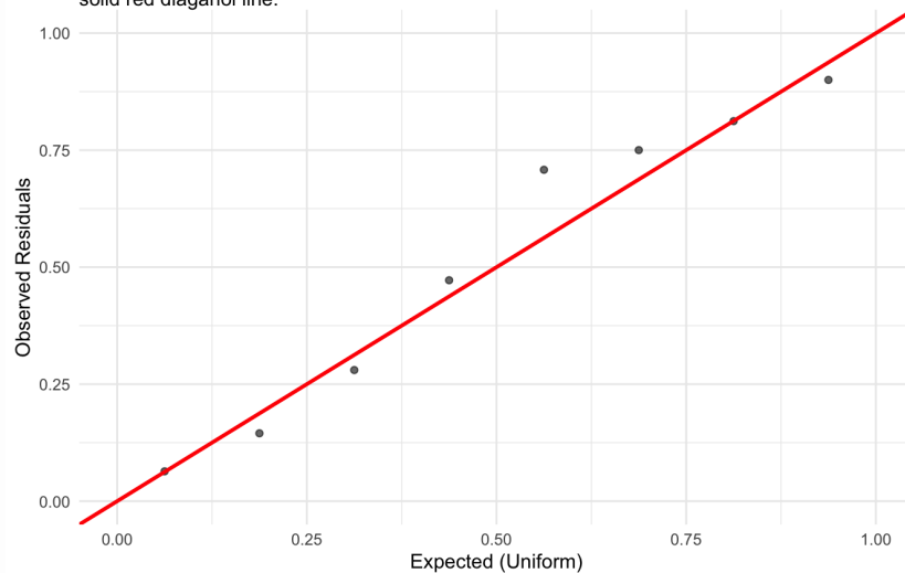
Figure 20: residuals_QQ. Q-Q Plot for Uniform Distribution. Expectation is that the black points lie on or close to the solid red diagonal line. Check the Q-Q plots for good and bad examples here: https://library.virginia.edu/data/articles/diagnostic-plots
