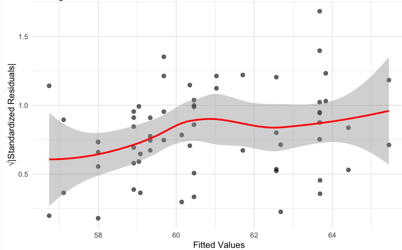
Figure 79: residuals_homoscedasticity. Check for homoscedasticity (natural scale wo outliers). Expectation is that the best fit solid red line is horizontal or close to being so. Check the Scale-Location plots for good and bad examples here: https://library.virginia.edu/data/articles/diagnostic-plots
