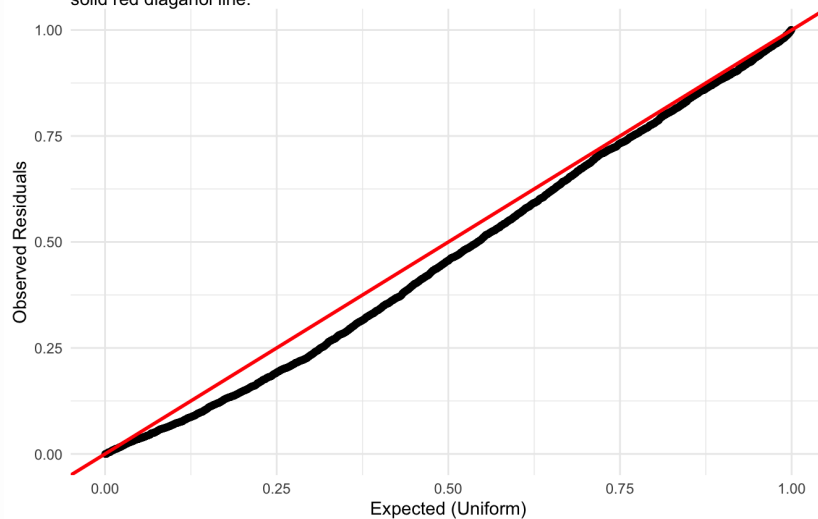
Figure 33: residuals_QQ. Q-Q Plot for Uniform Distribution. Expectation is that the black points lie on or close to the solid red diagonal line. Check the Q-Q plots for good and bad examples here: https://library.virginia.edu/data/articles/diagnostic-plots
