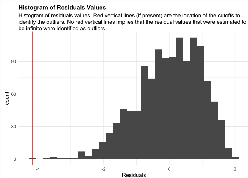
Figure 57: residuals_histogram. Histogram of residuals values. Red vertical lines (if present) are the location of the cutoffs to identify the outliers. No red vertical lines implies that the residual values that were estimated to be infinite were identified as outliers
