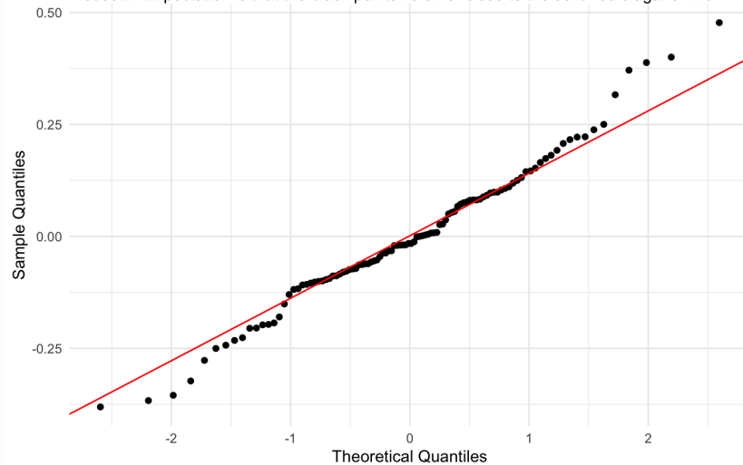
Figure 55: random_effects_QQ_1. Check normality of random effects for experimental_column2_(Intercept) (log scale): MouseID. Expectation is that the black points lie on or close to the solid red diagonal line. Check the Normal Q-Q plots for good and bad examples here: https://library.virginia.edu/data/articles/diagnostic-plots
