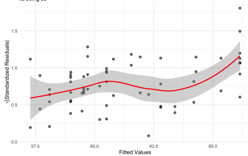
Figure 71: residuals_homoscedasticity. Check for homoscedasticity (natural scale). Expectation is that the best fit solid red line is horizontal or close to being so. Check the Scale-Location plots for good and bad examples here: https://library.virginia.edu/data/articles/diagnostic-plots
