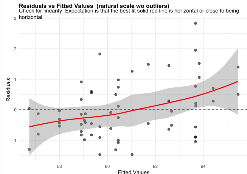
Figure 78: residuals_vs_fitted. Check for linearity (natural scale wo outliers). Expectation is that the best fit solid red line is horizontal or close to being horizontal. Check the Residuals vs Fitted plots for good and bad examples here: https://library.virginia.edu/data/articles/diagnostic-plots
