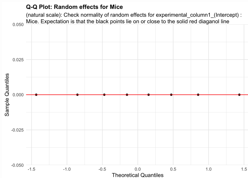
Figure 95: random_effects_QQ_2. Check normality of random effects for experimental_column1_(Intercept) (natural scale): Mice. Expectation is that the black points lie on or close to the solid red diagonal line. Check the Normal Q-Q plots for good and bad examples here: https://library.virginia.edu/data/articles/diagnostic-plots
