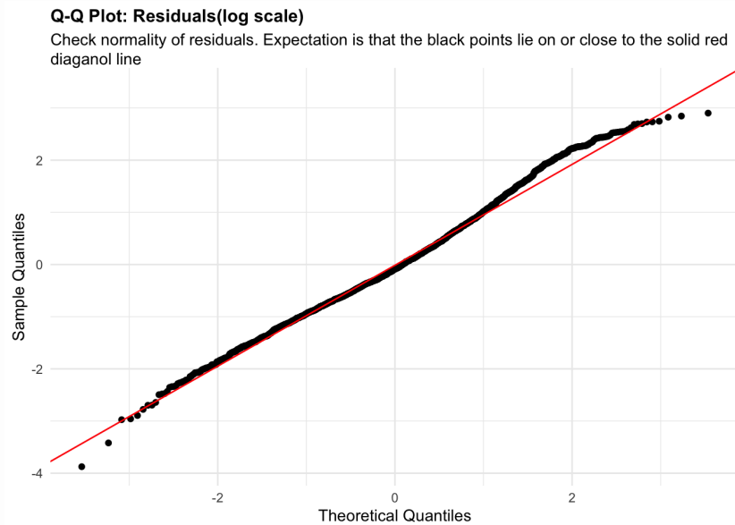
Figure 8: residuals_QQ. Check normality of residuals (log scale). Expectation is that the black points lie on or close to the solid red diagonal line. Check the Normal Q-Q plots for good and bad examples here: https://library.virginia.edu/data/articles/diagnostic-plots
