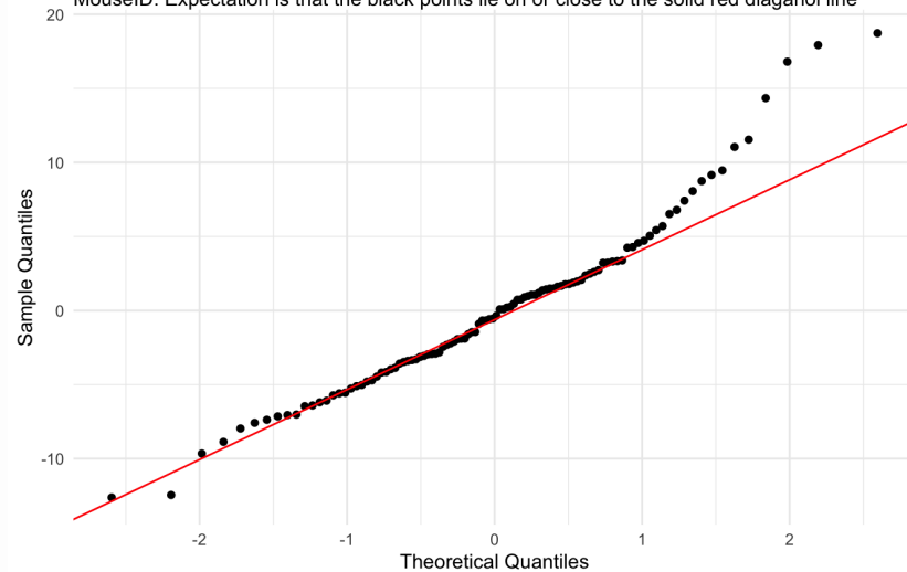
Figure 48: random_effects_QQ_1. Check normality of random effects for experimental_column2_(Intercept) (natural scale): MouseID. Expectation is that the black points lie on or close to the solid red diagonal line. Check the Normal Q-Q plots for good and bad examples here: https://library.virginia.edu/data/articles/diagnostic-plots
