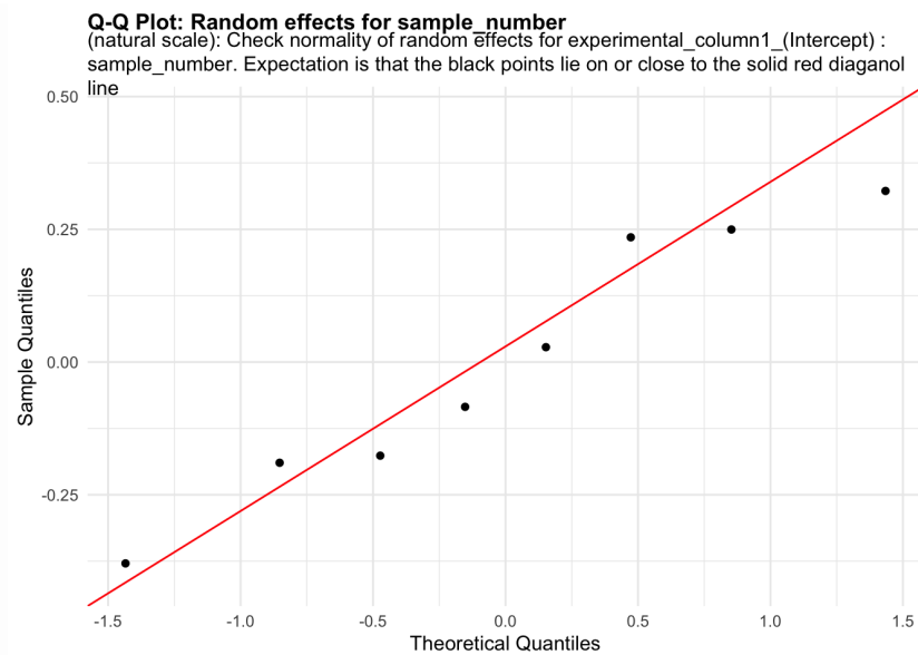
Figure 35: random_effects_QQ_1. Check normality of random effects for experimental_column1_(Intercept) (natural scale): sample_number. Expectation is that the black points lie on or close to the solid red diagonal line. Check the Normal Q-Q plots for good and bad examples here: https://library.virginia.edu/data/articles/diagnostic-plots
