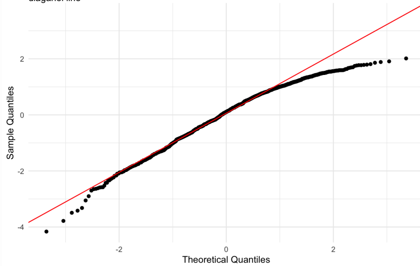
Figure 52: residuals_QQ. Check normality of residuals (log scale). Expectation is that the black points lie on or close to the solid red diagonal line. Check the Normal Q-Q plots for good and bad examples here: https://library.virginia.edu/data/articles/diagnostic-plots
