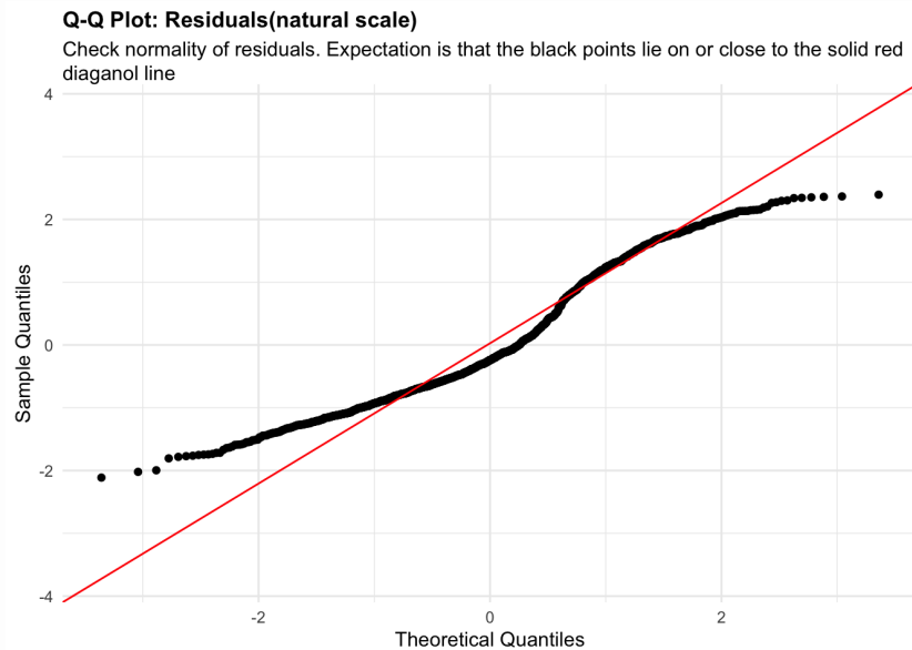
Figure 45: residuals_QQ. Check normality of residuals (natural scale). Expectation is that the black points lie on or close to the solid red diagonal line. Check the Normal Q-Q plots for good and bad examples here: https://library.virginia.edu/data/articles/diagnostic-plots
