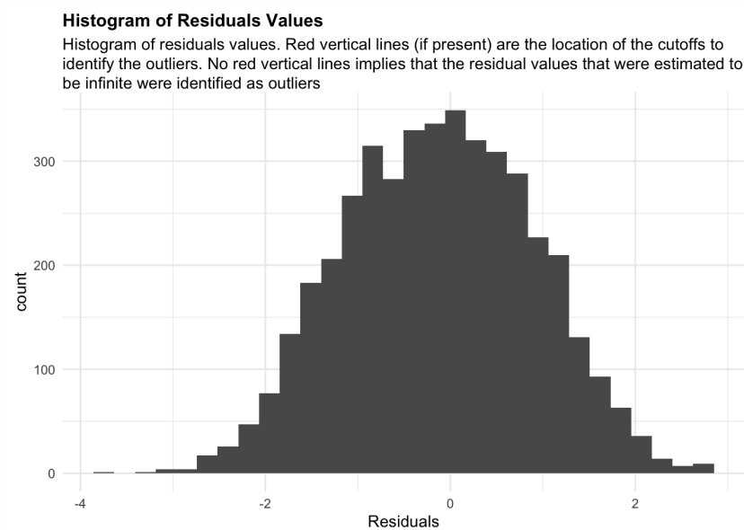
Figure 36: residuals_histogram. Histogram of residuals values. Red vertical lines (if present) are the location of the cutoffs to identify the outliers. No red vertical lines implies that the residual values that were estimated to be infinite were identified as outliers
