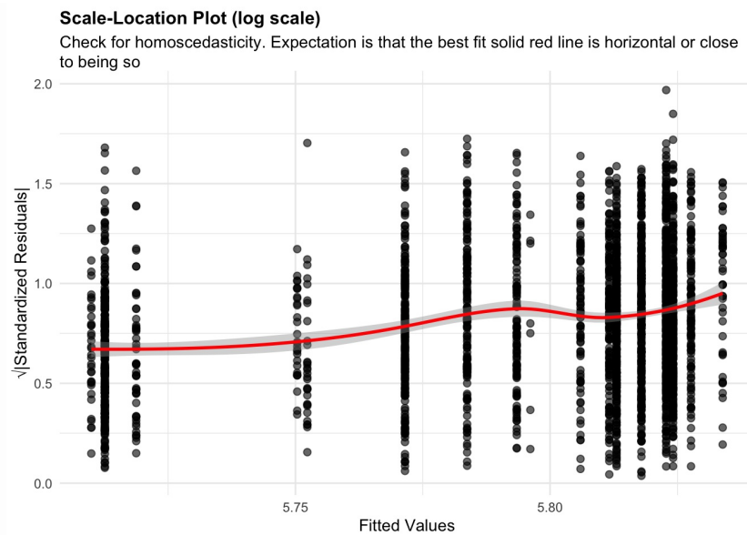
Figure 10: residuals_homoscedasticity. Check for homoscedasticity (log scale). Expectation is that the best fit solid red line is horizontal or close to being so. Check the Scale-Location plots for good and bad examples here: https://library.virginia.edu/data/articles/diagnostic-plots
