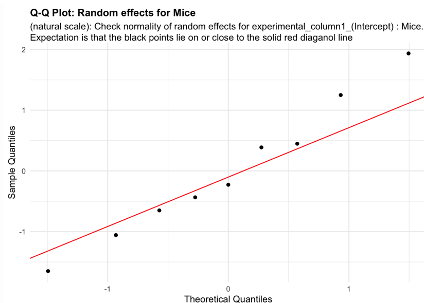
Figure 73: random_effects_QQ_2. Check normality of random effects for experimental_column1_(Intercept) (natural scale): Mice. Expectation is that the black points lie on or close to the solid red diagonal line. Check the Normal Q-Q plots for good and bad examples here: https://library.virginia.edu/data/articles/diagnostic-plots
