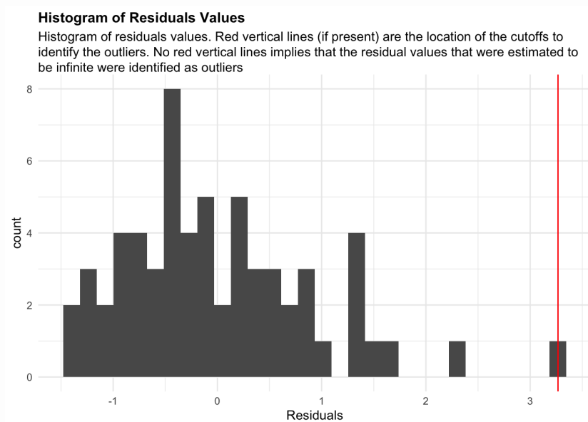
Figure 74: residuals_histogram. Histogram of residuals values. Red vertical lines (if present) are the location of the cutoffs to identify the outliers. No red vertical lines implies that the residual values that were estimated to be infinite were identified as outliers
