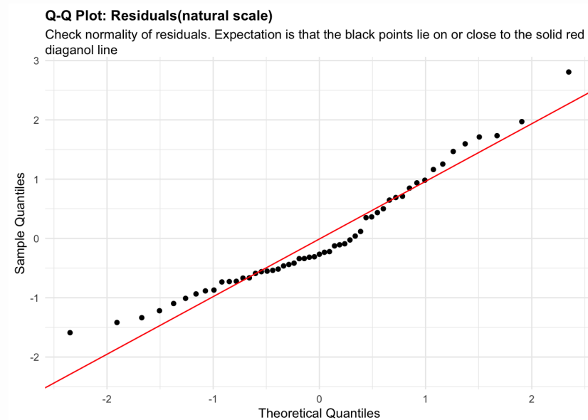
Figure 91: residuals_QQ. Check normality of residuals (natural scale). Expectation is that the black points lie on or close to the solid red diagonal line. Check the Normal Q-Q plots for good and bad examples here: https://library.virginia.edu/data/articles/diagnostic-plots
