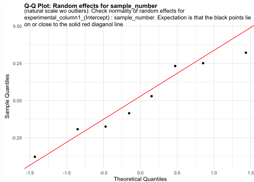
Figure 40: random_effects_QQ_1. Check normality of random effects for experimental_column1_(Intercept) (natural scale wo outliers): sample_number. Expectation is that the black points lie on or close to the solid red diagonal line. Check the Normal Q-Q plots for good and bad examples here: https://library.virginia.edu/data/articles/diagnostic-plots
