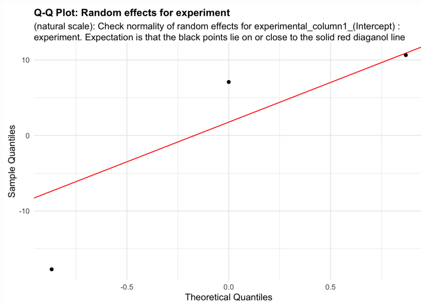
Figure 5: random_effects_QQ_2. Check normality of random effects for experimental_column1_(Intercept) (natural scale): experiment. Expectation is that the black points lie on or close to the solid red diagonal line. Check the Normal Q-Q plots for good and bad examples here: https://library.virginia.edu/data/articles/diagnostic-plots
