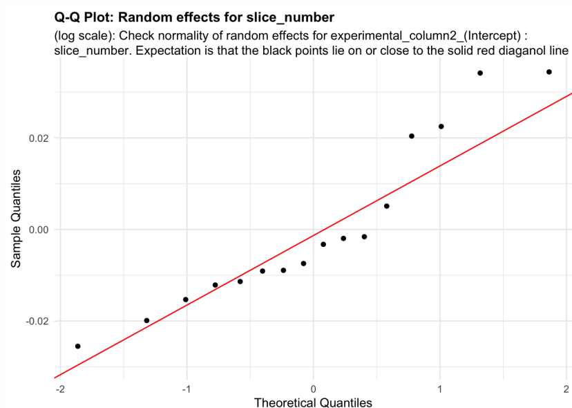
Figure 101: random_effects_QQ_1. Check normality of random effects for experimental_column2_(Intercept) (log scale): slice_number. Expectation is that the black points lie on or close to the solid red diagonal line. Check the Normal Q-Q plots for good and bad examples here: https://library.virginia.edu/data/articles/diagnostic-plots
