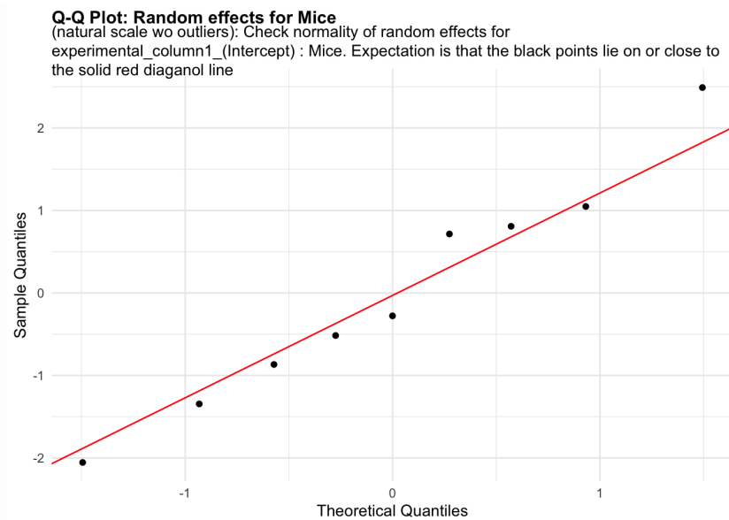
Figure 81: random_effects_QQ_2. Check normality of random effects for experimental_column1_(Intercept) (natural scale wo outliers): Mice. Expectation is that the black points lie on or close to the solid red diagonal line. Check the Normal Q-Q plots for good and bad examples here: https://library.virginia.edu/data/articles/diagnostic-plots
