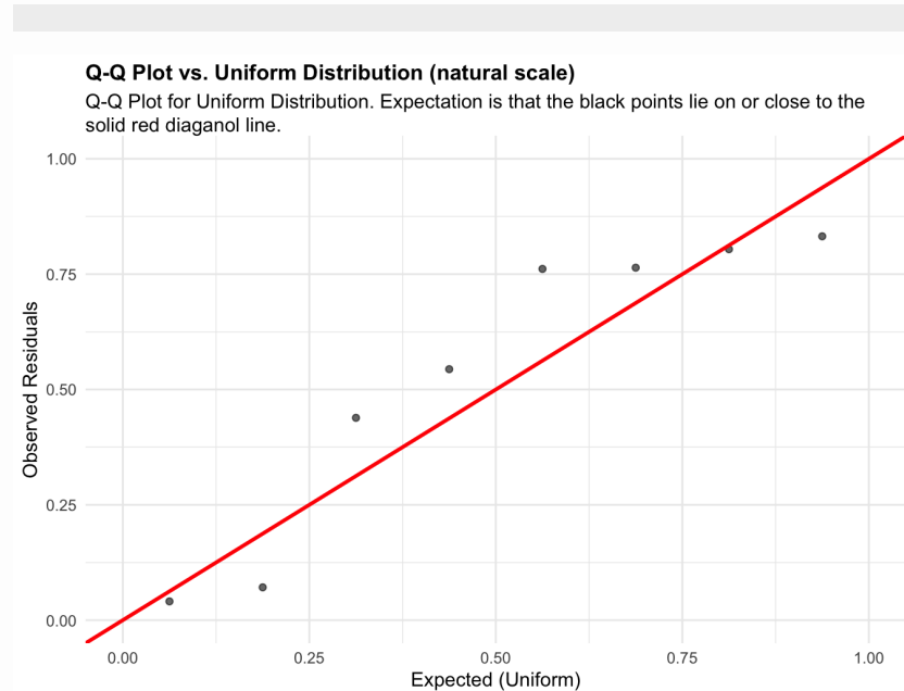
Figure 27: residuals_QQ. Q-Q Plot for Uniform Distribution. Expectation is that the black points lie on or close to the solid red diagonal line. Check the Q-Q plots for good and bad examples here: https://library.virginia.edu/data/articles/diagnostic-plots
