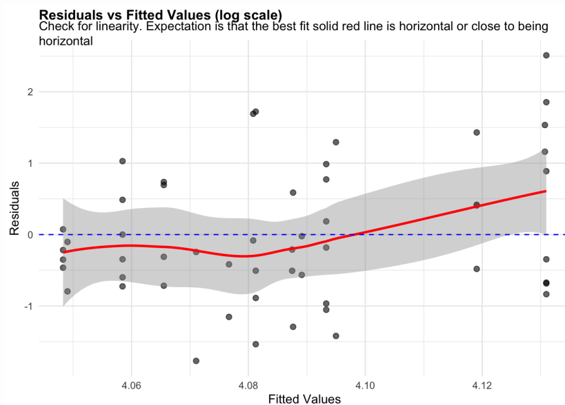
Figure 99: residuals_vs_fitted. Check for linearity (log scale). Expectation is that the best fit solid red line is horizontal or close to being horizontal. Check the Residuals vs Fitted plots for good and bad examples here: https://library.virginia.edu/data/articles/diagnostic-plots
