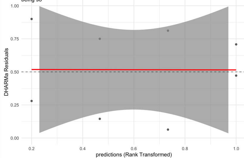
Figure 21: residuals_vs_predicted. Residuals vs Predicted Check the Residuals vs Fitted plots for good and bad examples here: https://library.virginia.edu/data/articles/diagnostic-plots
