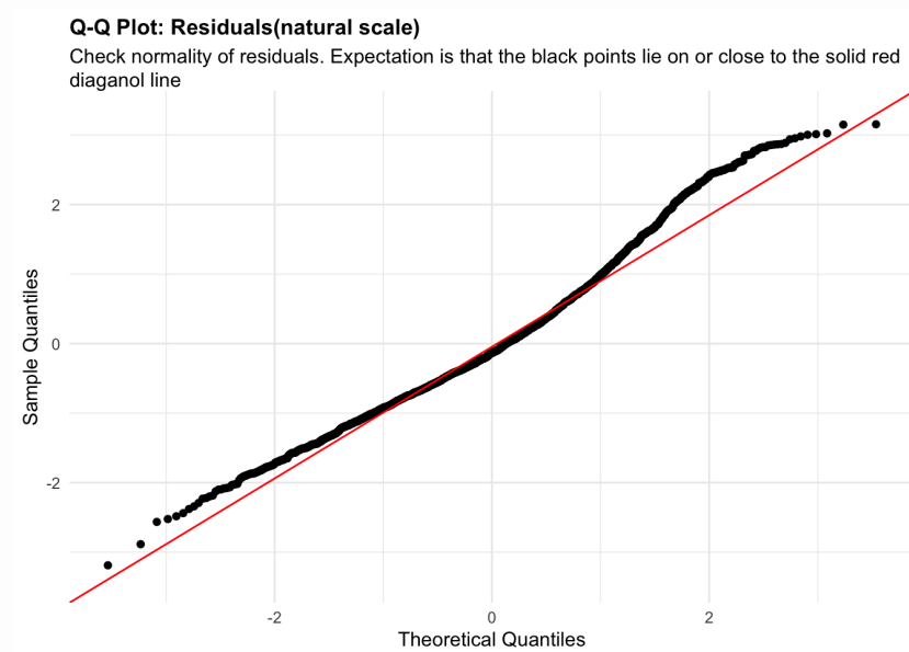
Figure 1: residuals_QQ. Check normality of residuals (natural scale). Expectation is that the black points lie on or close to the solid red diagonal line. Check the Normal Q-Q plots for good and bad examples here: https://library.virginia.edu/data/articles/diagnostic-plots
