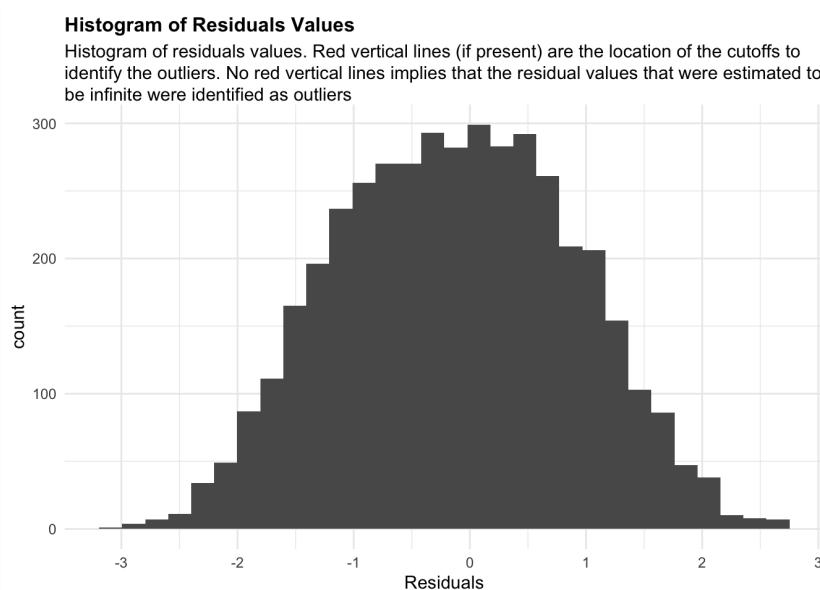
Figure 41: residuals_histogram. Histogram of residuals values. Red vertical lines (if present) are the location of the cutoffs to identify the outliers. No red vertical lines implies that the residual values that were estimated to be infinite were identified as outliers
