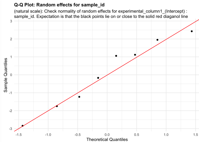
Figure 22: random_effects_QQ_1. Check normality of random effects for experimental_column1_(Intercept) (natural scale): sample_id. Expectation is that the black points lie on or close to the solid red diagonal line. Check the Normal Q-Q plots for good and bad examples here: https://library.virginia.edu/data/articles/diagnostic-plots
