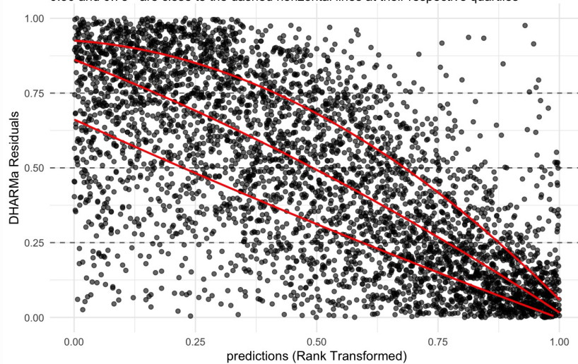
Figure 34: residuals_vs_predicted. Residuals vs Predicted Check the Residuals vs Fitted plots for good and bad examples here: https://library.virginia.edu/data/articles/diagnostic-plots
