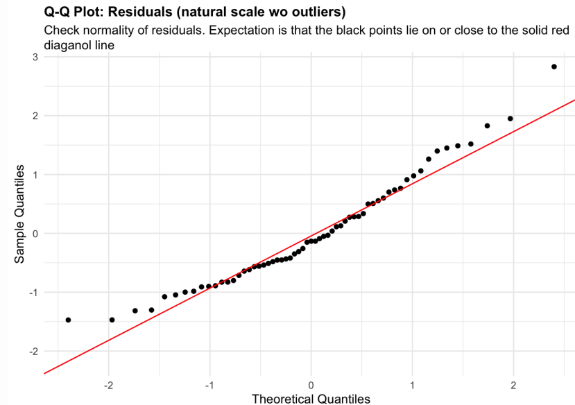
Figure 77: residuals_QQ. Check normality of residuals (natural scale wo outliers). Expectation is that the black points lie on or close to the solid red diagonal line. Check the Normal Q-Q plots for good and bad examples here: https://library.virginia.edu/data/articles/diagnostic-plots
