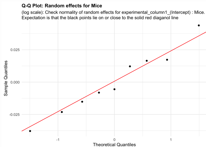
Figure 88: random_effects_QQ_2. Check normality of random effects for experimental_column1_(Intercept) (log scale): Mice. Expectation is that the black points lie on or close to the solid red diagonal line. Check the Normal Q-Q plots for good and bad examples here: https://library.virginia.edu/data/articles/diagnostic-plots
