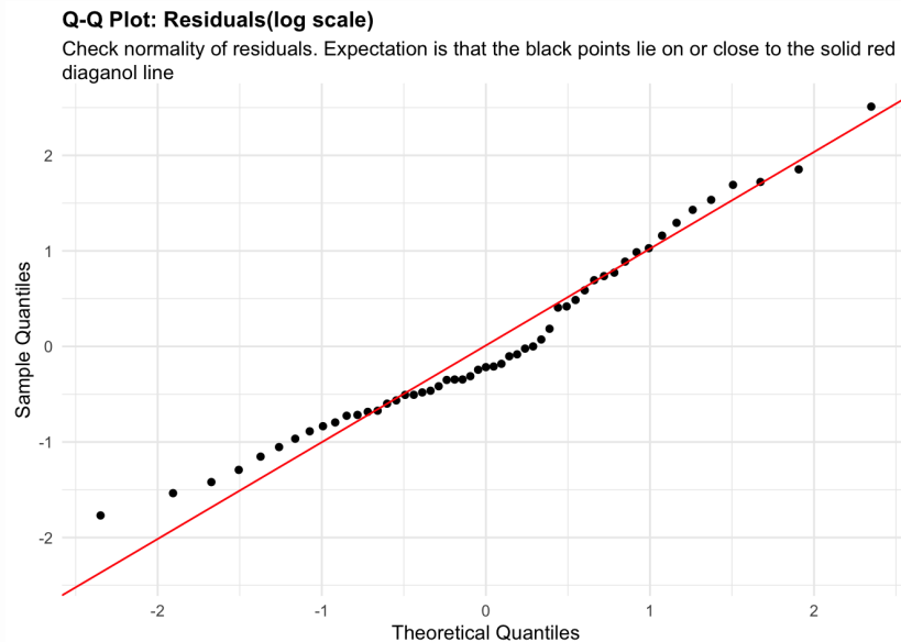
Figure 98: residuals_QQ. Check normality of residuals (log scale). Expectation is that the black points lie on or close to the solid red diagonal line. Check the Normal Q-Q plots for good and bad examples here: https://library.virginia.edu/data/articles/diagnostic-plots
