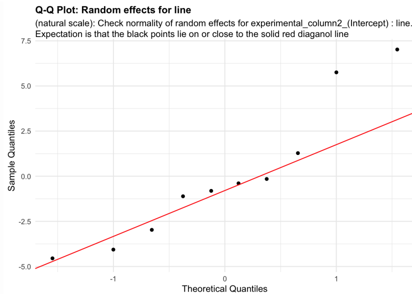
Figure 4: random_effects_QQ_1. Check normality of random effects for experimental_column2_(Intercept) (natural scale): line. Expectation is that the black points lie on or close to the solid red diagonal line. Check the Normal Q-Q plots for good and bad examples here: https://library.virginia.edu/data/articles/diagnostic-plots
