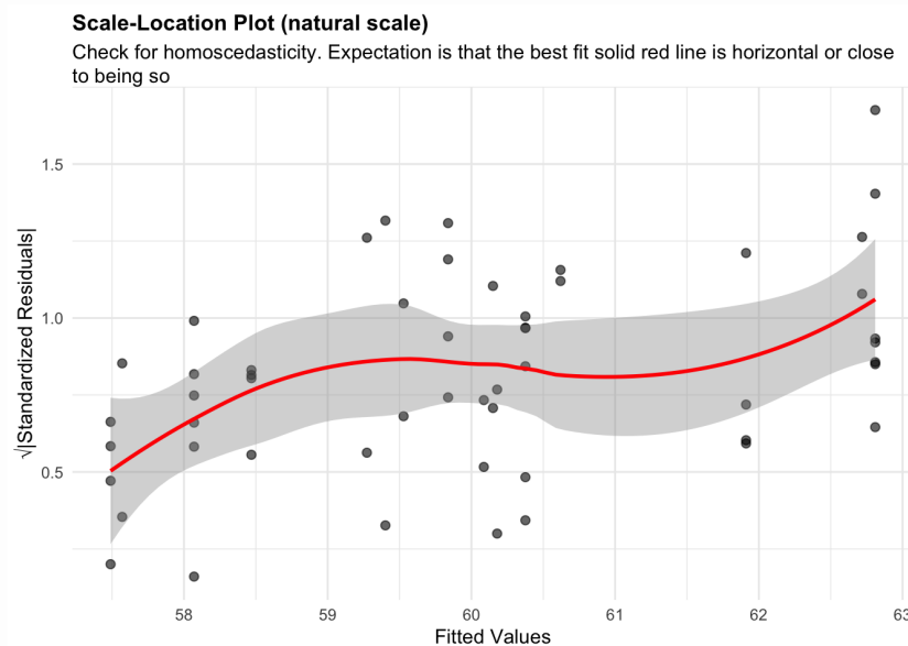
Figure 93: residuals_homoscedasticity. Check for homoscedasticity (natural scale). Expectation is that the best fit solid red line is horizontal or close to being so. Check the Scale-Location plots for good and bad examples here: https://library.virginia.edu/data/articles/diagnostic-plots
