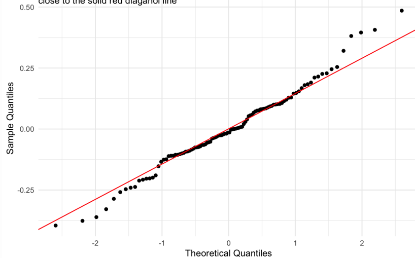
Figure 63: random_effects_QQ_1. Check normality of random effects for experimental_column2_(Intercept) (log scale wo outlier): MouseID. Expectation is that the black points lie on or close to the solid red diagonal line. Check the Normal Q-Q plots for good and bad examples here: https://library.virginia.edu/data/articles/diagnostic-plots
