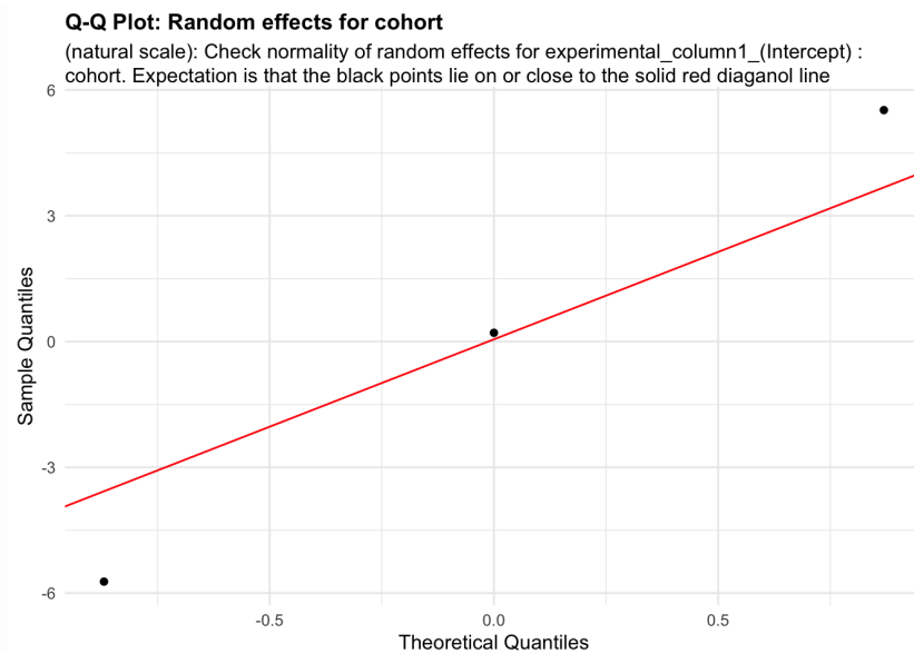
Figure 49: random_effects_QQ_2. Check normality of random effects for experimental_column1_(Intercept) (natural scale): cohort. Expectation is that the black points lie on or close to the solid red diagonal line. Check the Normal Q-Q plots for good and bad examples here: https://library.virginia.edu/data/articles/diagnostic-plots
