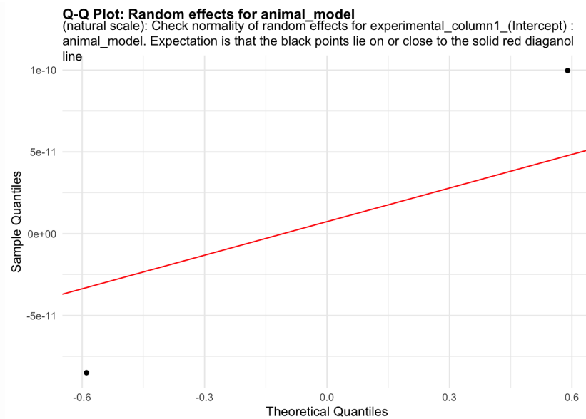
Figure 30: random_effects_QQ_2. Check normality of random effects for experimental_column1_(Intercept) (natural scale): animal_model. Expectation is that the black points lie on or close to the solid red diagonal line. Check the Normal Q-Q plots for good and bad examples here: https://library.virginia.edu/data/articles/diagnostic-plots
