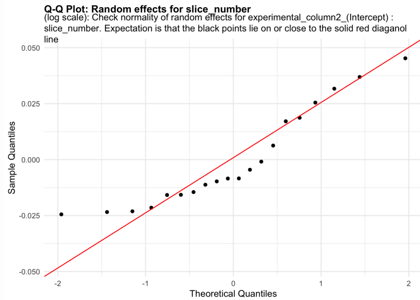
Figure 87: random_effects_QQ_1. Check normality of random effects for experimental_column2_(Intercept) (log scale): slice_number. Expectation is that the black points lie on or close to the solid red diagonal line. Check the Normal Q-Q plots for good and bad examples here: https://library.virginia.edu/data/articles/diagnostic-plots
