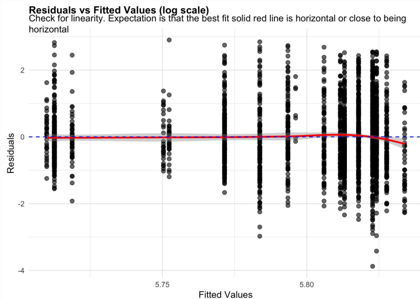
Figure 9: residuals_vs_fitted. Check for linearity (log scale). Expectation is that the best fit solid red line is horizontal or close to being horizontal. Check the Residuals vs Fitted plots for good and bad examples here: https://library.virginia.edu/data/articles/diagnostic-plots
