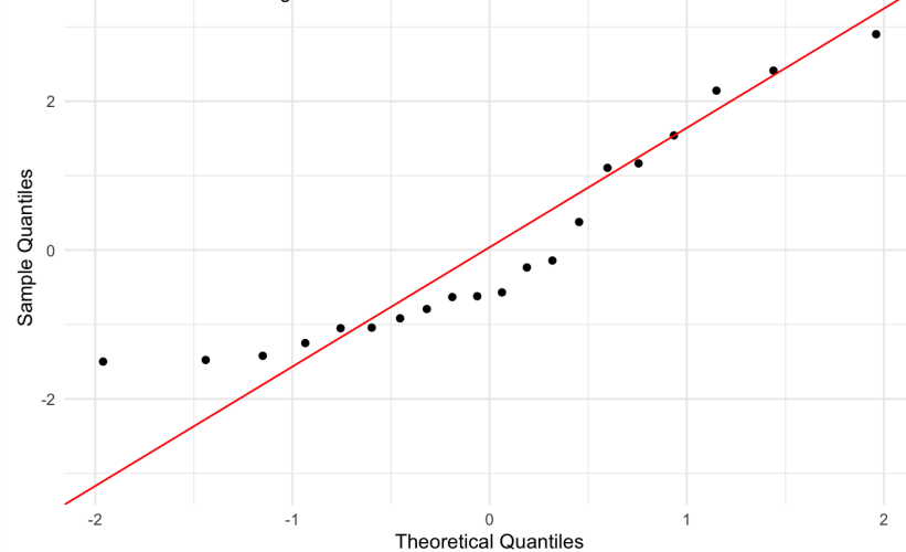
Figure 80: random_effects_QQ_1. Check normality of random effects for experimental_column2_(Intercept) (natural scale wo outliers): slice_number. Expectation is that the black points lie on or close to the solid red diagonal line. Check the Normal Q-Q plots for good and bad examples here: https://library.virginia.edu/data/articles/diagnostic-plots
