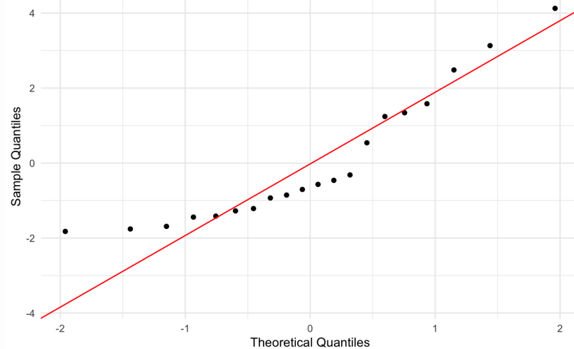
Figure 72: random_effects_QQ_1. Check normality of random effects for experimental_column2_(Intercept) (natural scale): slice_number. Expectation is that the black points lie on or close to the solid red diagonal line. Check the Normal Q-Q plots for good and bad examples here: https://library.virginia.edu/data/articles/diagnostic-plots
