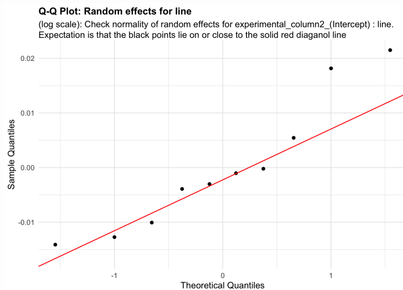
Figure 11: random_effects_QQ_1. Check normality of random effects for experimental_column2_(Intercept) (log scale): line. Expectation is that the black points lie on or close to the solid red diagonal line. Check the Normal Q-Q plots for good and bad examples here: https://library.virginia.edu/data/articles/diagnostic-plots
