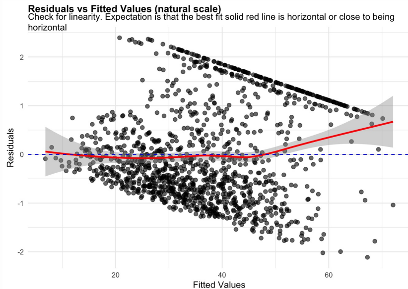
Figure 46: residuals_vs_fitted. Check for linearity (natural scale). Expectation is that the best fit solid red line is horizontal or close to being horizontal. Check the Residuals vs Fitted plots for good and bad examples here: https://library.virginia.edu/data/articles/diagnostic-plots
