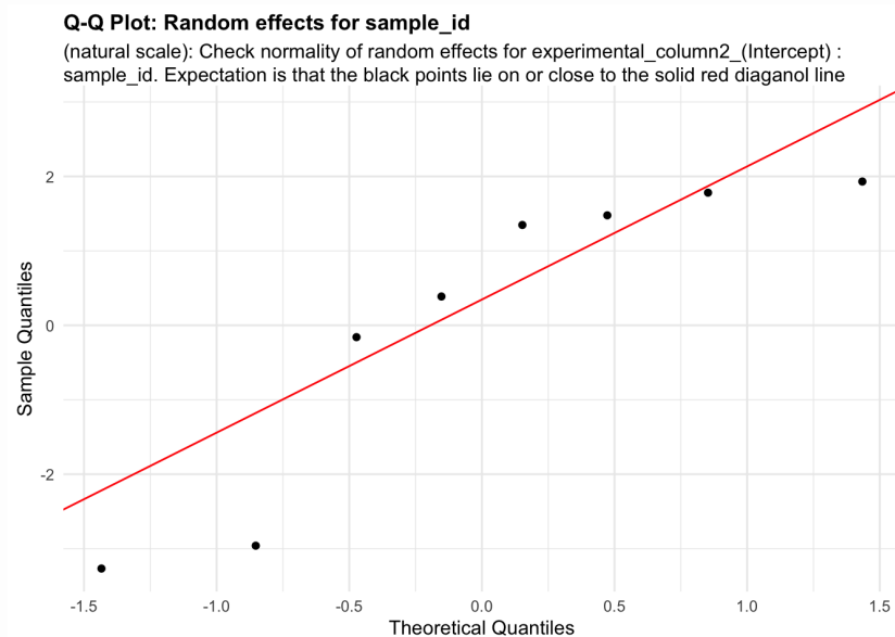
Figure 29: random_effects_QQ_1. Check normality of random effects for experimental_column2_(Intercept) (natural scale): sample_id. Expectation is that the black points lie on or close to the solid red diagonal line. Check the Normal Q-Q plots for good and bad examples here: https://library.virginia.edu/data/articles/diagnostic-plots
