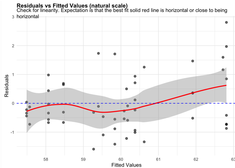
Figure 92: residuals_vs_fitted. Check for linearity (natural scale). Expectation is that the best fit solid red line is horizontal or close to being horizontal. Check the Residuals vs Fitted plots for good and bad examples here: https://library.virginia.edu/data/articles/diagnostic-plots
