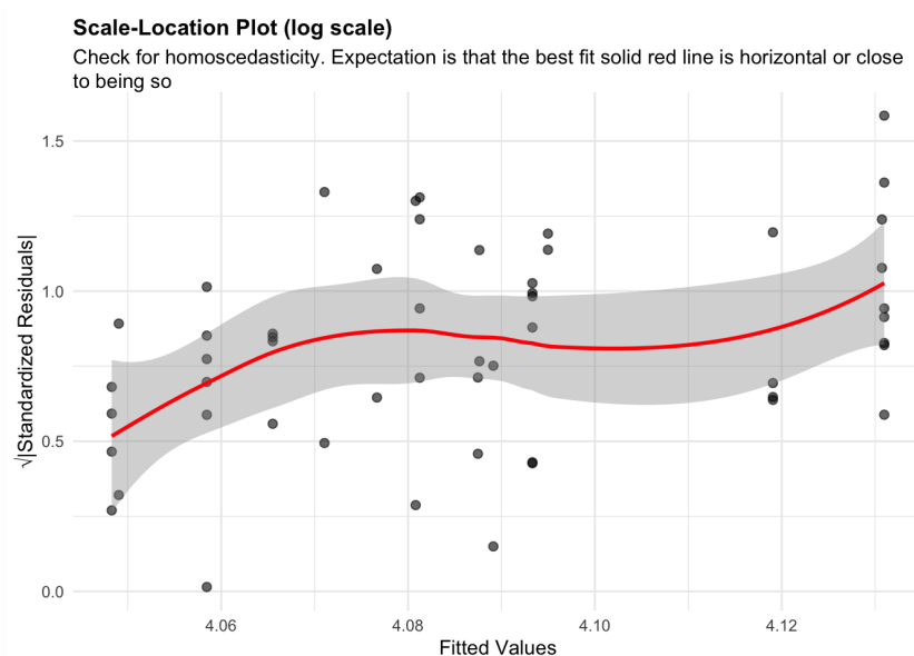
Figure 100: residuals_homoscedasticity. Check for homoscedasticity (log scale). Expectation is that the best fit solid red line is horizontal or close to being so. Check the Scale-Location plots for good and bad examples here: https://library.virginia.edu/data/articles/diagnostic-plots
