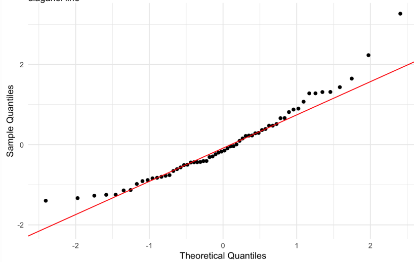
Figure 69: residuals_QQ. Check normality of residuals (natural scale). Expectation is that the black points lie on or close to the solid red diagonal line. Check the Normal Q-Q plots for good and bad examples here: https://library.virginia.edu/data/articles/diagnostic-plots
