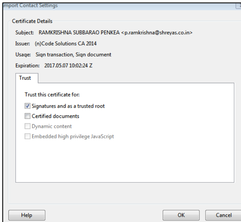
Figure 4: Import Contact Settings
