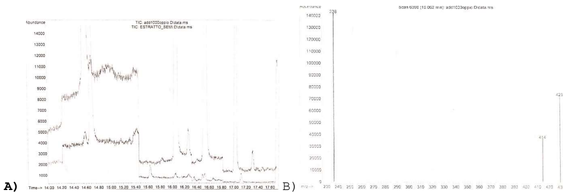
Figure 4 - A) Chromatogram of the qualitative analysis on poppy seeds; B) Ion rates (m/z) of morphine (429, 414, 236) present in poppy seeds sample.
