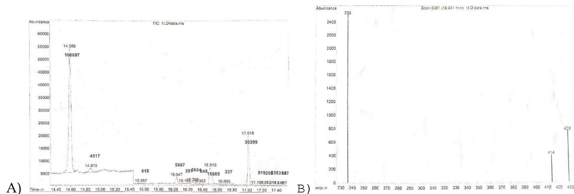
Figure 3 - A) Chromatogram of the analysed urine sample of subject 1; B) Ion rates (m/z) of morphine (429, 414, 236) present in the analysed urine sample of subject 1.
