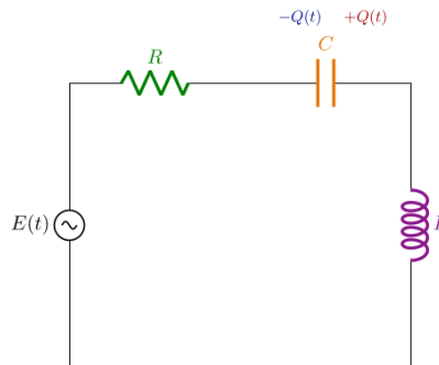
Figure 3.22: A simple RLC series electric circuit.
