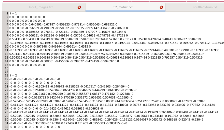
Figure 10.54: The S2 feature maps after performing average pooling on C1 layer.
