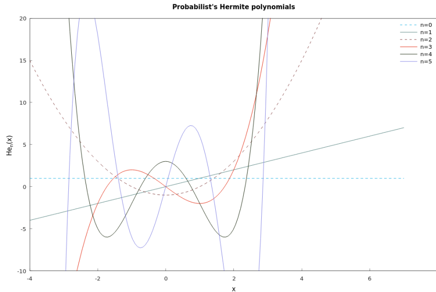
Figure 3.75: The probabilist's Hermite polynomials (Hamzstplot/Examples with Makefile/Differential Equation-s/Plot 2D Probabilist's Hermite Polynomials/main.cpp).
