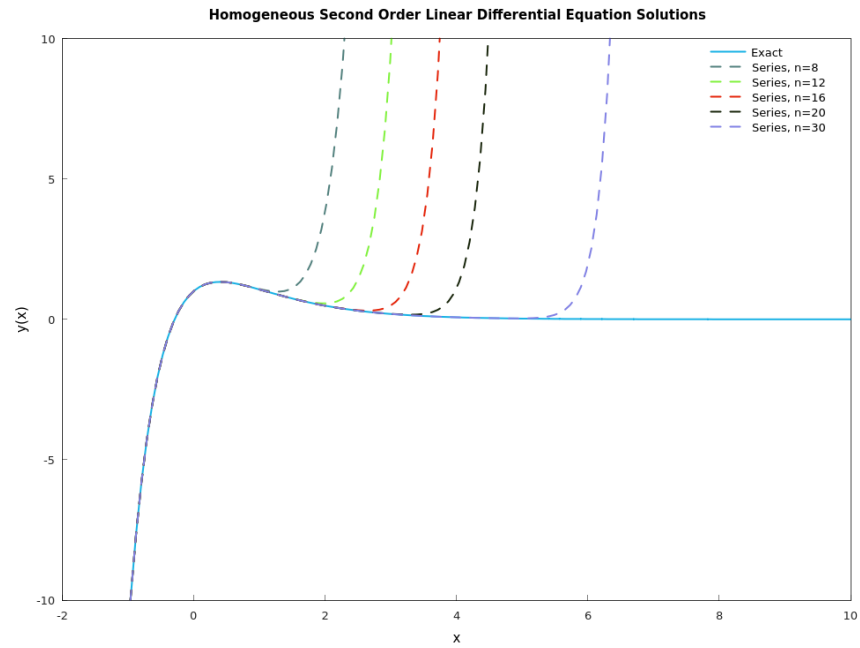
Figure 3.69: The plot of the exact solution and the series solution with various terms for the differential equation y'' + 3y' + 2y = 0 , we combine SymIntegration library with Hamzstplot, thus SymIntegration is used to compute the series solution and then plot it with Hamzstplot ( Hamzstplot/Examples with Makefile/Differential Equations/Plot 2D Comparing Series Solutions with Exact Solution for Second Order Homogeneous Linear Differential Equation/main.cpp ).
